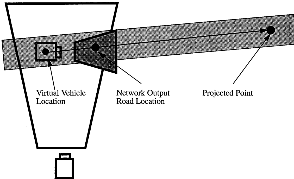
Figure 11: Network Output Based Point Projection Diagram.
