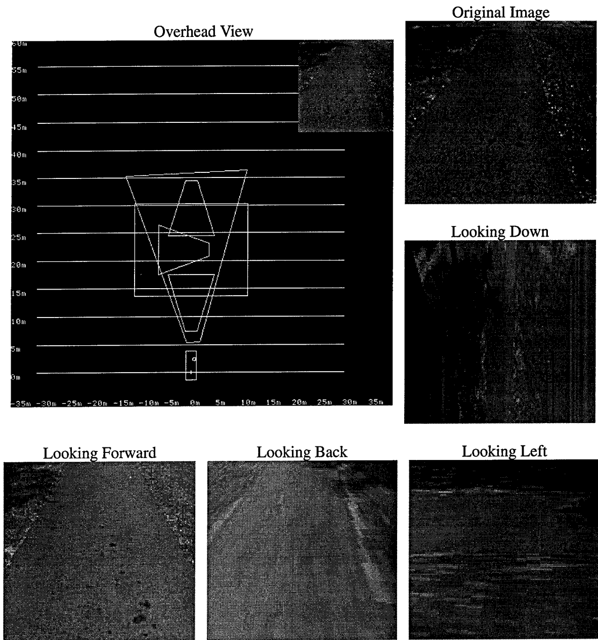
Figure 2: Typical virtual camera scenes.
