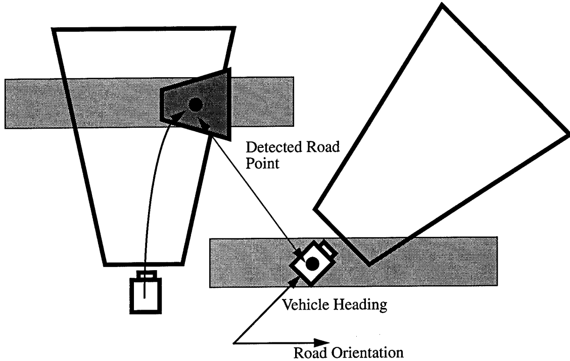
Figure 9: Vehicle/Road Misalignment.
