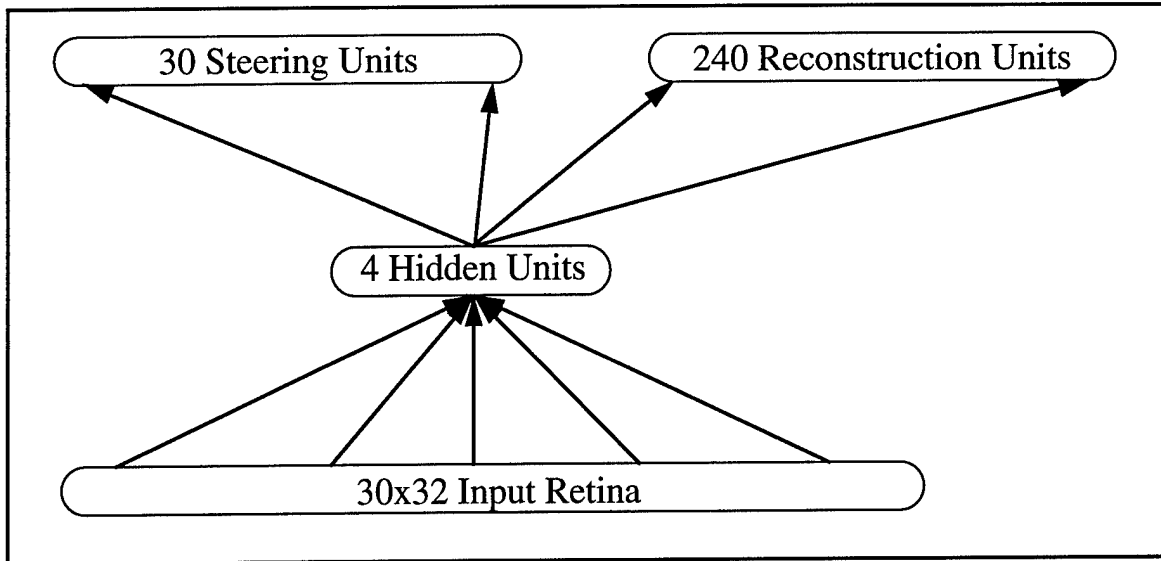
Figure 1: ALVINN network architecture.
