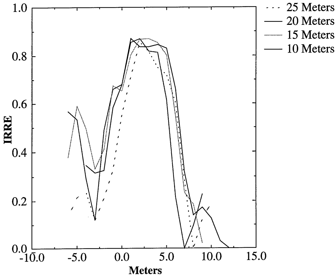
Figure 8: IRRE response as a function of virtual camera distance from the center of the road. Negative number are closer to the road and positive number are further away.
