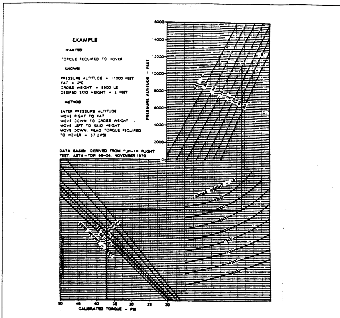
Figure 1, UH-1H Hover Performance Chart
