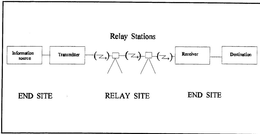
Figure 17: Microwave Relay Block Diagram
