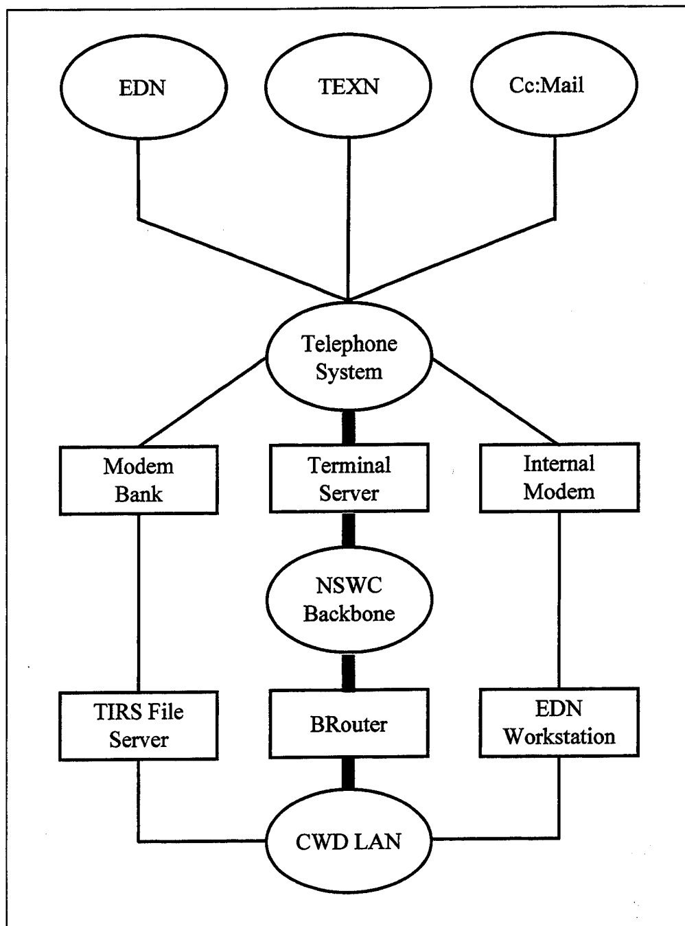
Figure 28. Dial-Up Networks
