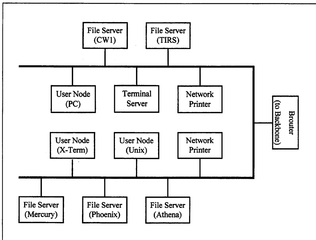
Figure 24. Local Area Network (Logical View)
