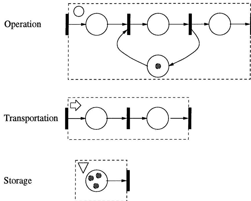
Figure 3.13: Petri nets for nodes
