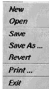
Figure 4.4: File menu
