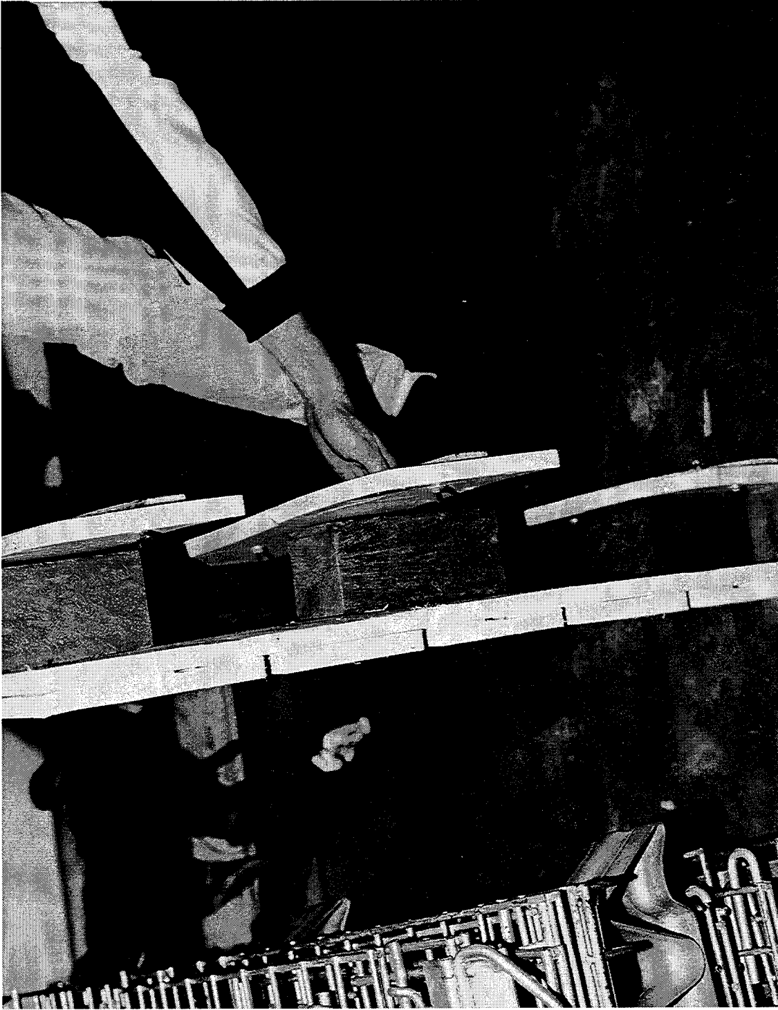
U.S. ARMY DEFENSE AMMUNITION CENTER AND SCHOOL - SAVANNA, IL AO317-SCN95-126-1348. This photo shows the skid detached from the post. The screws attaching the skid sheared off.
