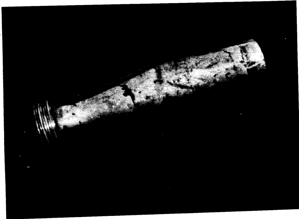
Figure 9. Standard Hamm Style Shotcrete Nozzle.
