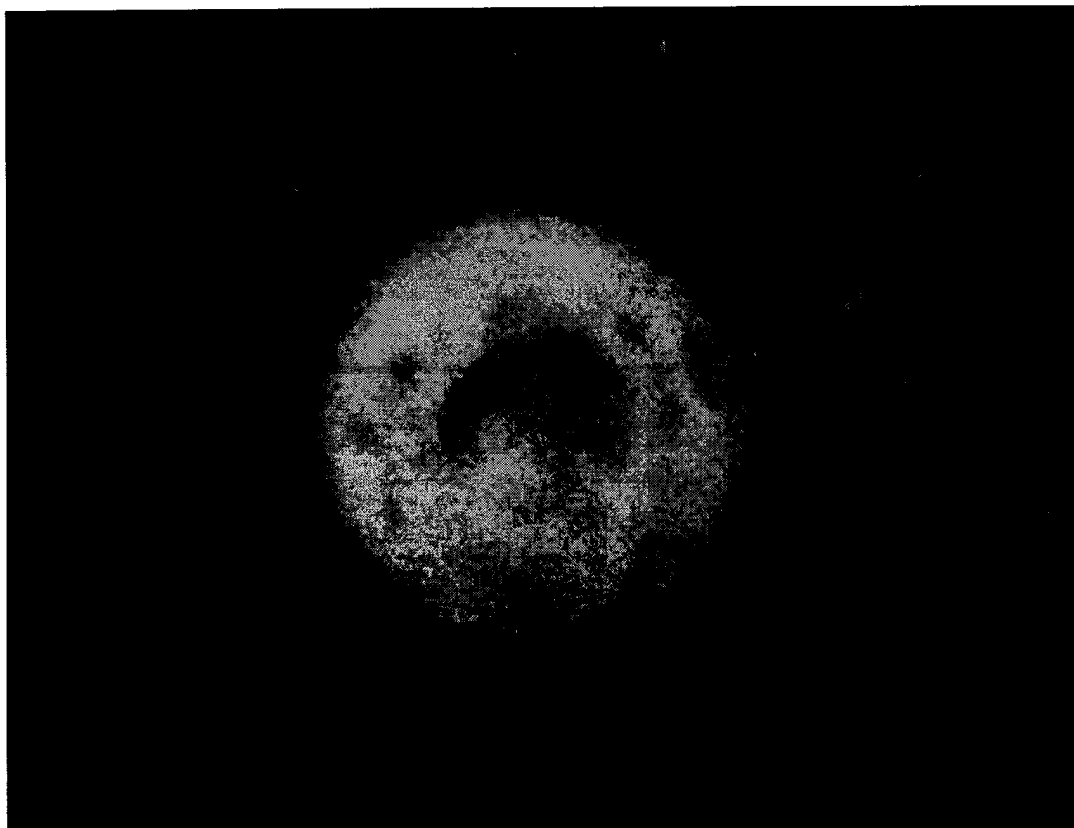
Figure 7.9: Anomalous lesion ( 900\ \mu\text{m} diameter) formed in an albumen eye phantom. Bubbles at the center of the lesion result in a lower reflectance and hence an overall annular reflectance pattern. Gaussian beam profile, \lambda = 488 and 514\ \text{nm} , 750\ \mu\text{m} spot, irradiation time of 0.5\ \text{s} at 195\ \text{mW} .
