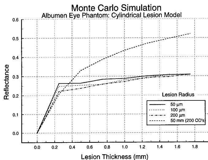
Figure 7.7: Monte Carlo simulation of buried cylindrical lesion in an albumen eye phantom. Gaussian laser beam (power is normalized) having a diameter of 750 \mu\text{m} and \lambda = 488 \text{ nm} and 514 nm; 5000 photons simulated.
