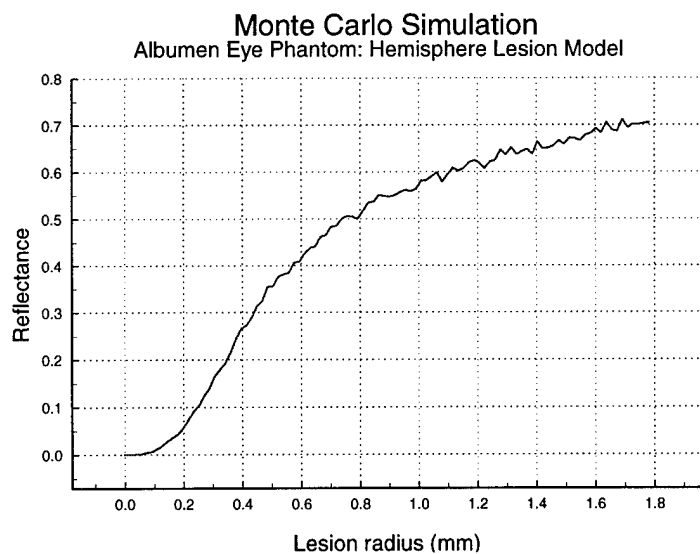
Figure 7.8: Monte Carlo simulation of buried hemispherical lesion in an albumen eye phantom. Gaussian laser beam (power is normalized) having a diameter of 750 \mu\text{m} and \lambda = 488 \text{ nm} and 514 nm; 5000 photons simulated.
