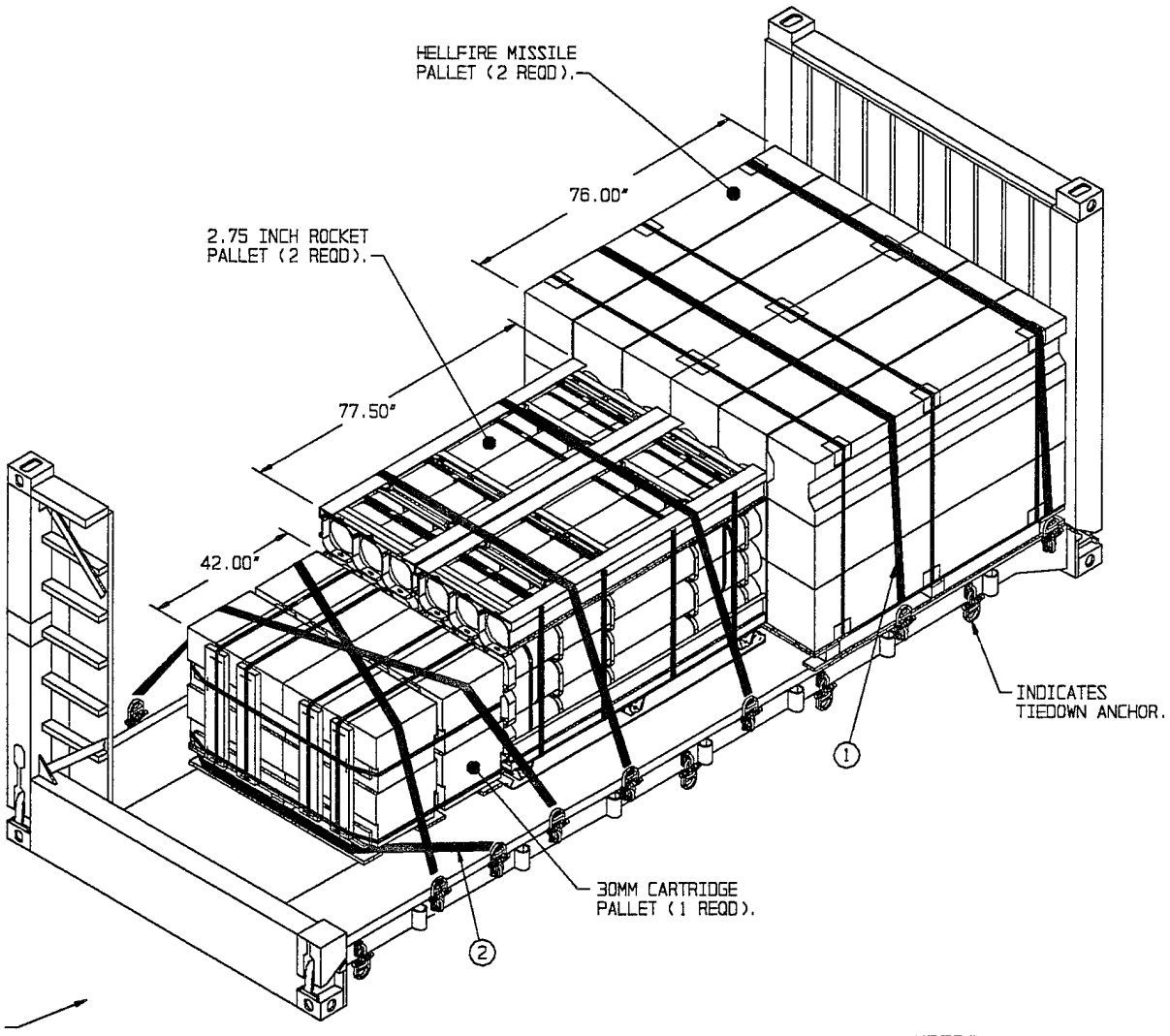
ISOMETRIC VIEW
