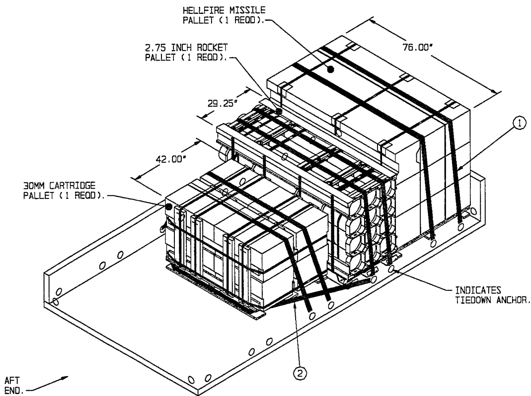
ISOMETRIC VIEW
