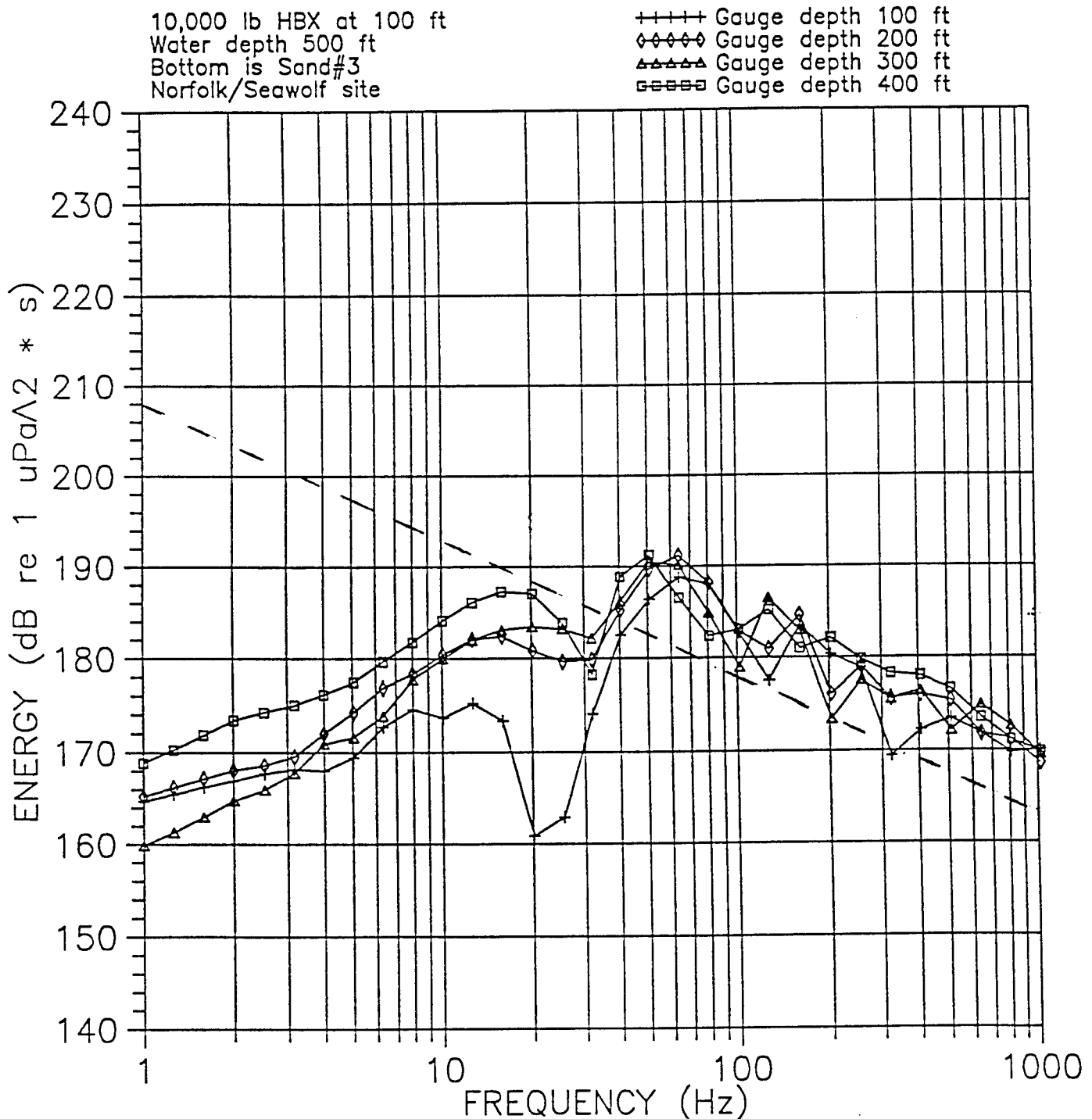
FIGURE D-1. 1/3-OCTAVE-BAND ENERGY VS FREQUENCY - NORFOLK AREA: APRIL; RANGE = 4 NM; MAMMAL DEPTH = 100 TO 400 FT
