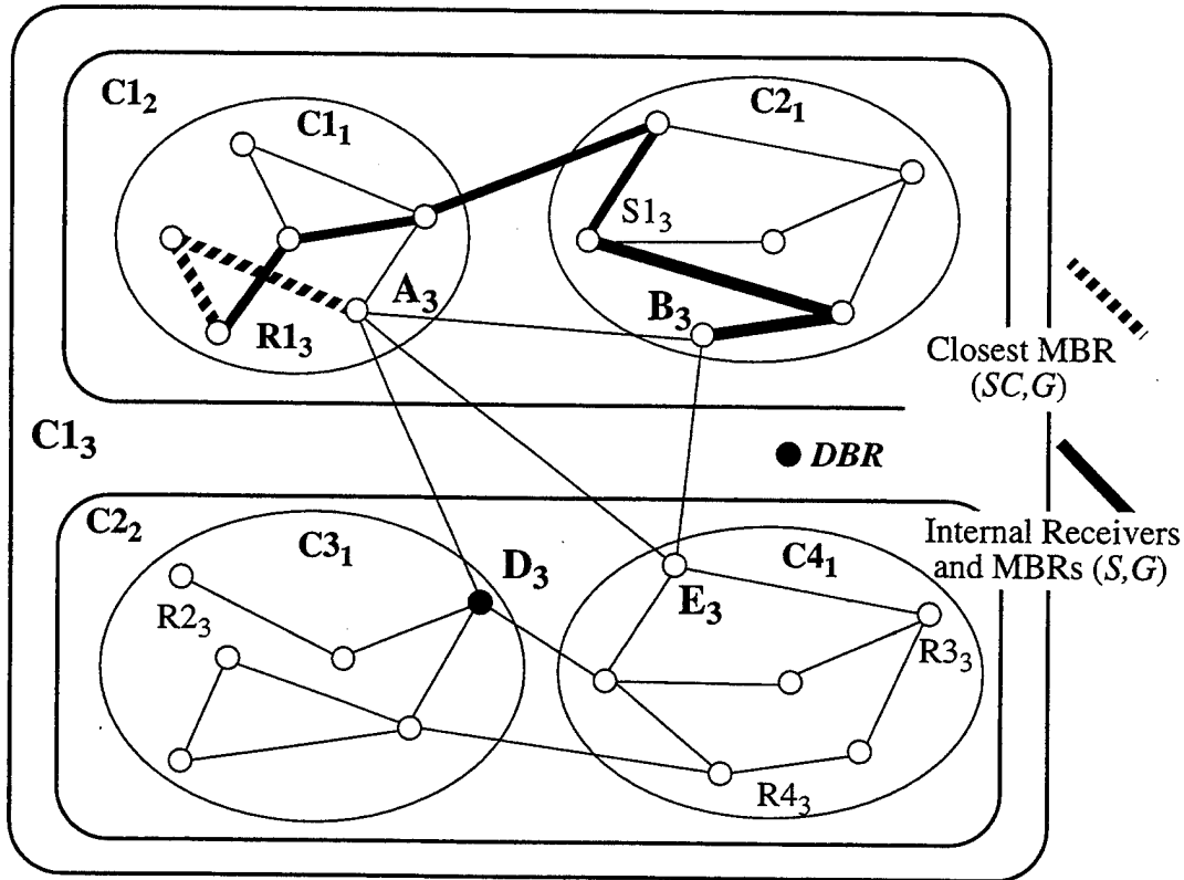
Figure 3.16: Receiver R1 3 Joins the Sender and Closest MBR
