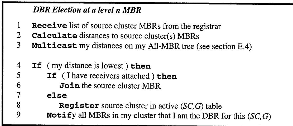
Figure 3.9: Algorithm for DBR Election
