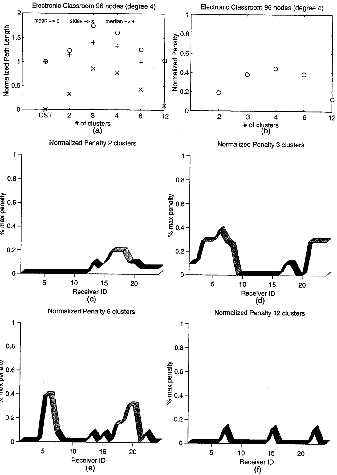
Figure 7.2 Electronic Classroom 96 Node Case Node Degree 4
