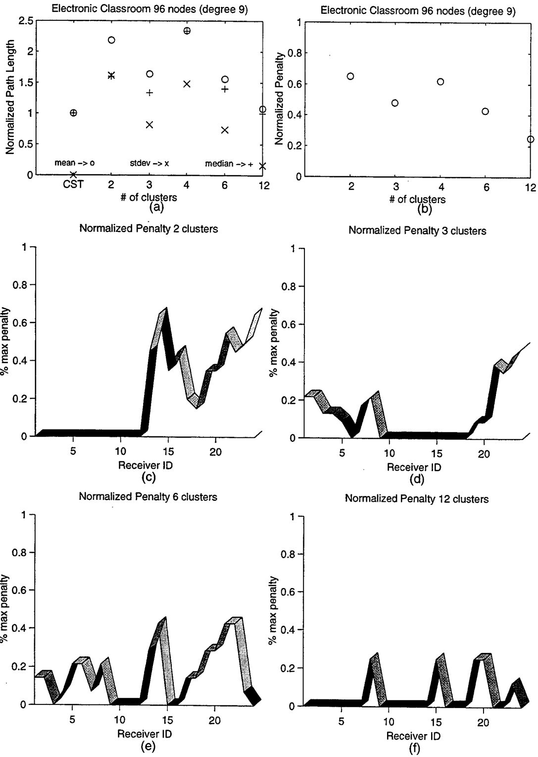
Figure 7.3 Electronic Classroom 96 Node Case Node Degree 9
