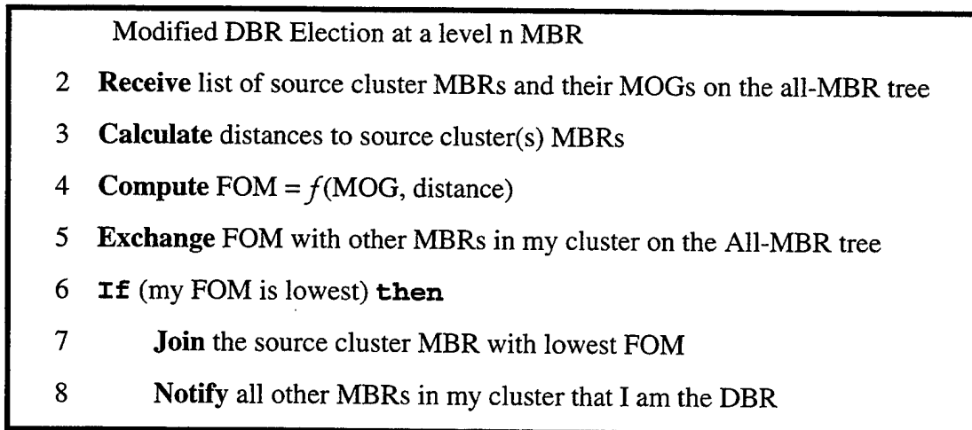
Figure 5.1: Algorithm for DBR Election using MOG
