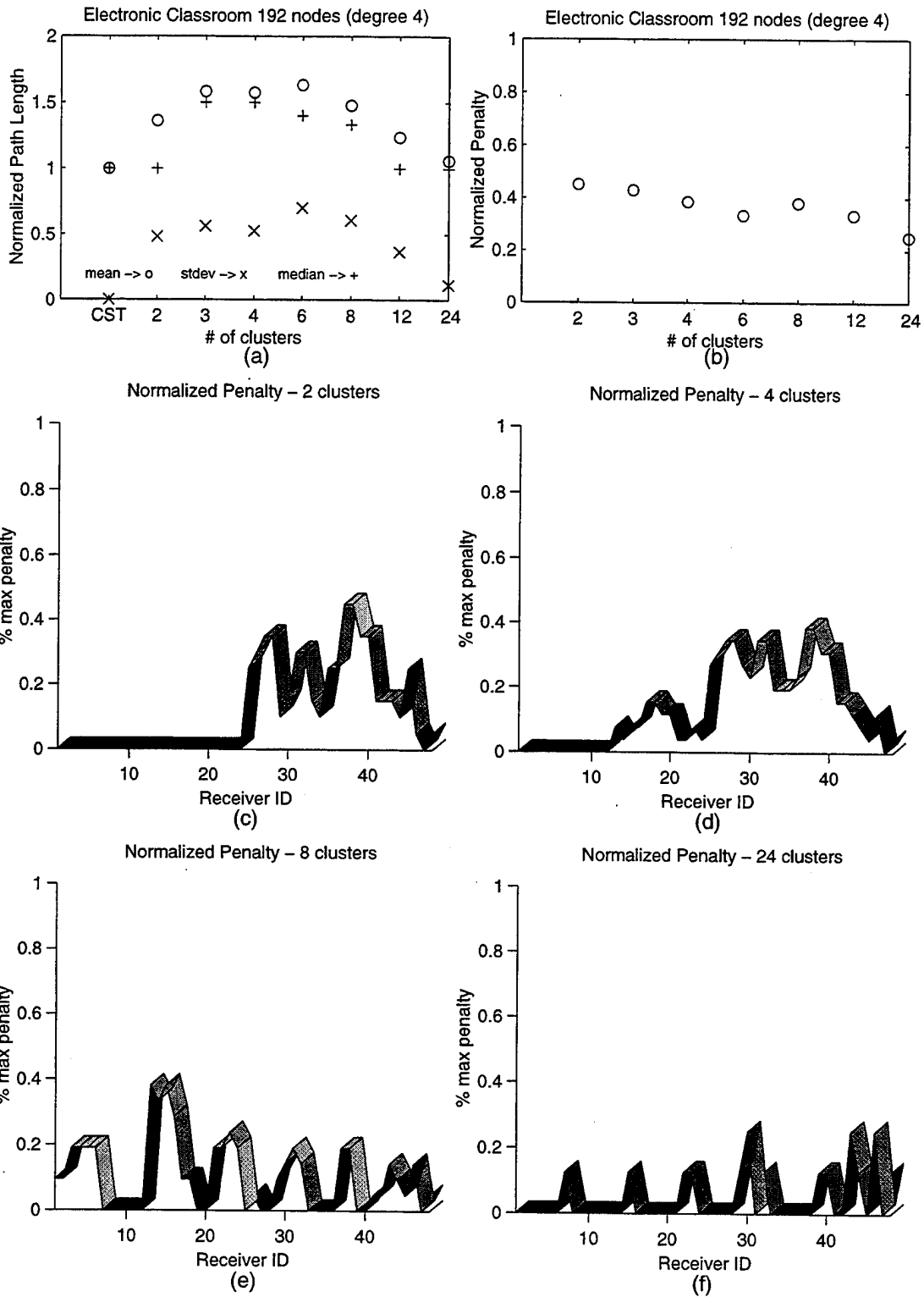
Figure 7.6 Electronic Classroom 192 Node Case Node Degree 4
