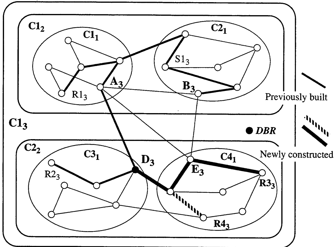
Figure 3.18: Receivers R_{3_3} and R_{4_3} Join their Closest MBRs
