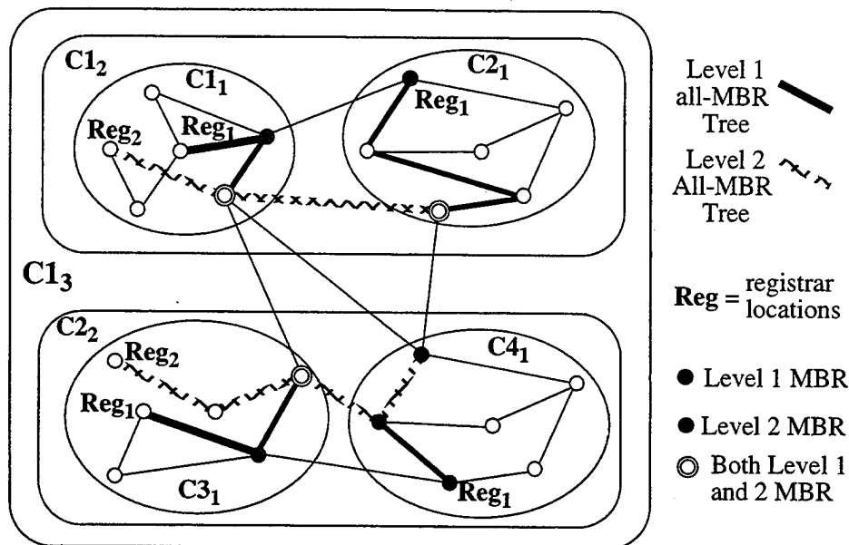
Figure 3.11: All-MBR Trees for a 3 Level, 4 Cluster Hierarchy
