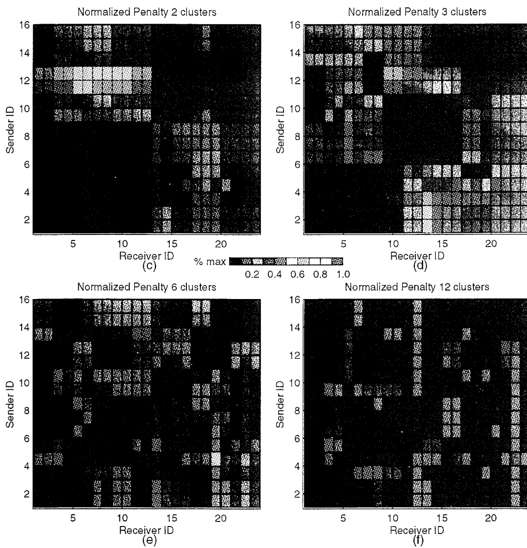
Figure 7.8 Video Conferencing 96 Node Case - Node Degree 4
