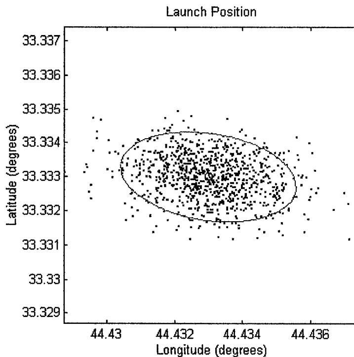
Figure 19. Launch Position Error Ellipse
