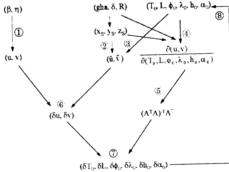
Figure 13. Flowchart Diagram of Iteration Process
