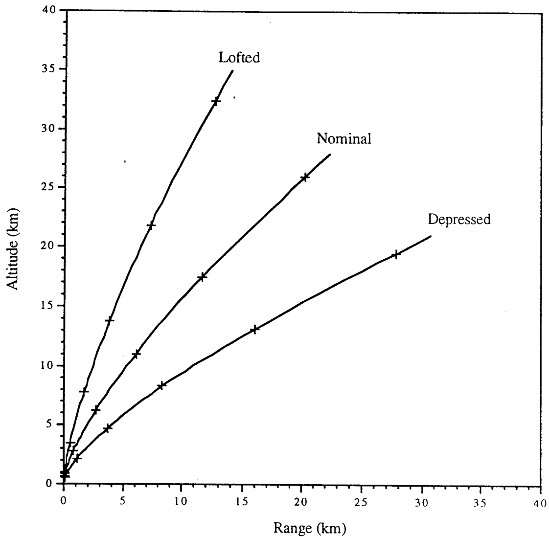
Figure 6. Trajectory Profiles for Three Loft Values
