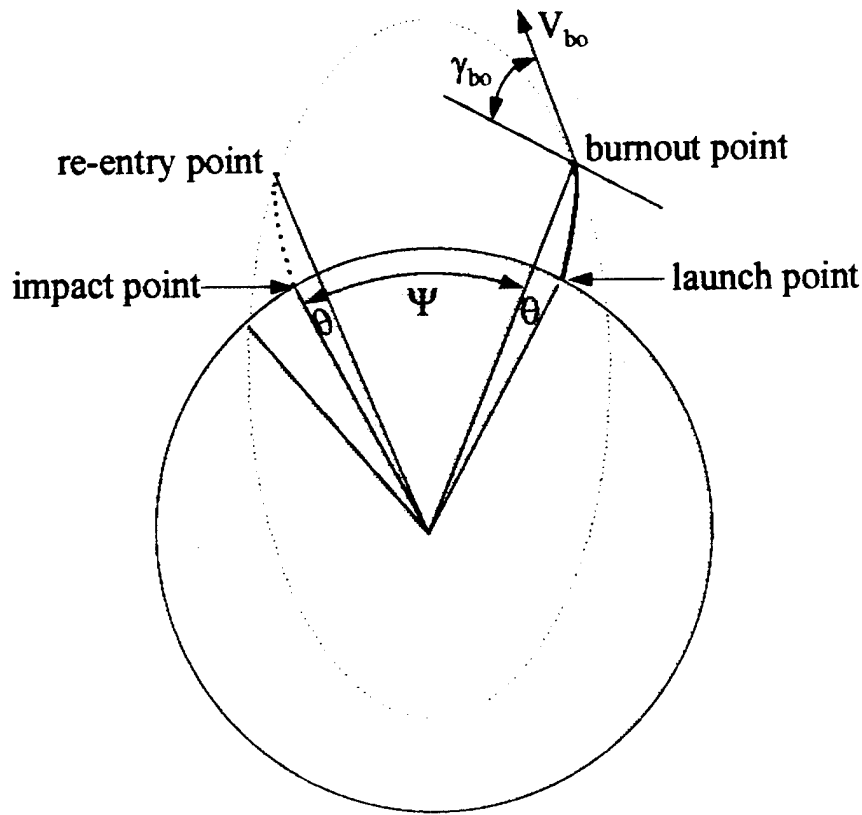
Figure 15. Ballistic Trajectory [Ref. 6]
