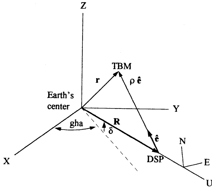
Figure 7. Coordinate Frame Illustration
