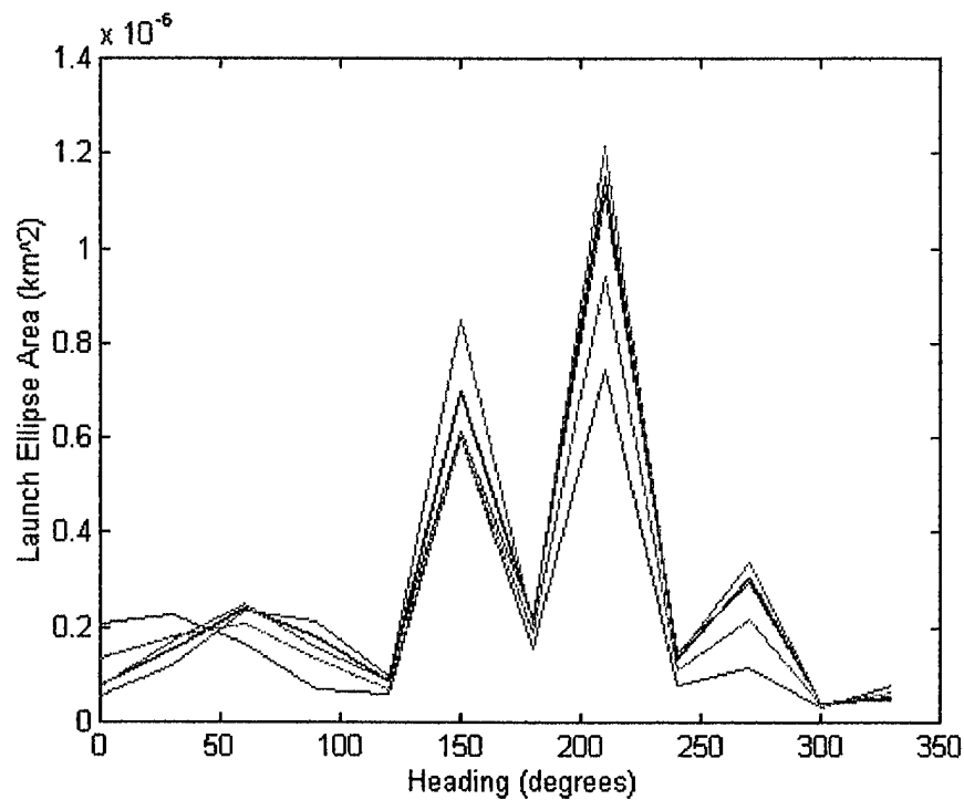
Figure 22. Time Error Effects Upon Launch Ellipse Area
