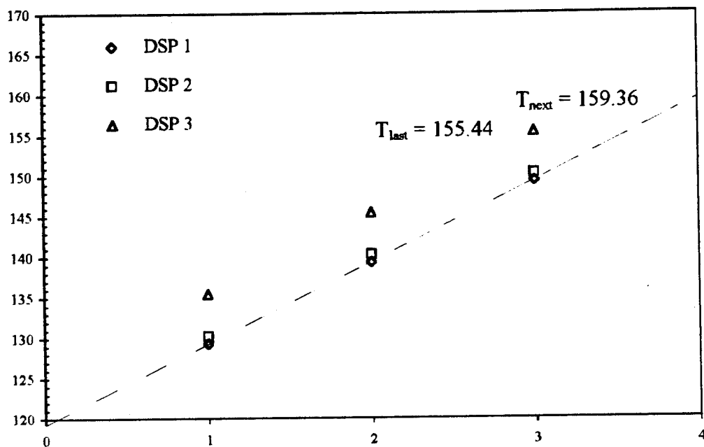
Figure 14. Burnout Time Estimation
