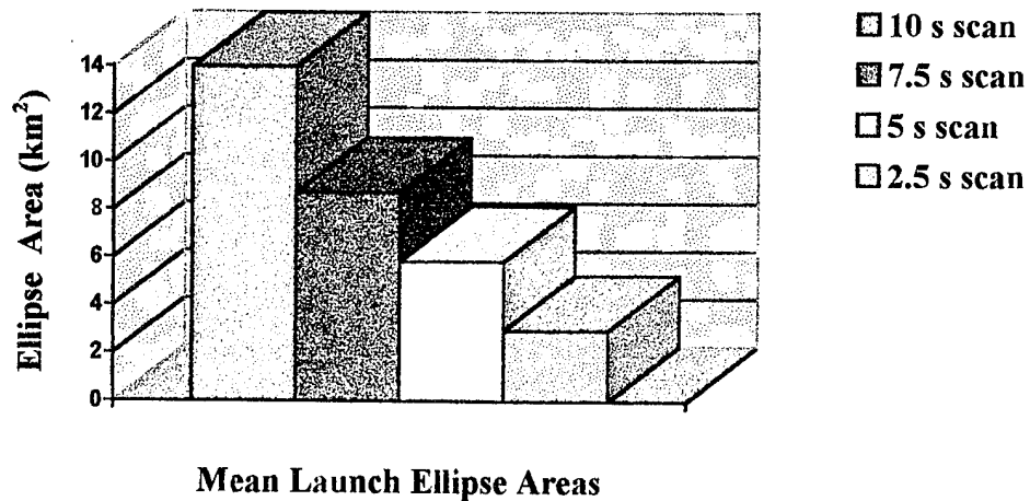
Figure 41. Scan Rate Effects on Launch Ellipse Area
