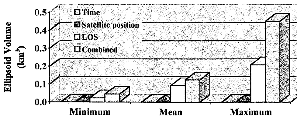
Figure 36. Burnout Ellipsoid Volume Comparison
