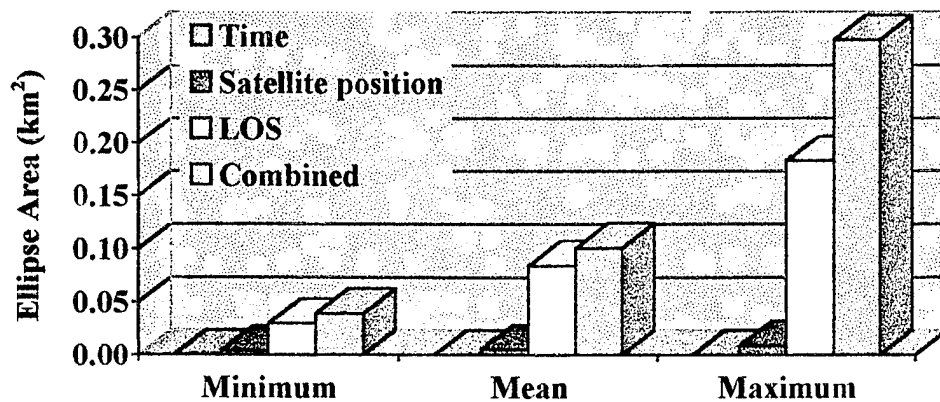
Figure 35. Launch Ellipse Area Comparison
