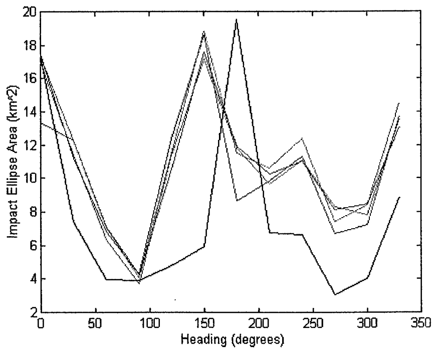
Figure 30. LOS Error Effects Upon Impact Ellipse Area
