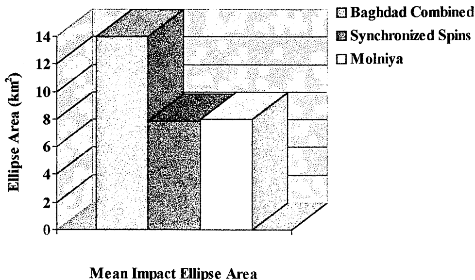
Figure 40. Comparison of Mean Impact Ellipse Areas
