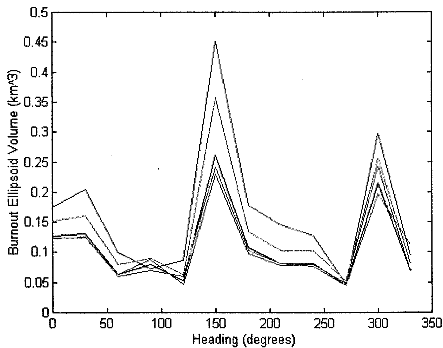
Figure 32. Combined Error Effects Upon Burnout Ellipsoid Volume
