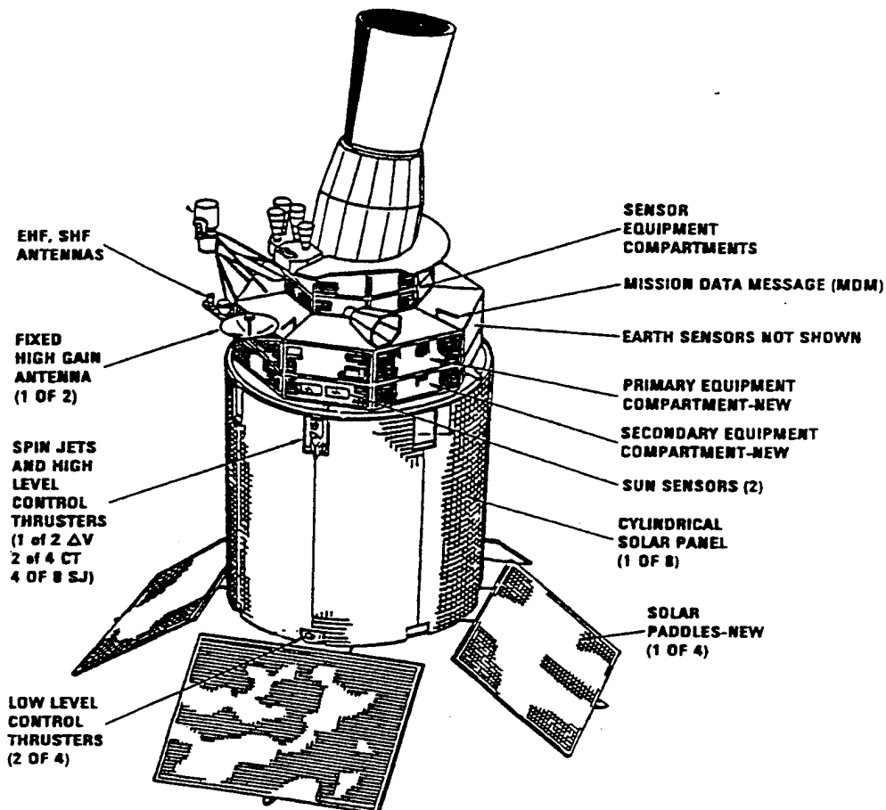
Figure 1. Diagram of DSP Satellite [From Ref. 2]
