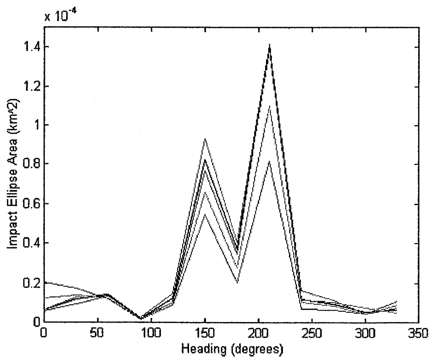
Figure 24. Time Error Effects Upon Impact Ellipse Area
