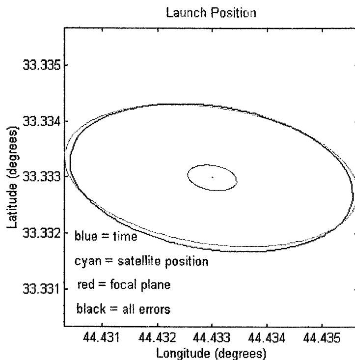
Figure 34. Launch Error Ellipses for Each Error Source
