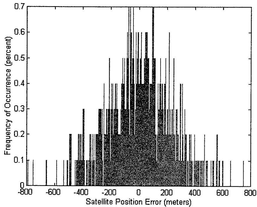
Figure 17. Histogram of Satellite Position Error - Normal Distribution
