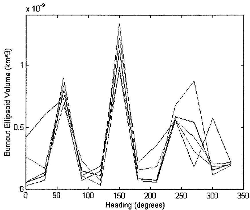
Figure 23. Time Error Effects Upon Burnout Ellipsoid Volume
