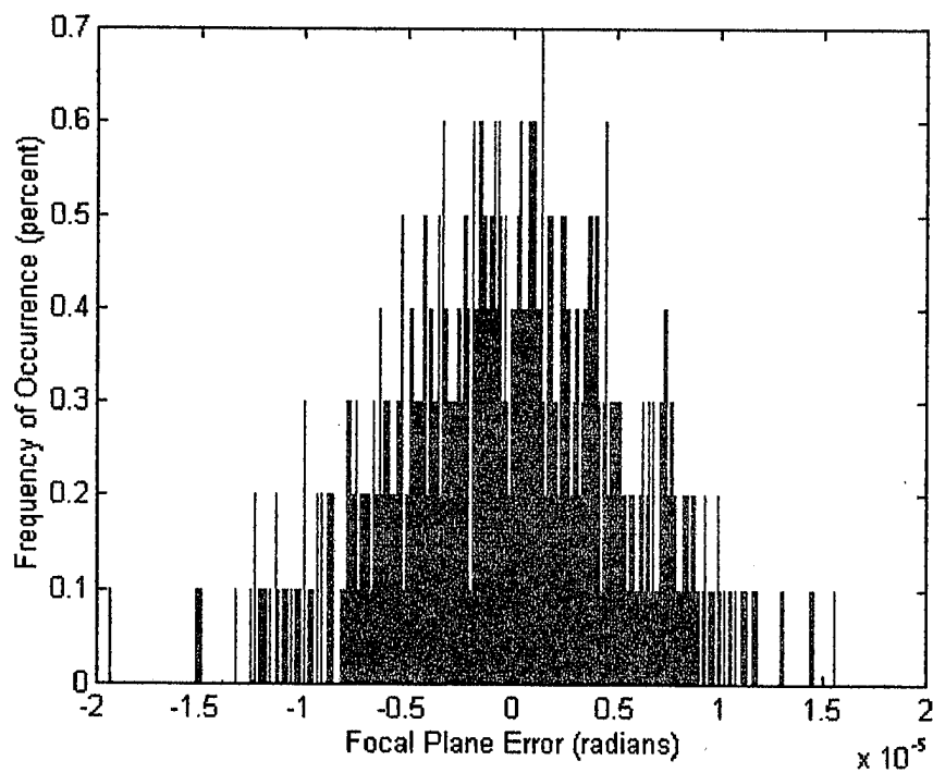
Figure 18. Histogram of LOS Error - Normal Distribution
