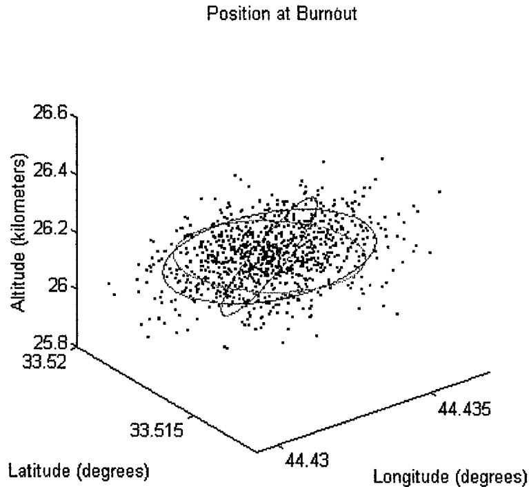
Figure 20. Position at Burnout
