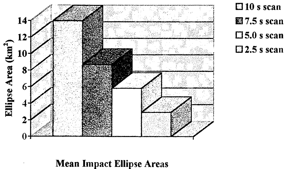
Figure 43. Scan Rate Effects on Impact Ellipse Area
