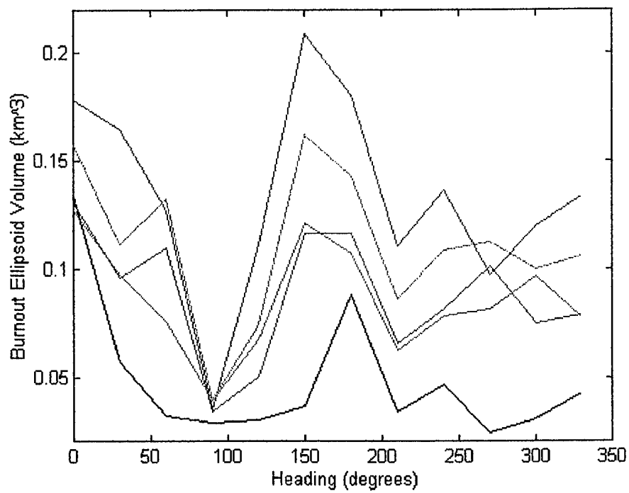
Figure 29. LOS Error Effects Upon Burnout Ellipsoid Volume
