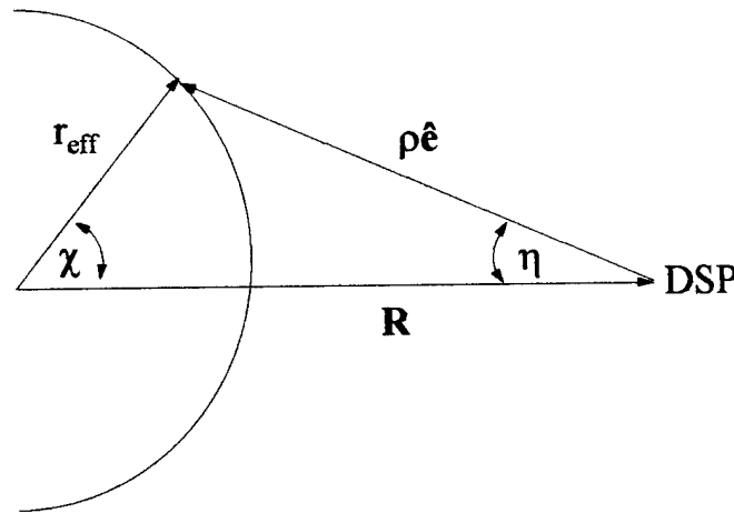
Figure 9. Initial Position Estimate Geometry
