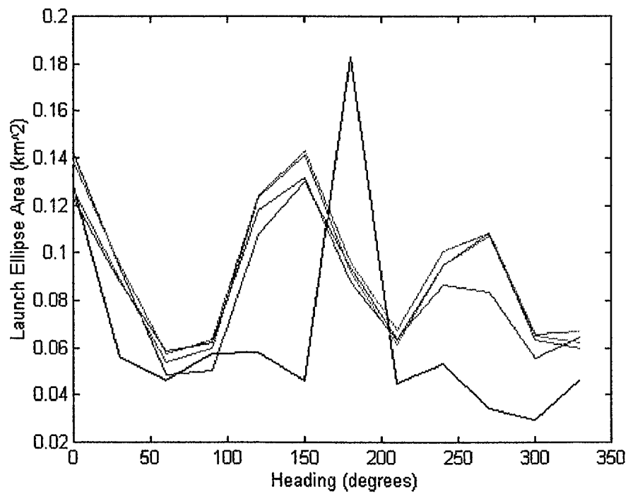
Figure 28. LOS Error Effects Upon Launch Ellipse Area
