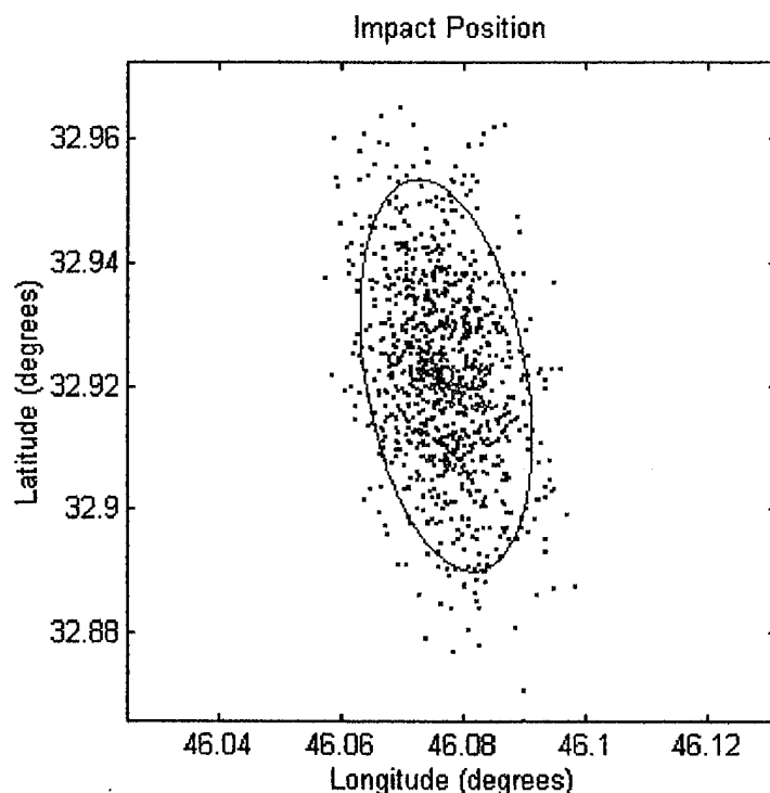
Figure 21. Impact Position Error Ellipse
