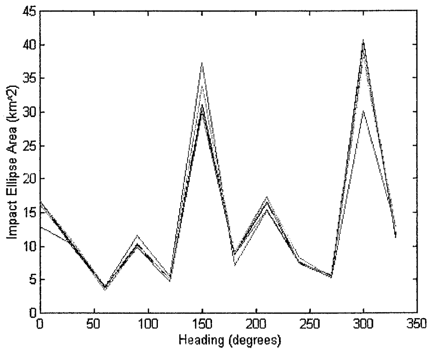
Figure 33. Combined Error Effects Upon Impact Error Ellipse
