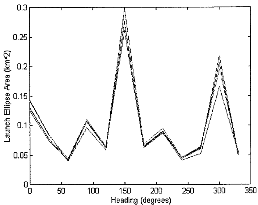
Figure 31. Combined Error Effects Upon Launch Ellipse Area
