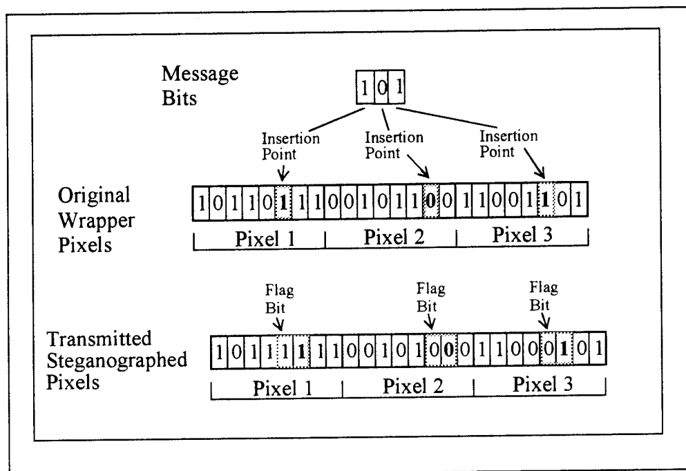
Figure 6: Flat Bit
