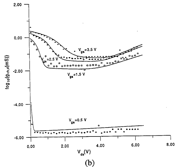
Fig. 4. Source current (a) and channel conductance (b) for a nMOSFET with L_m = 1.5 \mu\text{m} . V_{sb} = 0 . Solid line: model. Symbols: measurements.
