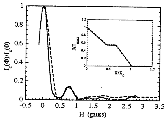
Fig. 2. Field modulations of I_c(H)/I_c(0) for a type A sample at 77 K. Data is the solid line and the FT fit is the dotted line. Inset: The supercurrent distribution that the fit is based on.
