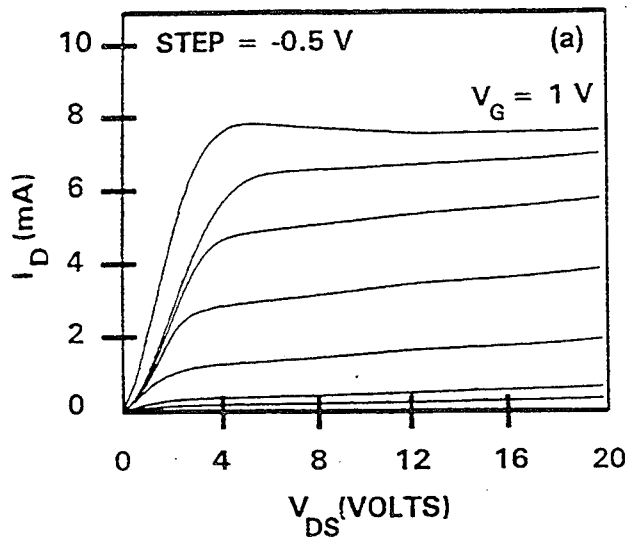
Figure 6. The souece-drain I-V curves of a 0.25 \mu\text{m} long gate and 150 \mu\text{m} wide device.
