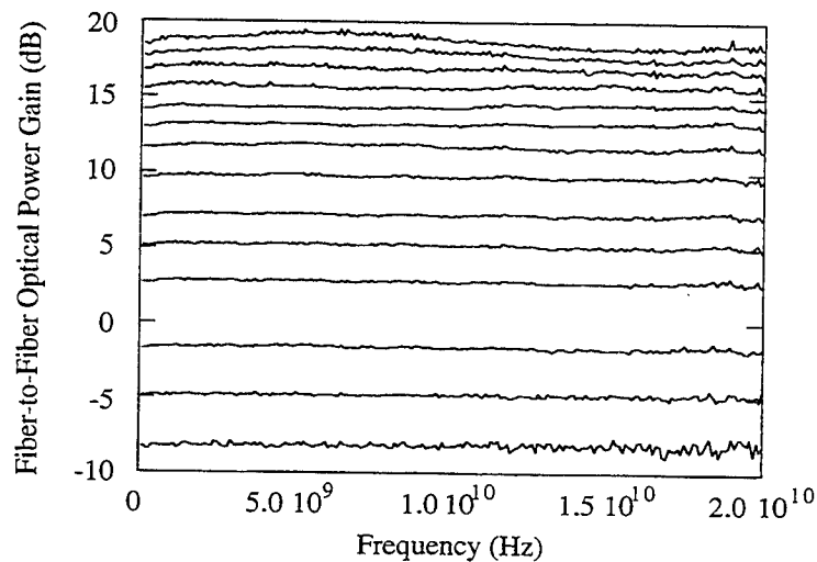
Figure 3. Unsaturated fiber-fiber TE mode gain vs. modulation frequency for amplifier drive currents from 70 mA - 200 mA in 10 mA steps (gain increasing with increasing current)
