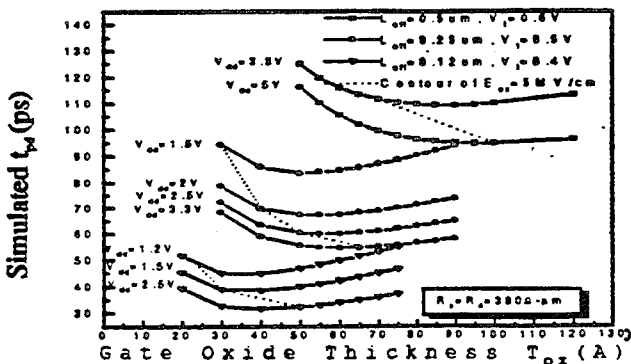
Fig. 15 There exist optimum T_{ox} for given V_{dd} and L_{eff} : a new result from the mobility model.
