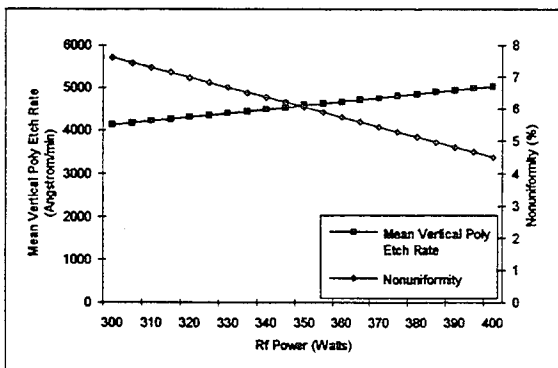
Fig. 1 The poly etch rate and nonuniformity vs. the Rf power.
