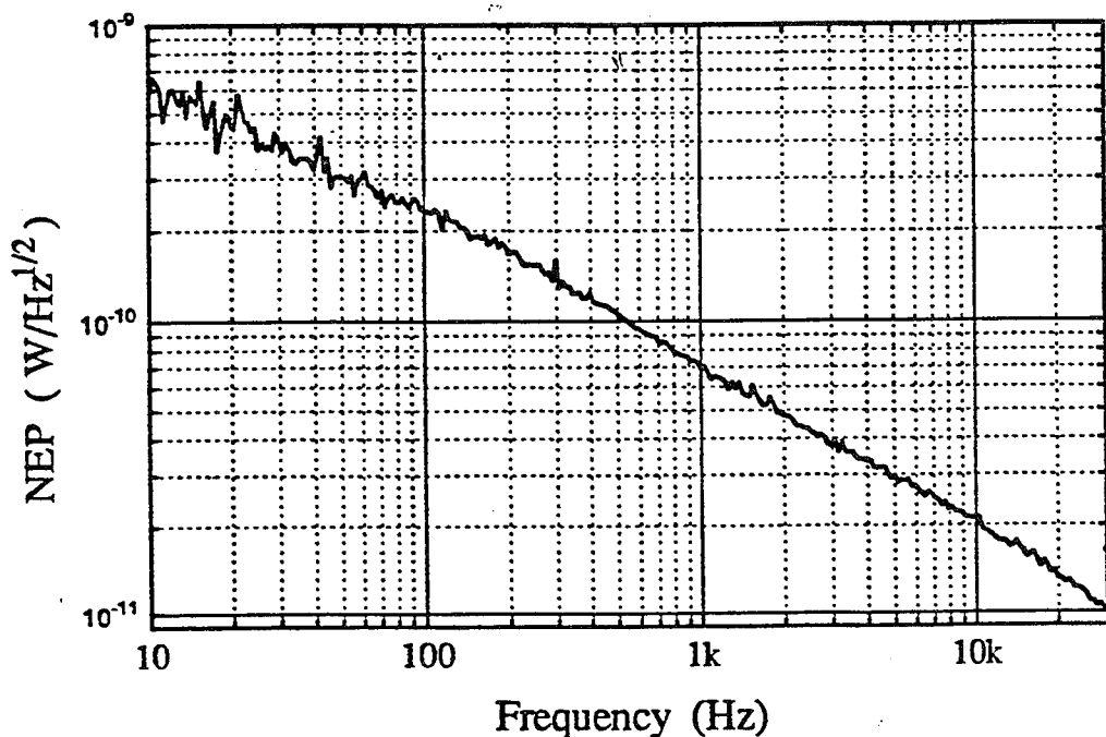
Fig. 3. Noise equivalent power for \nu = 10 GHz microwave radiation ( R_{\nu} = 2.5 \times 10^3 V/W) and modulation frequencies in the range 10 Hz - 30 kHz.
