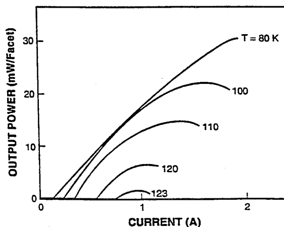
Fig. 6. CW power vs current of InAsSb/InAlAsSb QW laser at several temperatures.
