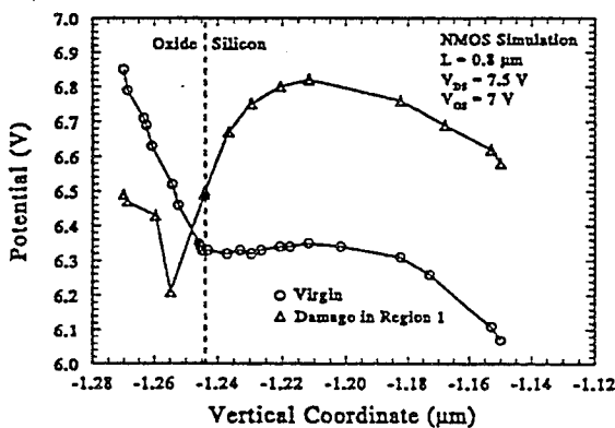
Figure 5. Simulation of the vertical potential profiles at the peak of lateral electron temperature profiles (see fig. 10). \phi_b of -0.6\text{eV} as observed in fig. 4 is obtained in simulation here with the damage located in Region 1 of fig.10.
