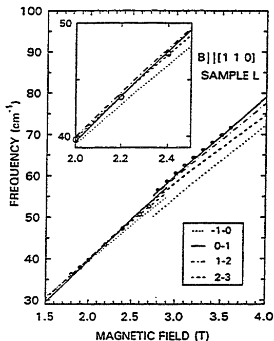
Fig. 3: Emission frequency of low doped lasers as a function of applied magnetic field. Circles indicate the experimental data. The lines show the theoretical results for n = -1 to 0 , n = 0 to 1 , n = 1 to 2 , and n = 2 to 3 in the Landau level transitions in the b-set.
