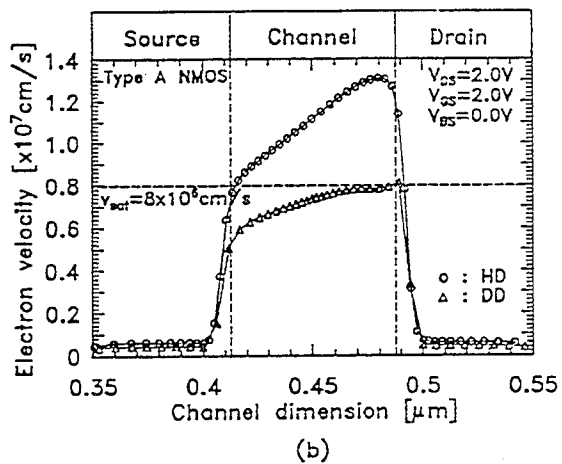
Figure 1: (a) The profiles of the areal electron density( N_{inv} ) and (b) electron velocity( v_n ) from the HD and DD simulations.
