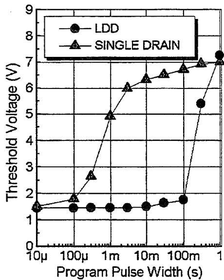
Fig. 8. CHE programming characteristics for the single-poly EEPROM cell with single drain and LDD structures ( V_{CG}=12V , V_D=6V , V_S=0V , coupling ratio = 0.8, p+ control gate).
