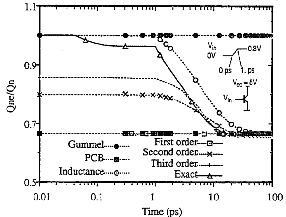
Fig 4 : Comparison of the transient variation of charge flowing through emitter terminal ( Q_{ne} ) for the different models and the exact solution (solid line) When V_{be} increase from 0v to 0.8v in 1ps.
