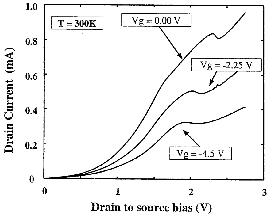
Fig.2 Drain to source currents for a 0.8μm x 10μm device at various gate biases. Gate leakage currents at all biases were below 1μA.
