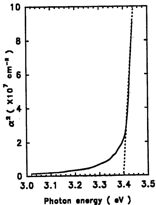
Fig. 3 Absorption coefficient square ( \alpha^2 ) of GaN vs. photon energy h\nu .
