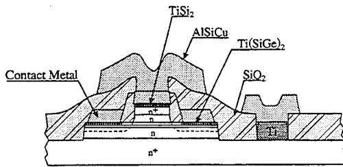
Fig. 2: Schematic cross-section of the Si/SiGe HBT
