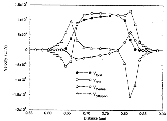
Figure 3: The channel velocity and its components obtained from the HD model in the SOI N-MOSFET using c = -0.5 . The drain bias, the back-gate bias, and the front-gate bias are 1.5V, 64V, and -3V, respectively.
