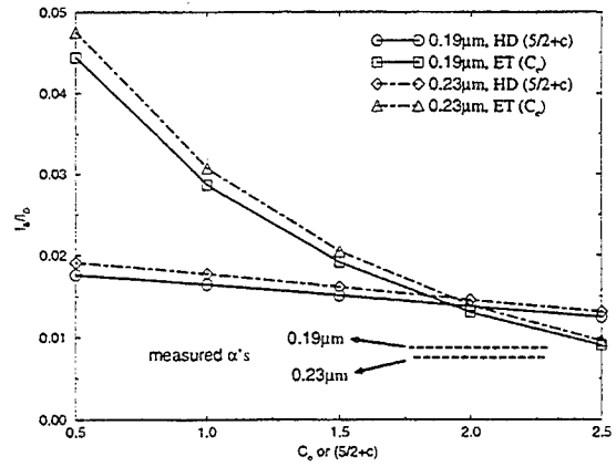
Figure 7: The dependence of I_B/I_D on 5/2 + c and C_e , in the HD model and in the ET model, respectively for the LDD MOSFETs with channel lengths of 0.19 \mu\text{m} and 0.23 \mu\text{m} . The measured \alpha 's are denoted by the dashed line.
