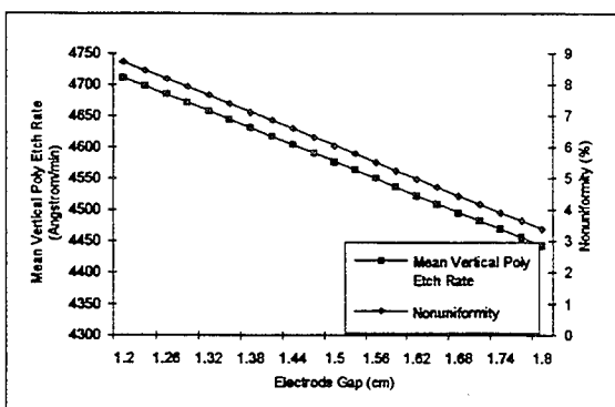
Fig. 3 The poly etch rate and nonuniformity vs. the electrode spacing.
