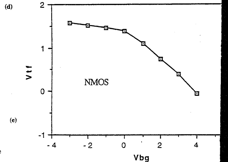
Figure 4. Threshold voltage shift for N-channel DG-TFSOI MOSFET versus applied backgate voltage (
