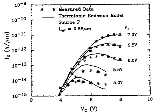
Figure 5: Comparisons of simulated and experimentally measured I_G - V_G curves for the Source F LDD device with L_{eff} = 0.68 \mu\text{m} .
