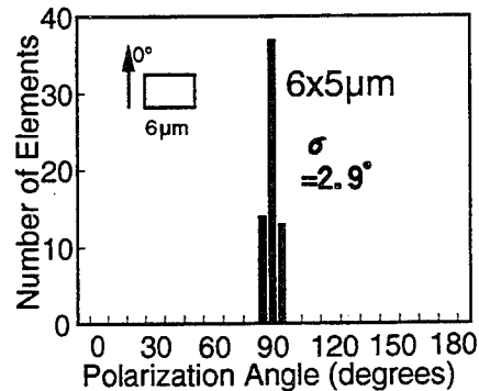
Fig. 4 Polarization angle of the 6\times 6\mu\text{m} size polarization uncontrolled array and the 6\times 5\mu\text{m} polarization controlled array. The deviation angle is only 2.9^\circ for the 6\times 5\mu\text{m} array
