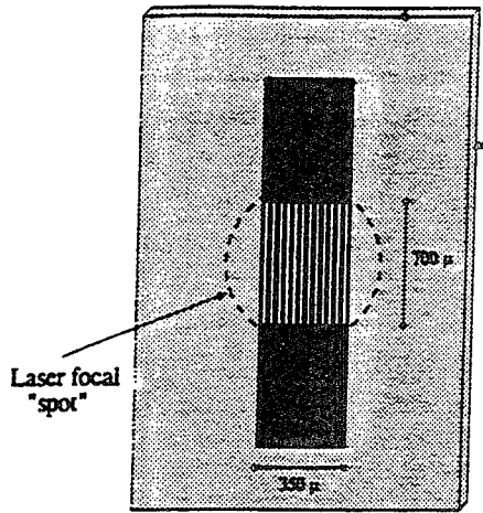
Figure 1. NbN device for the 2.5 THz mixer.
