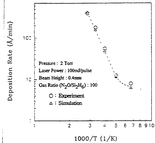
Figure 10. Deposition rate vs. Substrate temperature
