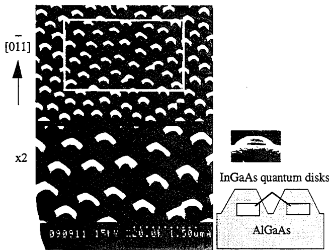
Fig. 1. SEM images with a schematic cross-sectional view of as-grown InGaAs on a GaAs (311)B substrate. The layer beneath is an AlGaAs film. The self-organization seems to result from the barrier height for adatom migration being lower than that of the (100) surface.
