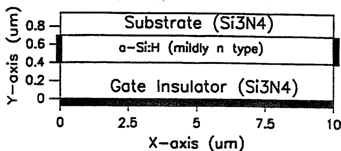
Fig.1 (b) The rectangular geometry of a-Si:H TFTs.
