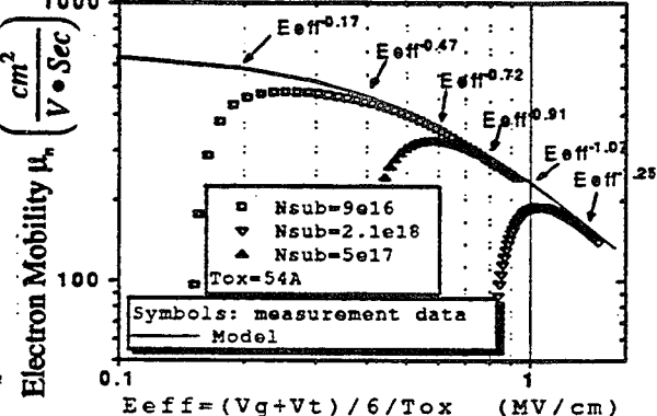
Fig. 12 Electron mobility's E_{eff} power dependence. of phonon scattering are increased with E_{eff} .
