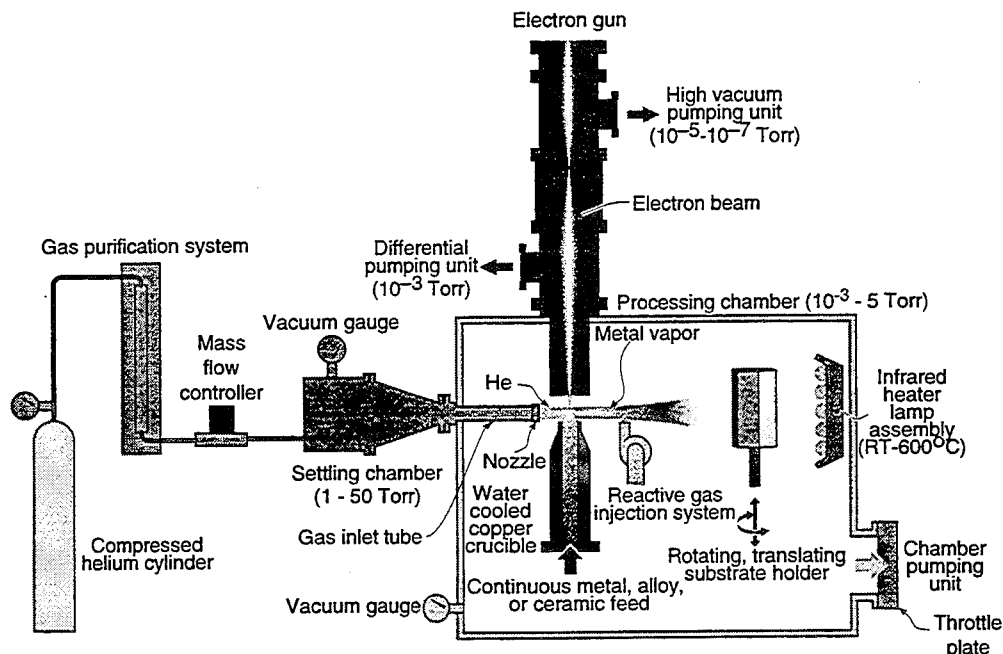
Fig. 1 The primary DVD configuration combines a purified gas flow with evaporant from an e-beam source to enable high rate vapor deposition.
