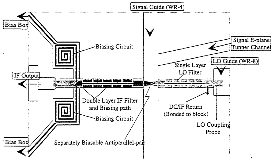
Figure 1. The center portion of the lower half of the mixer split-block that houses biasable diodes and microstrip circuits.
