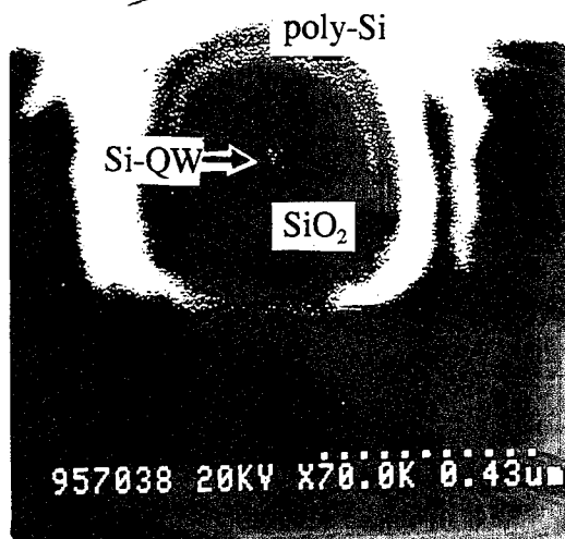
Figure 2. Cross-sectional image of SEM of thinned SQW with the lateral linewidth of \sim 40\text{nm} .
