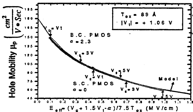
Fig. 11 SC vs BC PMOS for the same V_t and T_{ox} . BC achieves the same \mu_p at 2V lower V_t than SC PMOSFET.
