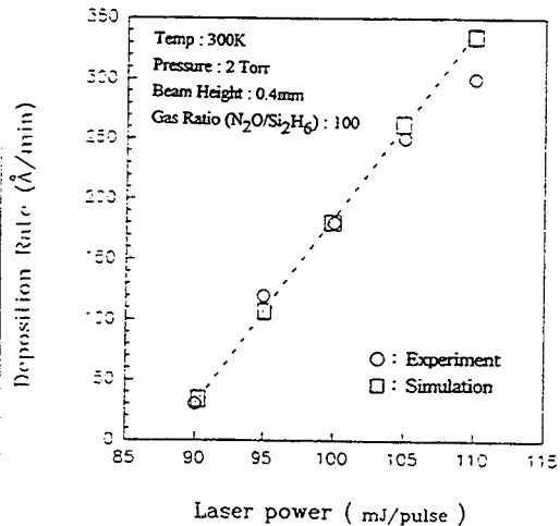
Figure 11. Deposition rate vs. Laser power
