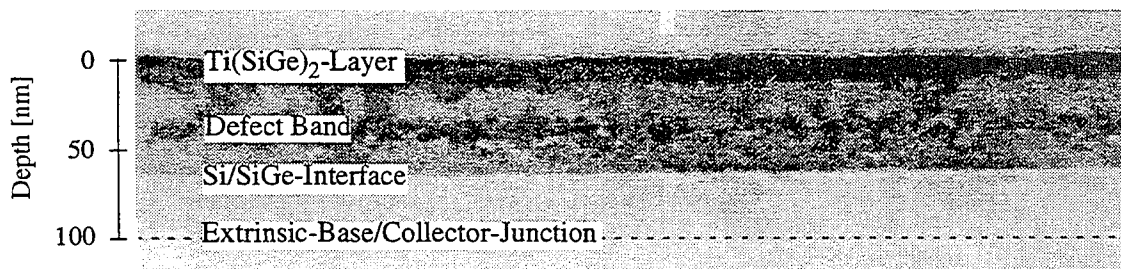
Fig. 4: Cross-sectional TEM micrograph of a \text{BF}_2 -implanted SiGe base layer. Silicidation of 10nm Ti, recrystallisation and dopant-activation were performed simultaneously at 650^\circ\text{C} for 300s.
