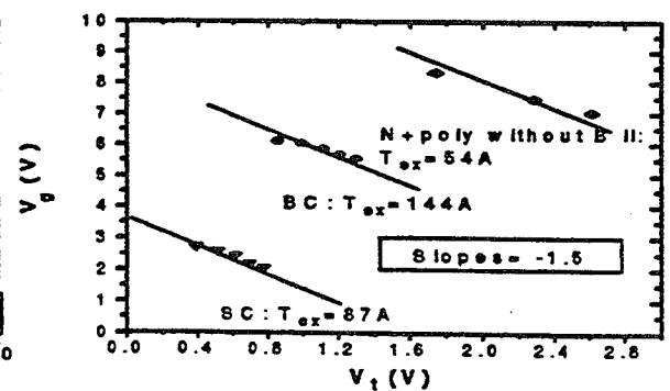
Fig. 8 The slope = -1.5 indicating that \eta=2.5 for PMOSFET holes.
