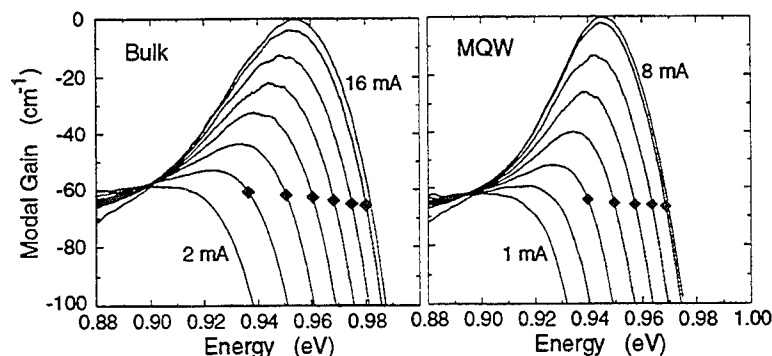
Figure 1. Families of measured gain spectra as a function of photon energy for the indicated ranges of device current for a bulk active and a MQW active laser at 25 C.
