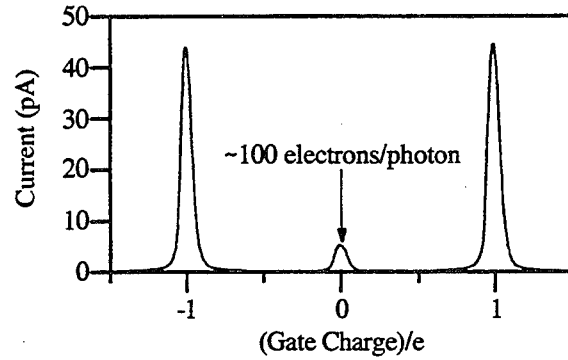
Fig. 4. Experimental incomplete-shielding I-Q_o curve for an SSS SET transistor at V = 20 \mu\text{V} and T_{MC} = 15 mK. Note the larger current scale in comparison with Fig. 3. Near Q_o = 0 , this particular device absorbs about 200 aW of microwave power and this produces a sizeable secondary peak. Since the device acts as a single-photon-activated switch, the secondary peak can correspond to the tunneling of many electrons for every absorbed photon.
