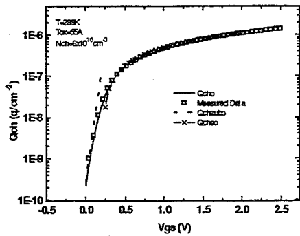
Fig. 1 Comparisons between unified charge model and piecewise models in subthreshold and strong inversion regions. Qch0 is the model result from (1), Qchso and Qchsub0 are the model results from the charge expressions in previous BSIM3 model in strong inversion and subthreshold regimes respectively.
