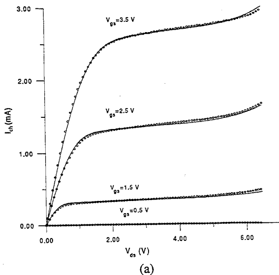
Fig. 4. Source current (a) and channel conductance (b) for a nMOSFET with L_m = 1.5 \mu\text{m} . V_{sb} = 0 . Solid line: model. Symbols: measurements.
