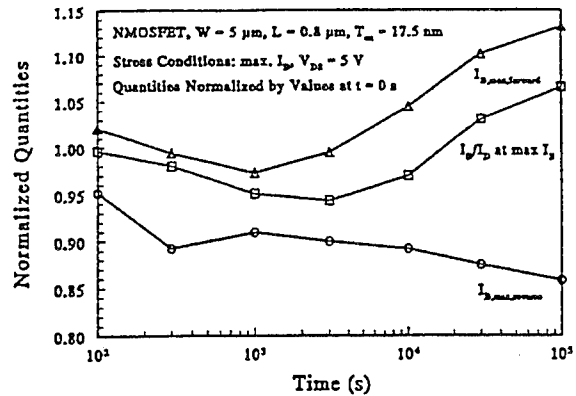
Figure 2. Both I_{B,max} and I_B/I_D at max. I_B measured in the forward mode drop in the initial phase. As we show later, this does not mean that the electron temperature is falling. In the reverse mode I_{B,max} falls all the way as in conventional degradation.
