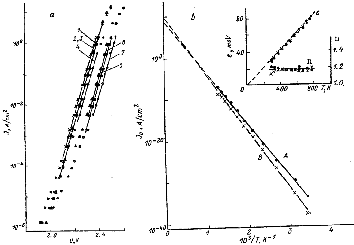
Fig. 1. a) Room temperature current-voltage characteristics J=J_0 \exp[qU/(nkT)] of several pn structures with n=6/5 : 1-4 - II structures, 5-7 - LPE structures; b) temperature dependence of the preexponential factor J_0 , of the characteristic energies \epsilon=nkT , and of the coefficient n for II structure (A) and LPE structure (B) [5].
