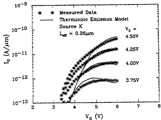
Figure 6: Comparisons of simulated and experimentally measured I_G - V_G curves for the Source K LDD device with L_{eff} = 0.26 \mu\text{m} .
