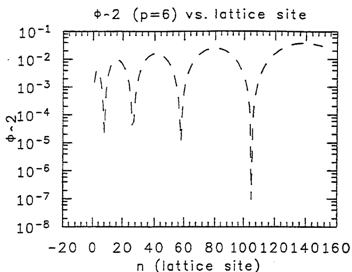
Figure 2. |\Phi_{p,n}|^2 vs. n , this time for p = 6 .
