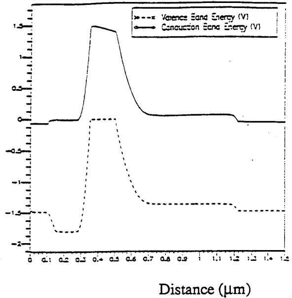
Figure 2. Energy Band Diagram for Graded Al x GaAs Base HBT ( V_{BE}=V_{CE}=0 V, W_B=2000 Å)
