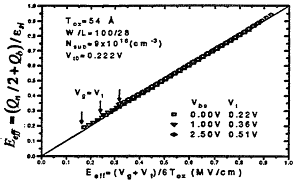
Fig. 2 Two E_{eff} comparison for three different technologies.
