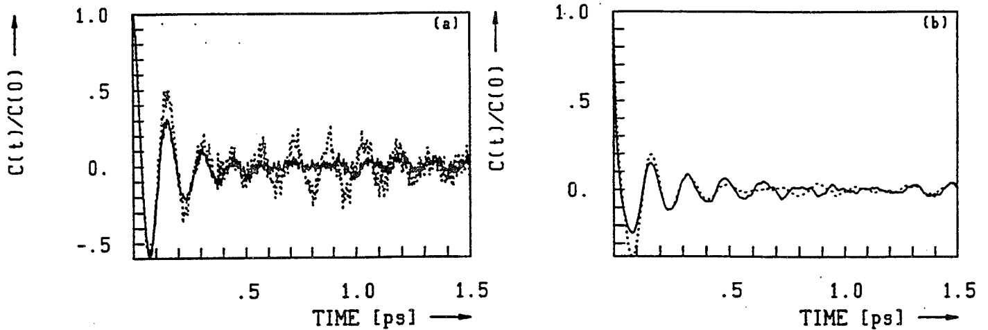
Fig.3 Drain (a) and gate (b) current autocorrelation functions. V_d=2V , V_g=.6V (solid line), V_g=-.2V (dashed line)
