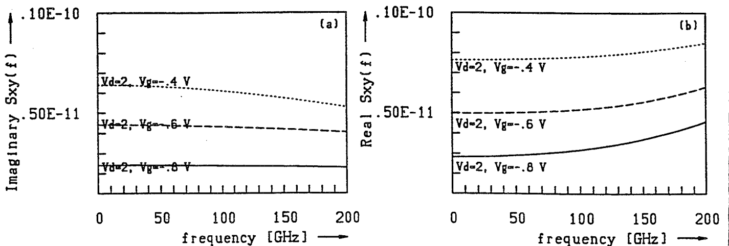
Fig.5 2DEG channel (a) and gate-drain (b) noise current spectral densities in regions V and III, respectively, of fig.1.
