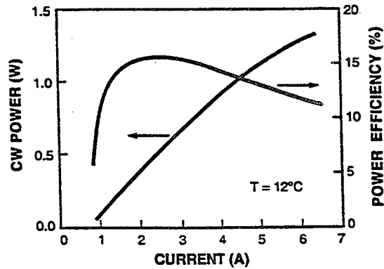
Fig. 2. CW output power vs current for a 1000- \mu\text{m} -long GaInAsSb/AlGaAsSb QW laser.
