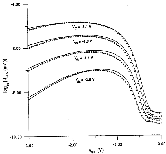
Fig. 2. I_{sub} for a pMOSFET with L_m = 1.5 \mu\text{m} . V_{sb} = 0 . Solid line: model. Symbols: measurements.
