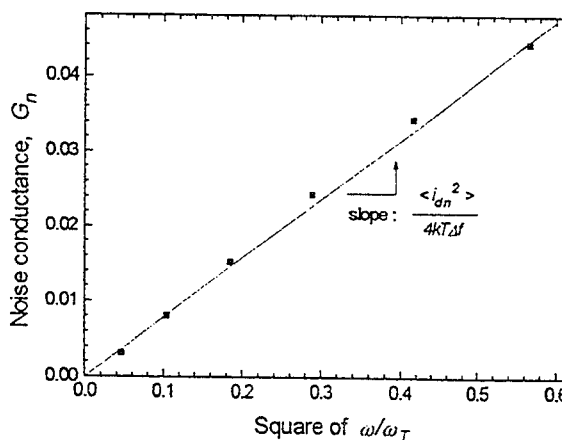
Fig.2. G_n vs. (\omega / \omega_T)^2 plot at V_{GS}, V_{DS}=0.0, 3.0V .
