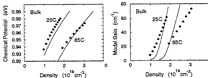
Figure 4. Comparison of the model (lines) to experiment (solid circles) for the chemical potential and peak modal gain as a function of density for the bulk active 1.3 \mu\text{m} device at room temperature and 85 C.
