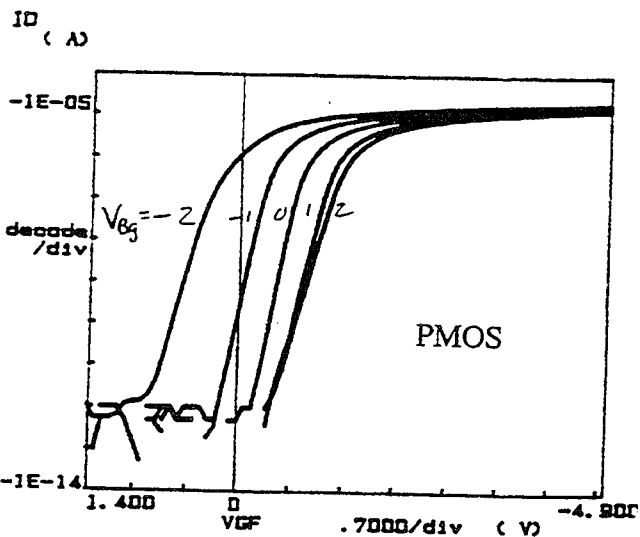
Figure 5. Topgate subthreshold characteristics versus backgate voltage ( V_{bg} ) for P-channel DG-TFSOI MOSFET.
