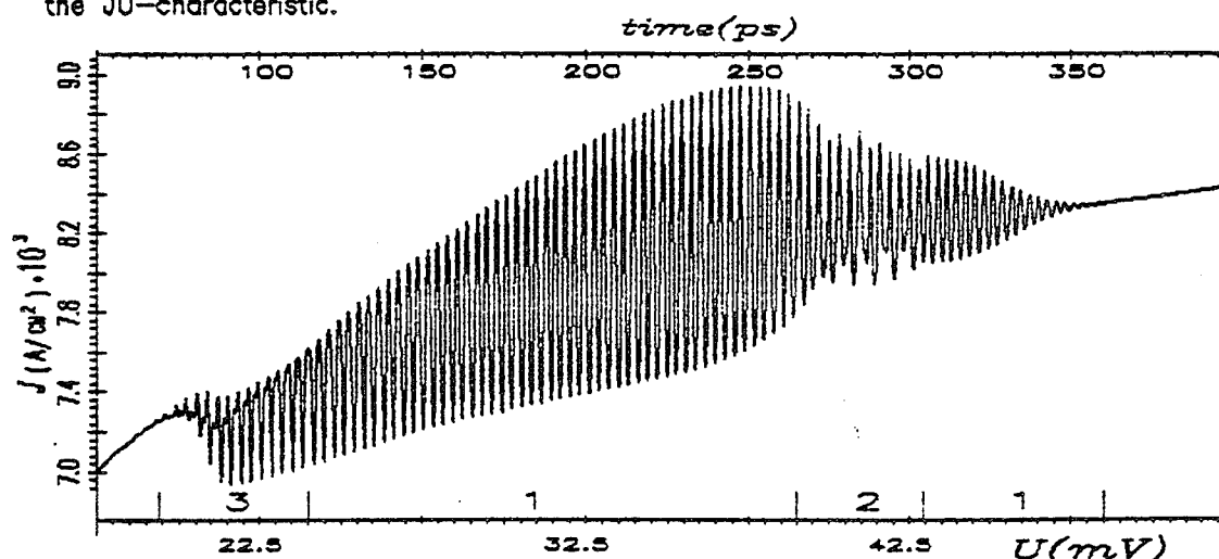
Fig.4. Typical oscillations of ballistic hole current for compressed p-Ge: T=4.2 K, l=1 \mu m, n_0=3 \cdot 10^{15} \text{cm}^{-3} , compression 0.2%. Ranges of oscillations: 1—quasilinear, 2—regular nonlinear, 3—irregular nonlinear. Oscillations have obtained by numerical method described in detail in [2].
