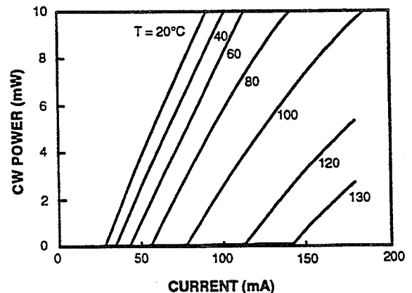
Fig. 4. CW output power vs current of a GaInAsSb/AlGaAsSb ridge-waveguide laser at temperatures between 20 and 130°C.
