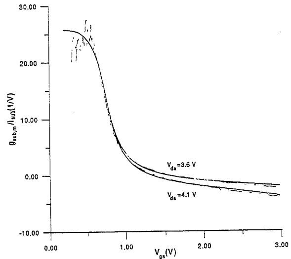
Fig. 3. g_{sub,m}/I_{sub} for an nMOSFET with L_m = 1.2 \mu\text{m} . V_{sb} = 0 . Solid line: model. Symbols: measurements.
