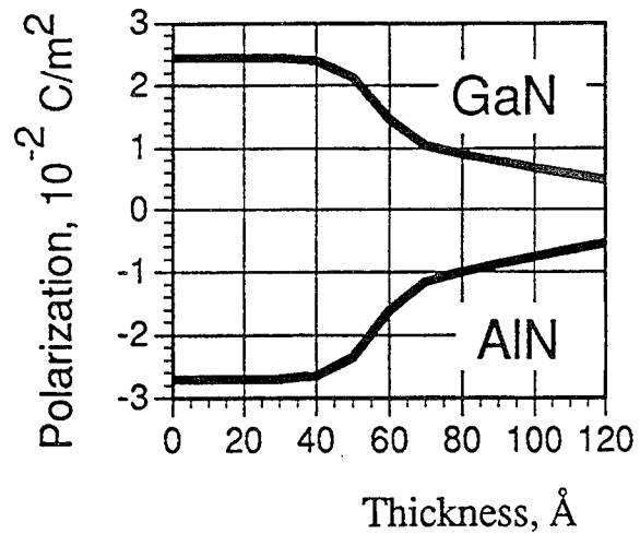
Fig. 3. Strain-induced polarization in (0001) direction as a function of L .
