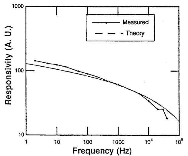
Fig. 3. Calculated and measured voltage responsivities of a 10nm thick microbolometer. Theoretical values were calculated by assuming a 2-D point source radiating heat in the membrane along the radial direction.
