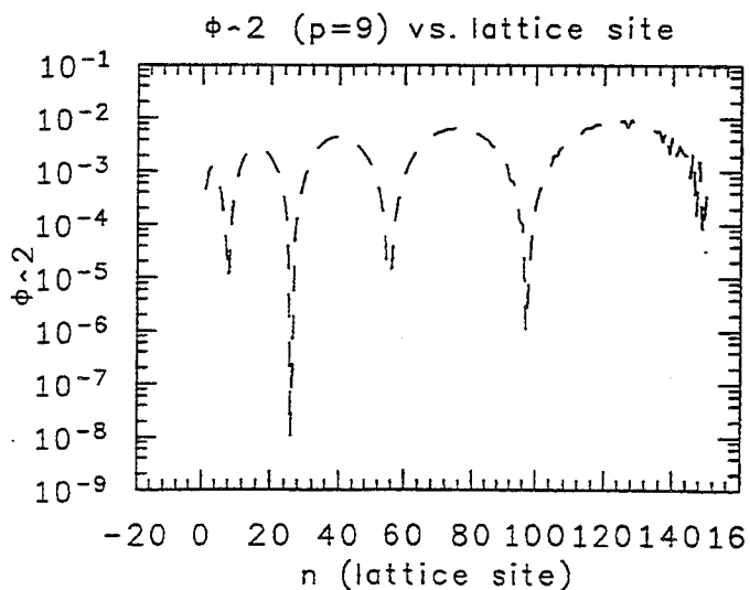
Figure 4. |\Phi_{p,n}|^2 for p = 9 .
