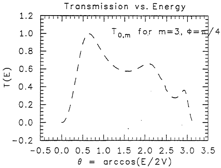
Figure 1. Transmission vs. Energy for zero initial phonons and three final phonons. Magnetic flux ratio = \pi/4 .
