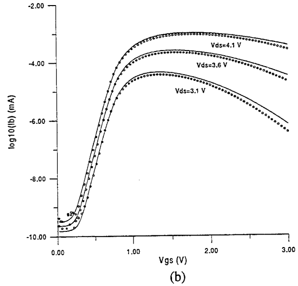
Fig. 1. I_{sub} for nMOSFETs with (a) L_m = 1.2 \mu\text{m} and (b) L_m = 1.5 \mu\text{m} . Solid line: model. Symbols: measurements.
