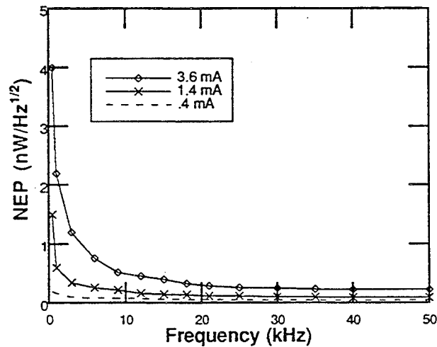
Fig. 6. Electric Noise Equivalent Power (NEP) of a 10nm thick microbolometer at various bias current.
