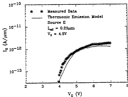
Figure 3: Comparisons of simulated and experimentally measured I_G - V_G curves for the Source E LDD device with L_{eff} = 0.29 \mu\text{m} .
