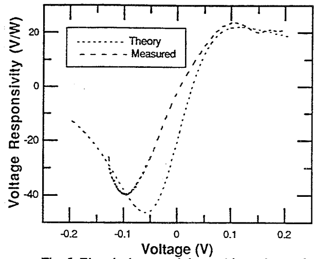
Fig. 5. Electrical responsivity vs. bias voltage of a 10nm microbolometer. Theoretical values were calculated by using the Jones' expression.
