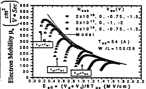
Fig. 4 NMOSFETs of different V_t (by varying V_{bs} ) observe the universal model.
