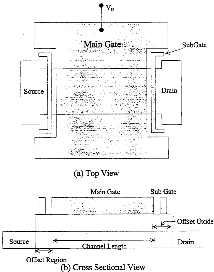
Fig. 1 The schematic view of the proposed TFT
