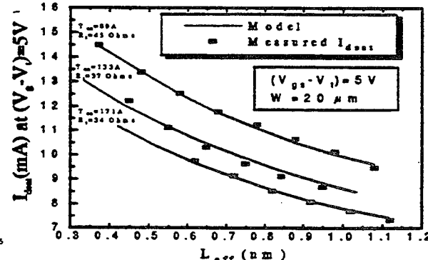
Fig. 14 I_{d,drain} modeling is found accurate for different LDD NMOS technologies.
