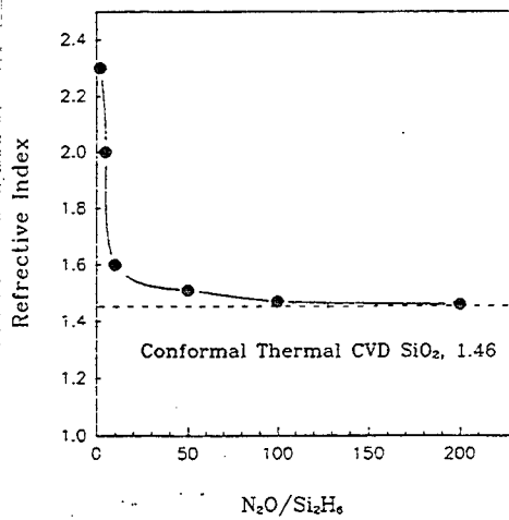
Figure 7. Refractive Index vs. Gas ratio
