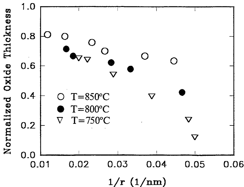
Figure 3. Oxide thickness on SQW surfaces normalized to that on the flat surface as a function of the inverse of the radius of the SQWs for 850^{\circ}\text{C} , 800^{\circ}\text{C} and 750^{\circ}\text{C} wet oxidation, respectively.
