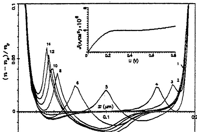
Fig.2. Stationary concentrations of the carriers in the doped bases ( n_0 is the equilibrium cathode concentration) for a set of voltages ( U=0.1-0.8 V, where N_0 is the number at curve). Inset shows the JU -characteristic.
