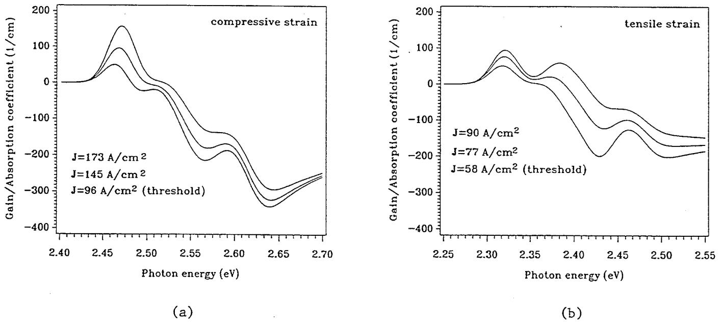
Fig. 2 Computed gain/absorption coefficient for ZnCdSe-ZnMgSSe quantum wire laser: (a) Compressively strained active layer. (b) Tensile strained active layer
