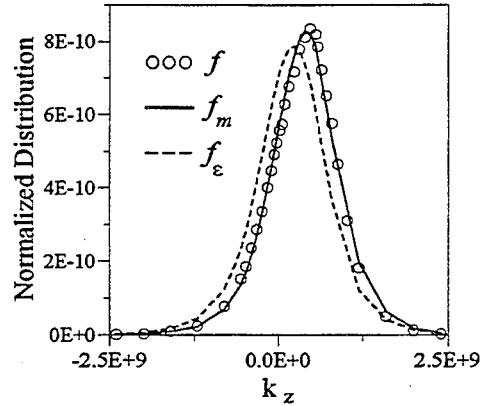
Fig. 3 The distribution near the peak of the velocity overshoot at the slower increase in field.
