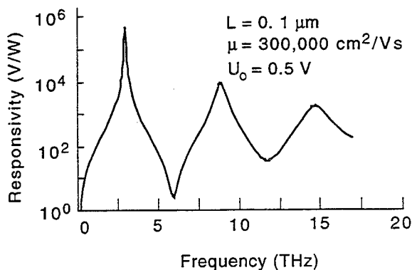
Fig. 1. Responsivity of a HEMT detector versus radiation frequency. (The viscosity of the electronic fluid is accounted for. Without viscosity, all resonance peaks would have equal magnitudes, approximately 10^7 V/W.)
