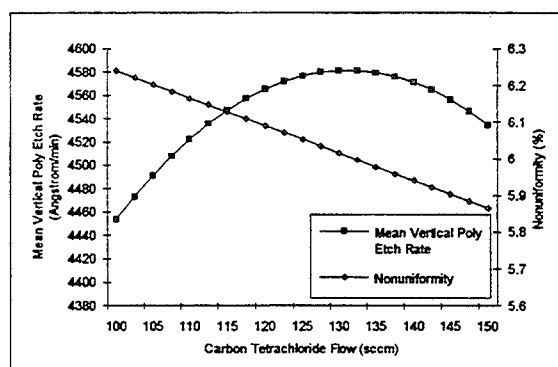
Fig. 4 The poly etch rate and nonuniformity vs. the CCl 4 flow.
