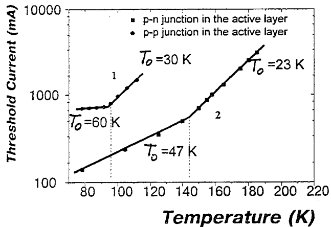
Fig.3. Temperature dependence of threshold current for two laser structures with type II broken-gap heterojunction in an active layer.
