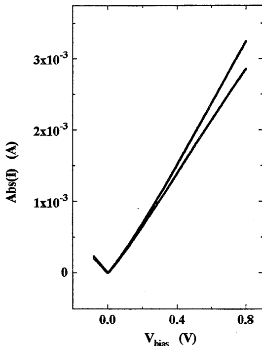
Fig. 1 Current-voltage characteristics at room temperature with and without microwave irradiation (incident power P_i = 4 \times 10^{-5} \text{ W} , \theta = 0^\circ ).
