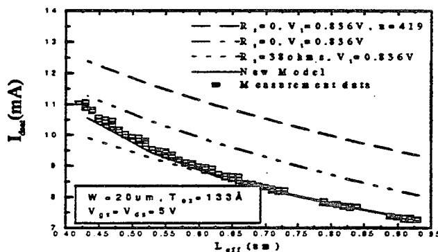
Fig. 13 I_{d,drain} modeling is found accurate with the new mobility model for LDD NMOSFET.
