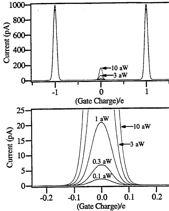
Fig. 5. (a) Theoretical I-Q_o curves for an optimal SSS SET transistor microwave detector (maximum supercurrent of 1 nA, escape time of 1 \mu s) for different amounts of absorbed power. These curves are calculated for V = 20 \mu V and T = 50 mK and are labeled by the power the device absorbs at Q_o = 0 . (b) A blowup of the region near Q_o = 0 . Note that the absorption of only 0.1 aW produces a 2 pA secondary peak, a current that is easily measured.
