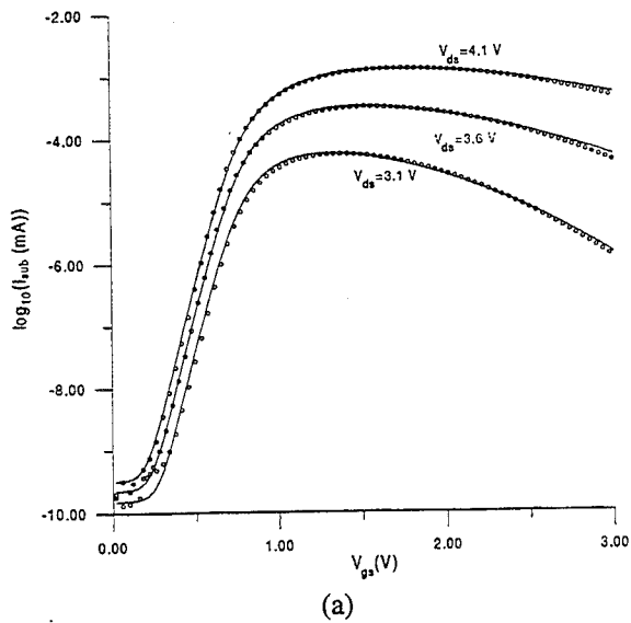
Fig. 1. I_{sub} for nMOSFETs with (a) L_m = 1.2 \mu\text{m} and (b) L_m = 1.5 \mu\text{m} . Solid line: model. Symbols: measurements.
