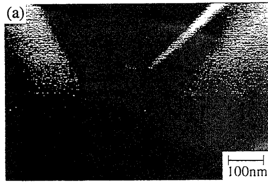
Figure 3 An SEM image of InAs dots grown on the bottom of a group of 6 inverted tetrahedrons.
