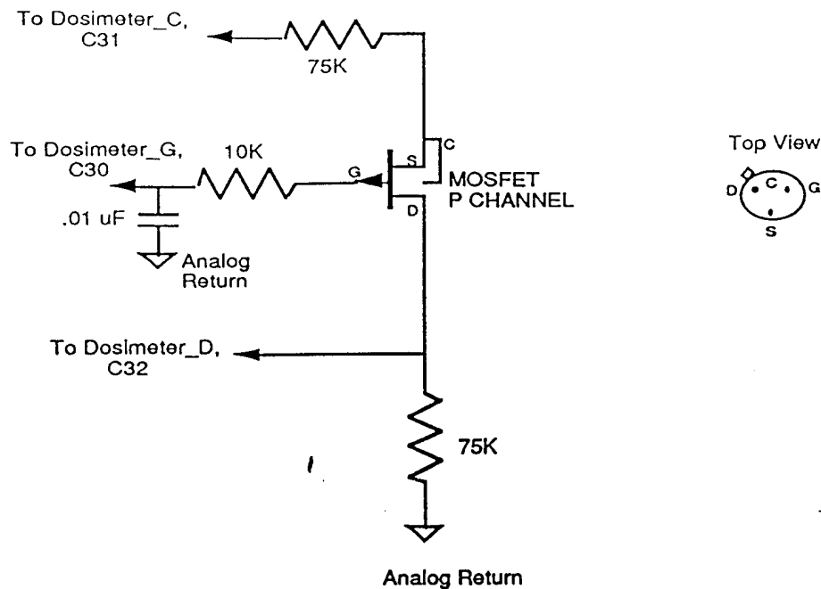
Figure 8 - Dosimeter Circuitry
