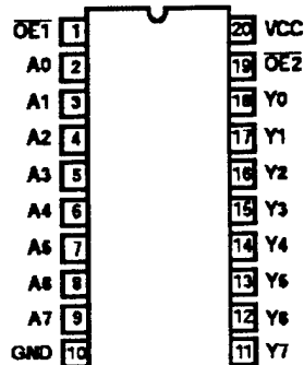
20 LEAD CERAMIC DUAL-IN-LINE METAL SEAL PACKAGE (SBDIP) MIL-STD-1835 CDIP2-T20 TOP VIEW
