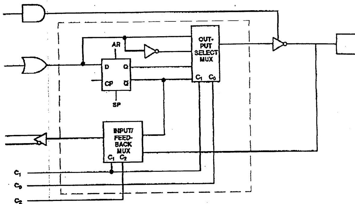
Figure 2. Macrocell
