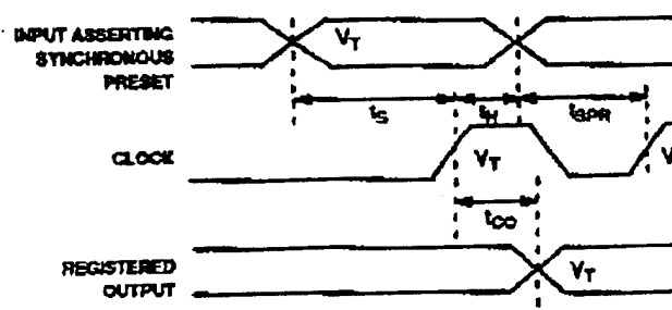
Synchronous Preset
