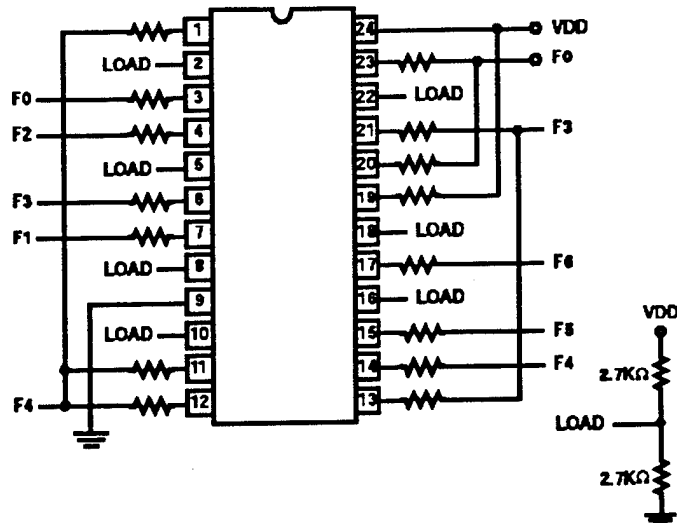
DYNAMIC CONFIGURATION
