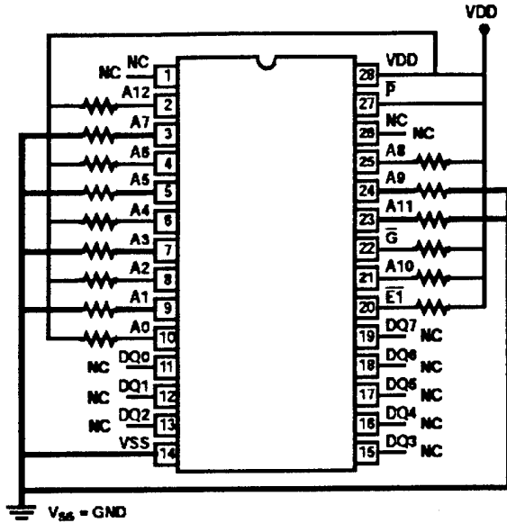
STATIC CONFIGURATION
