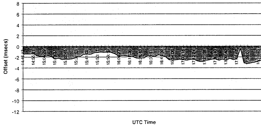
Figure 4: Synchronization of IST Stratum 2 (Logger) to Veda Stratum 1
