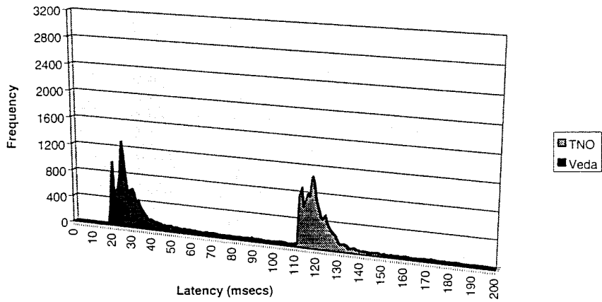
Figure 8: Latency distribution of IST PDU's to TNO and Veda during heavy network load
