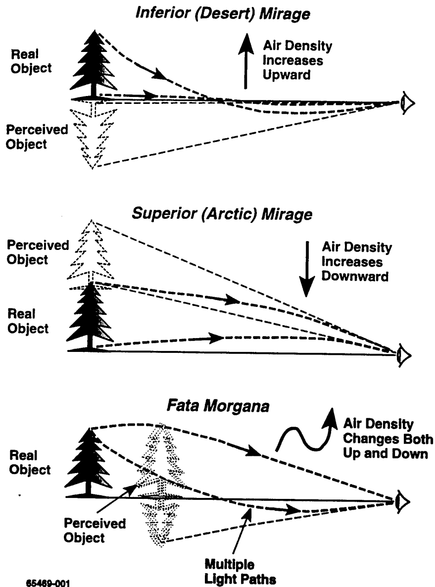
Figure 3. How Mirages Are Produced (from Davis, 1982)
