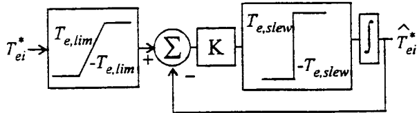
Figure 7. Torque limiter.
