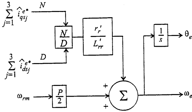
Figure 10. Field oriented controller.
