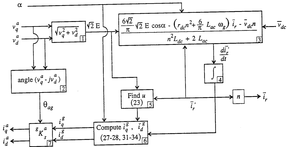
Figure 11. Diagram of rectifier model for 12-pulse power supply.
