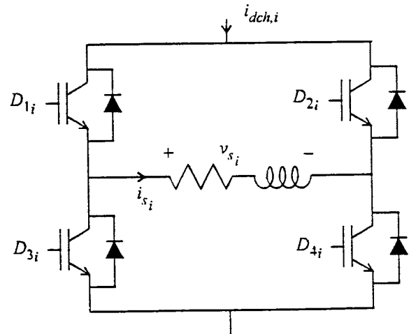
Figure 3. H-bridge.
