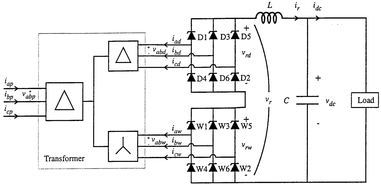
Figure 6. Power supply.
