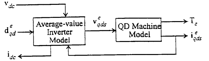
Figure 7. Average-value simulation structure..
