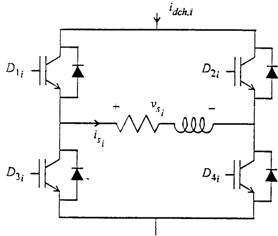
Figure 2. H-bridge.
