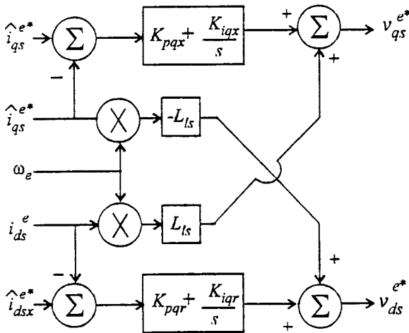
Figure 11. QD set current control.
