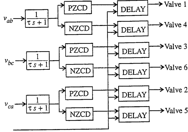
Figure 16. Gate sequencer.
