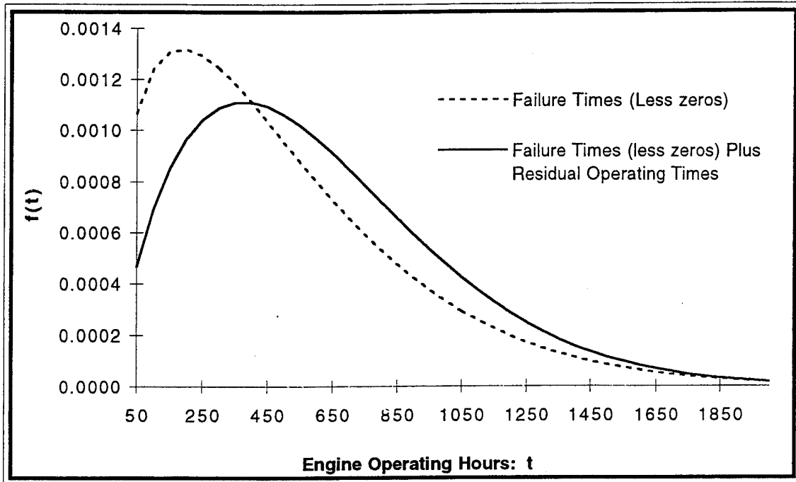
Figure 2-1. Weibull Distribution PDF Comparison
