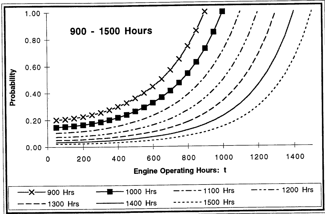
Figure 2-5. Conditional Probabilities With Residual Operating Times
