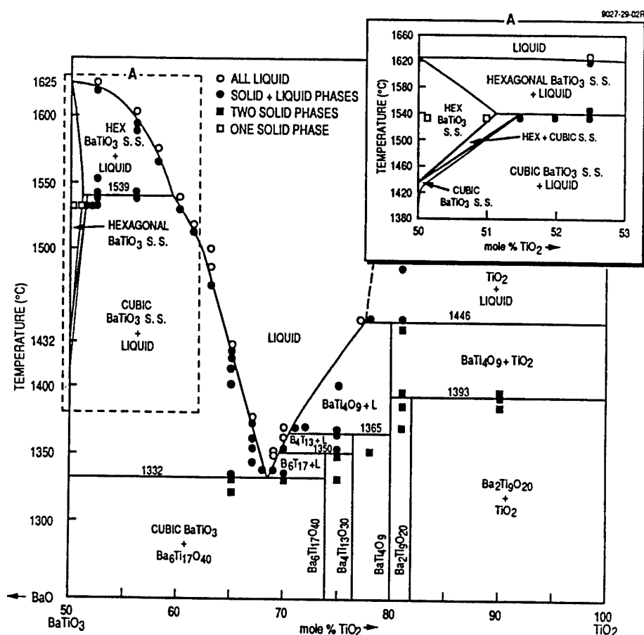
Figure 9-6. Phase diagram for the system BaTiO 3 -TiO 2 . From Kirby and Wechsler (1991) © 1991. Reprinted by permission of the American Ceramic Society.
