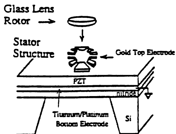
Fig.18 Ultrasonic micro-motor.
