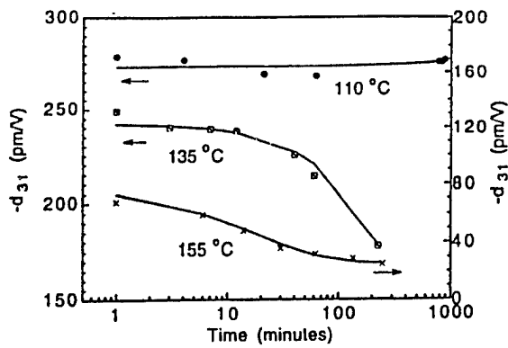
FIG. 4. The aging of d_{31} for 0.7PMN-0.3PT doped with 1% La as a function of temperature. The dc bias field is 5 kV/cm. The solid curves for 135 and 155 °C data are the fitting with Eq. (3) and for 110 °C is drawn to guide the eye. The data show that the relaxation time \tau decreases with temperature.
