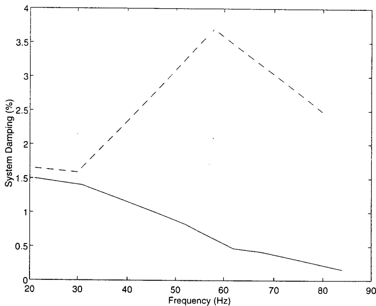
Figure 5.12. Percent Damping as a Function of Frequency.
