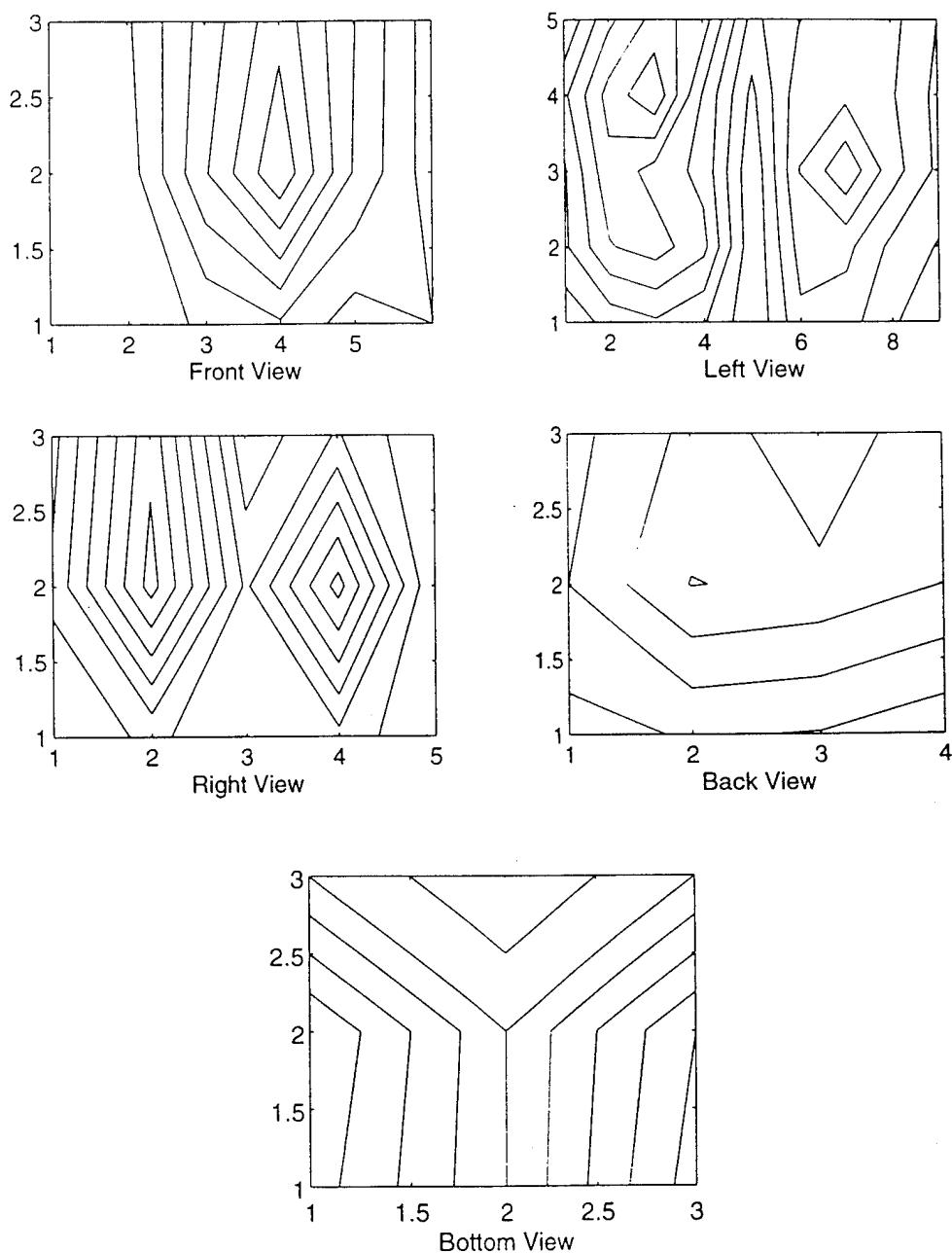
Figure 5.8. Experimental Mode Shape: 84 Hz.
