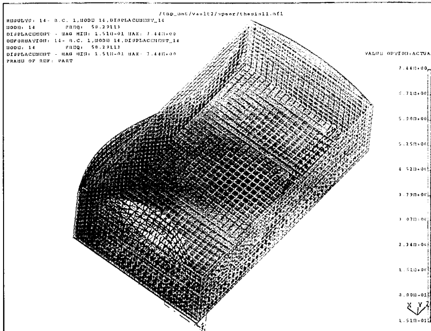
Figure 3.10. 58.29 Hz Mode Shape.
