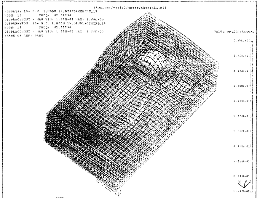
Figure 3.11. 62.02 Hz Mode Shape.
