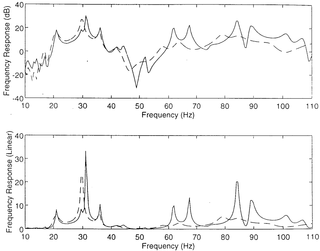
Figure 5.13. Frequency Response: Point E [Left side; (0, 6,24)]. ( top : dB scale : bottom : Linear scale)
