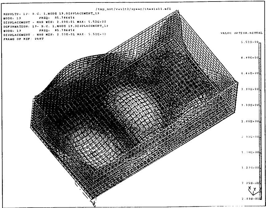
Figure 3.15. 85.78 Hz Mode Shape.
