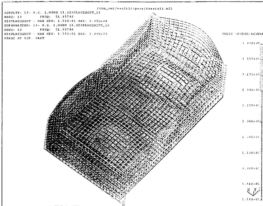
Figure 3.9. 51.35 Hz Mode Shape.
