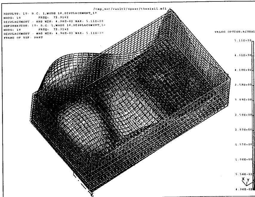
Figure 3.14. 72.91 Hz Mode Shape.
