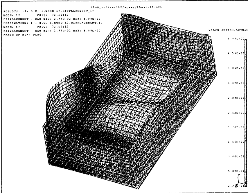
Figure 3.13. 72.46 Hz Mode Shape.
