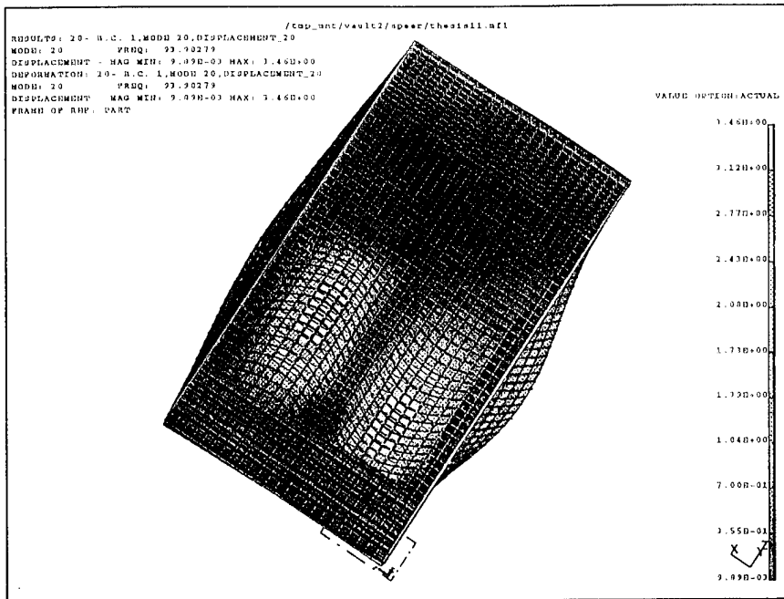
Figure 3.16. 93.9 Hz Mode Shape.
