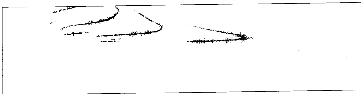
Figure 2.7: Ionogram 3 — hand filtered.
