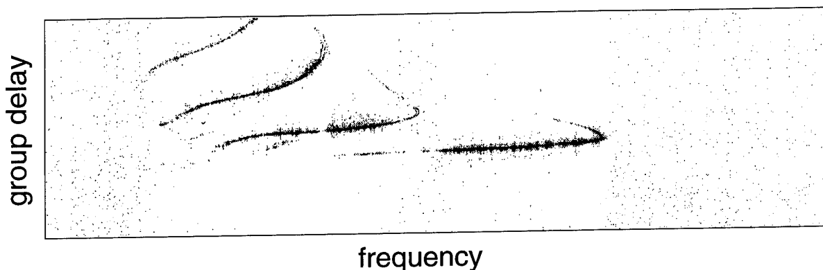
Figure 1.2: An example of an oblique ionogram.
