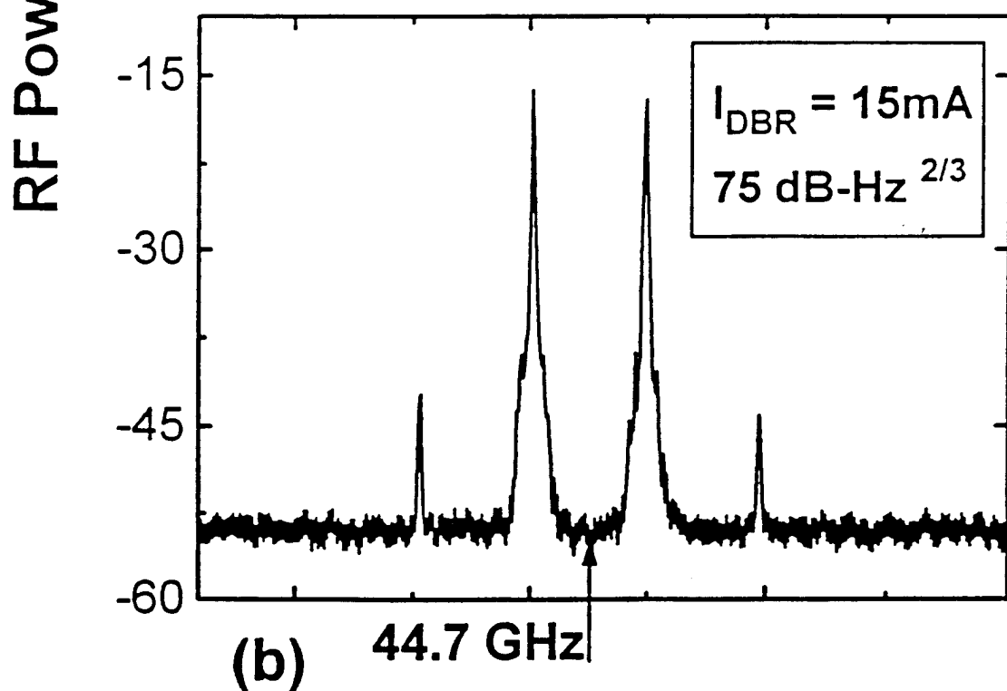
Figure 6. (a) Measured two-tone dynamic range for a modulation efficiency of (a) 0dB at 41GHz. The scale for the inset is 5dB/div. (b) Two-tone plot for a spur-free dynamic range of 75\text{dB} - \text{Hz}^{2/3} of a 3-section DBR laser described in Ref. [21].
