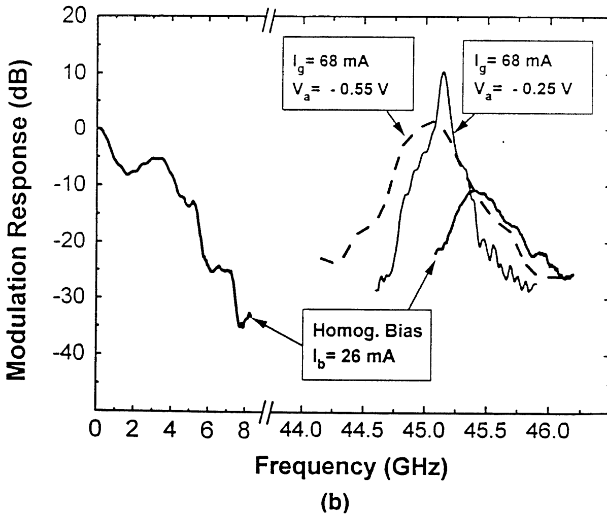
Figure 1. (a) Monolithic semiconductor laser of cavity length L . Modulation is applied to only a part of the laser cavity. (b) Measured low and high-frequency modulation response of the monolithic semiconductor laser in (a) at a cavity round-trip frequency of 45GHz.
