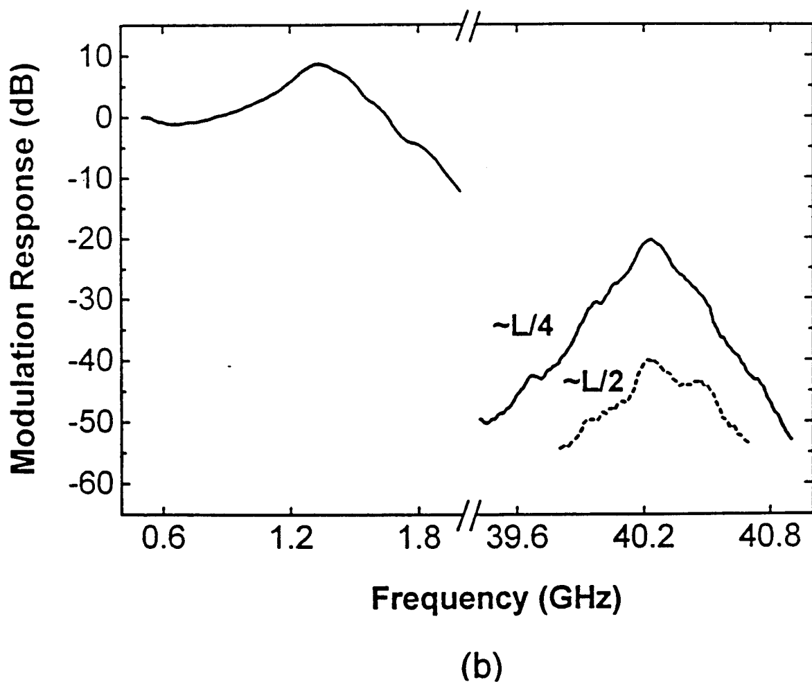
Figure 8. Illustration of the principle of resonant modulation and mode-locking of a single-contact monolithic semiconductor laser. (a) The microwave propagation loss of the applied modulation current at the round-trip cavity frequency results in partial cavity modulation and eliminates the need for a second contact. (b) Measured modulation response in the low and high frequency range when the modulation feed is positioned at L/4 and L/2 along the laser contact.
