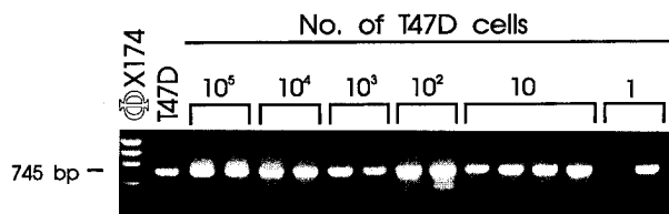
Fig 2. Sensitivity of the K19 RT-PCR assay. Molecular-weight marker is a Hae III digest of \phi X174. The number of T47D breast carcinoma cells mixed with 1 million normal PBMC cells is shown. Analyses at 10^5 , 10^4 , 10^3 , and 10^2 T47D cells were performed in duplicate and at 10 cells in quadruplicate.
