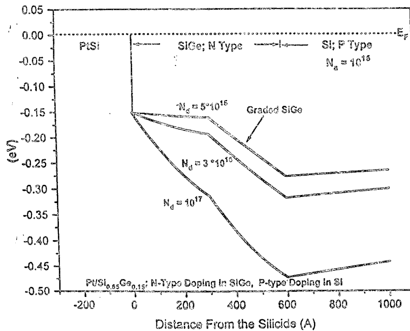
Figure 17: Band diagram at zero bias for a structure similar to that of Fig. 14, with p-type doping of 1 \times 10^{15} \text{ cm}^{-3} below 60 nm from the surface, but with n-type doping in the top 60 nm. Note the total barrier face by holes at zero bias exceeds 250 meV.
