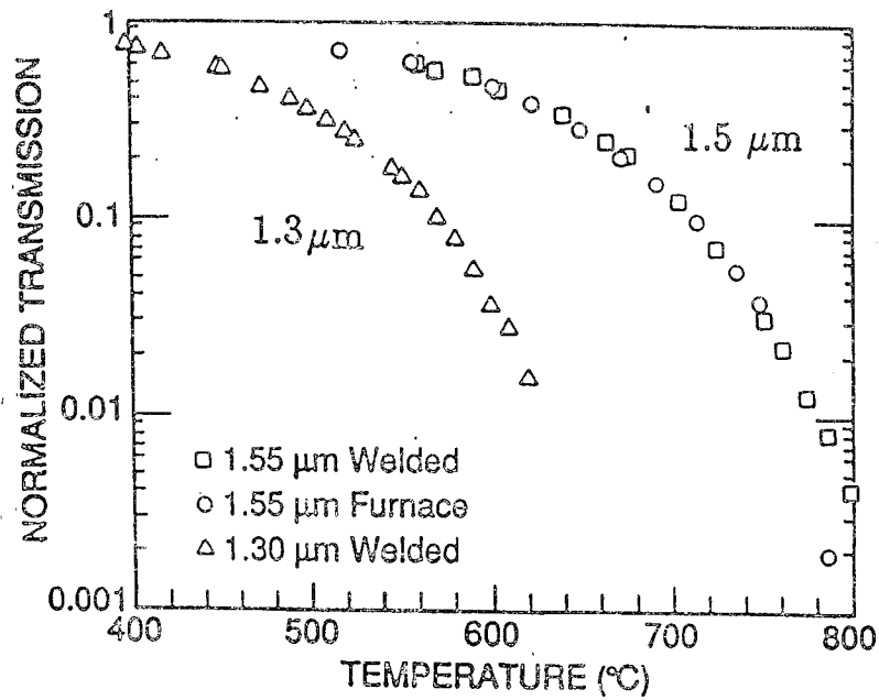
Figure 6: Normalized transmission vs. temperature for 1.3 \mu m and 1.55 \mu m radiation for a 500- \mu m thick lightly doped silicon wafer.
