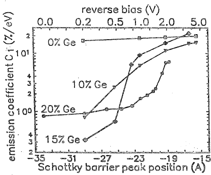
Figure 13: Dependence of barrier height and emission coefficient ( C_1 ) extracted from Fowler plots for various final Ge fractions.
