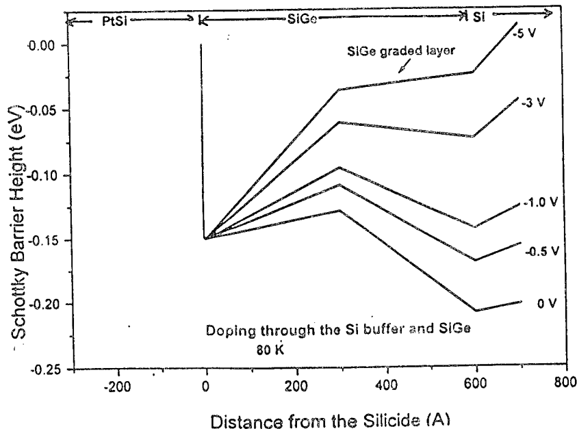
Figure 15: Band diagram at several reverse biases for the structure of Fig. 14 with a doping of 1 \times 10^{15} \text{cm}^{-3} . Note the reduction of the total barrier faced by a hole from the PtSi.
