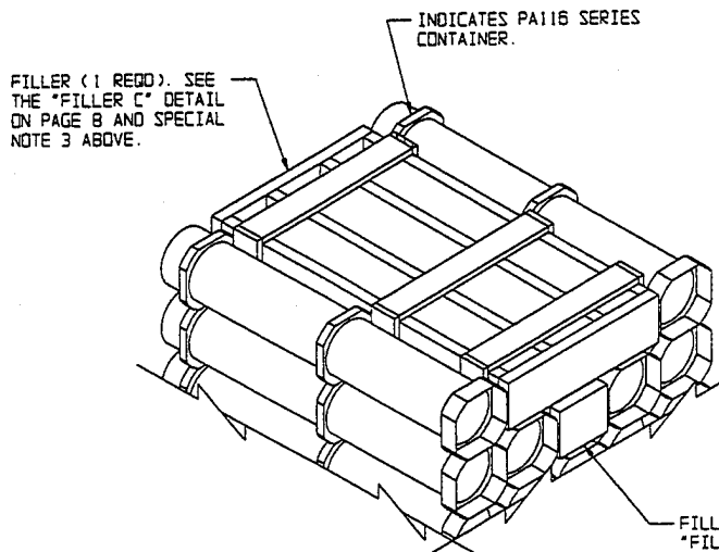
DETAIL C
