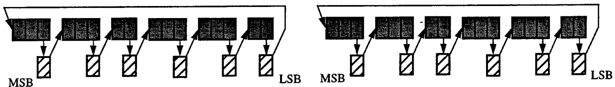
FIGURE 6. Toroidal-pipelined ones-complement adders
