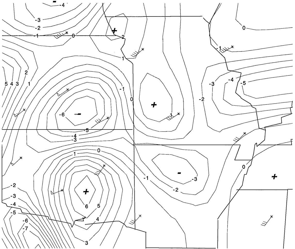
Figure 4.7: 600 mb vorticity ( 10^{-5} \text{ s}^{-1} ) chart for 0800 UTC 8 June 1993.
