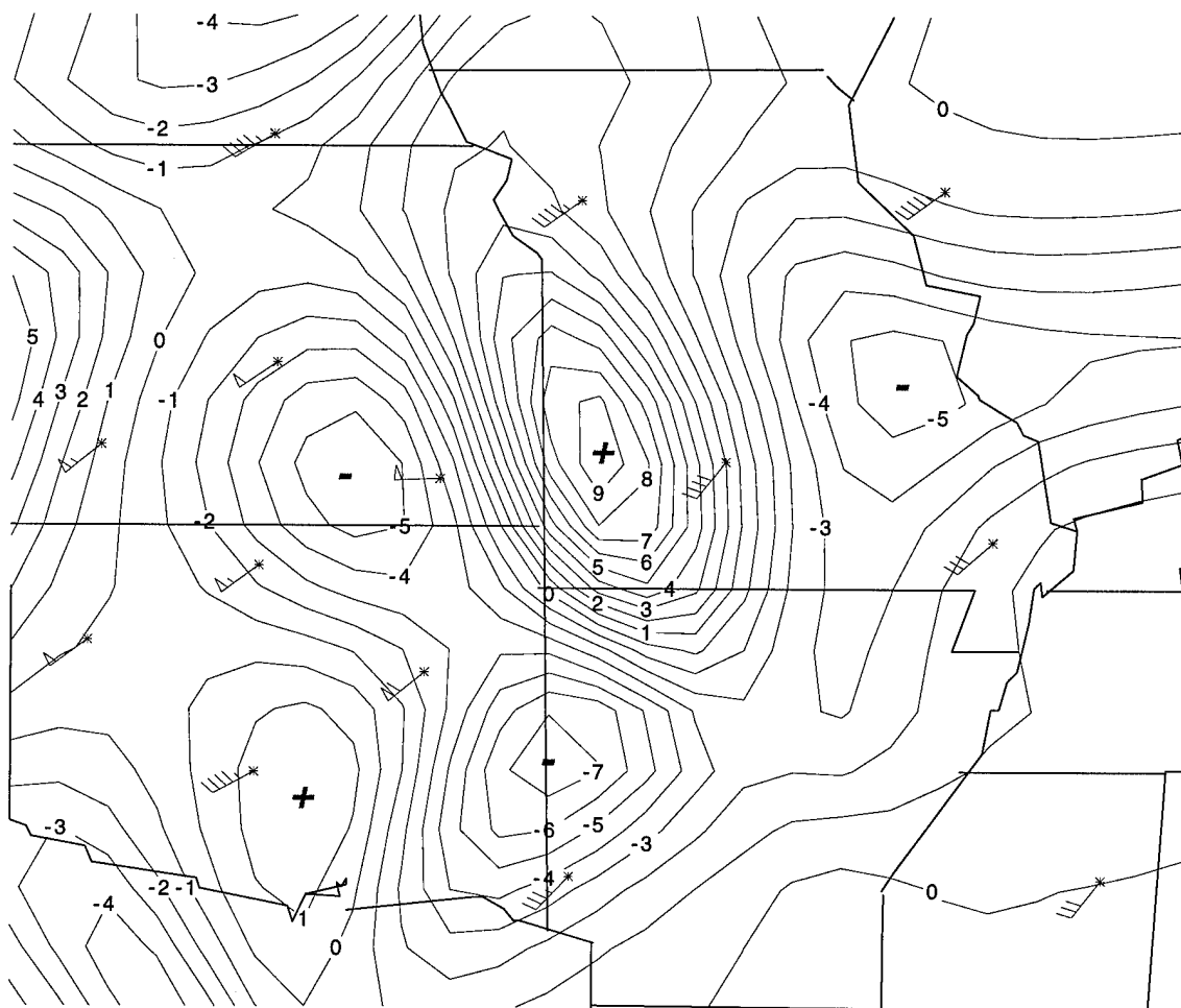
Figure 4.8: 600 mb vorticity ( 10^{-5} \text{ s}^{-1} ) chart for 0900 UTC 8 June 1993.
