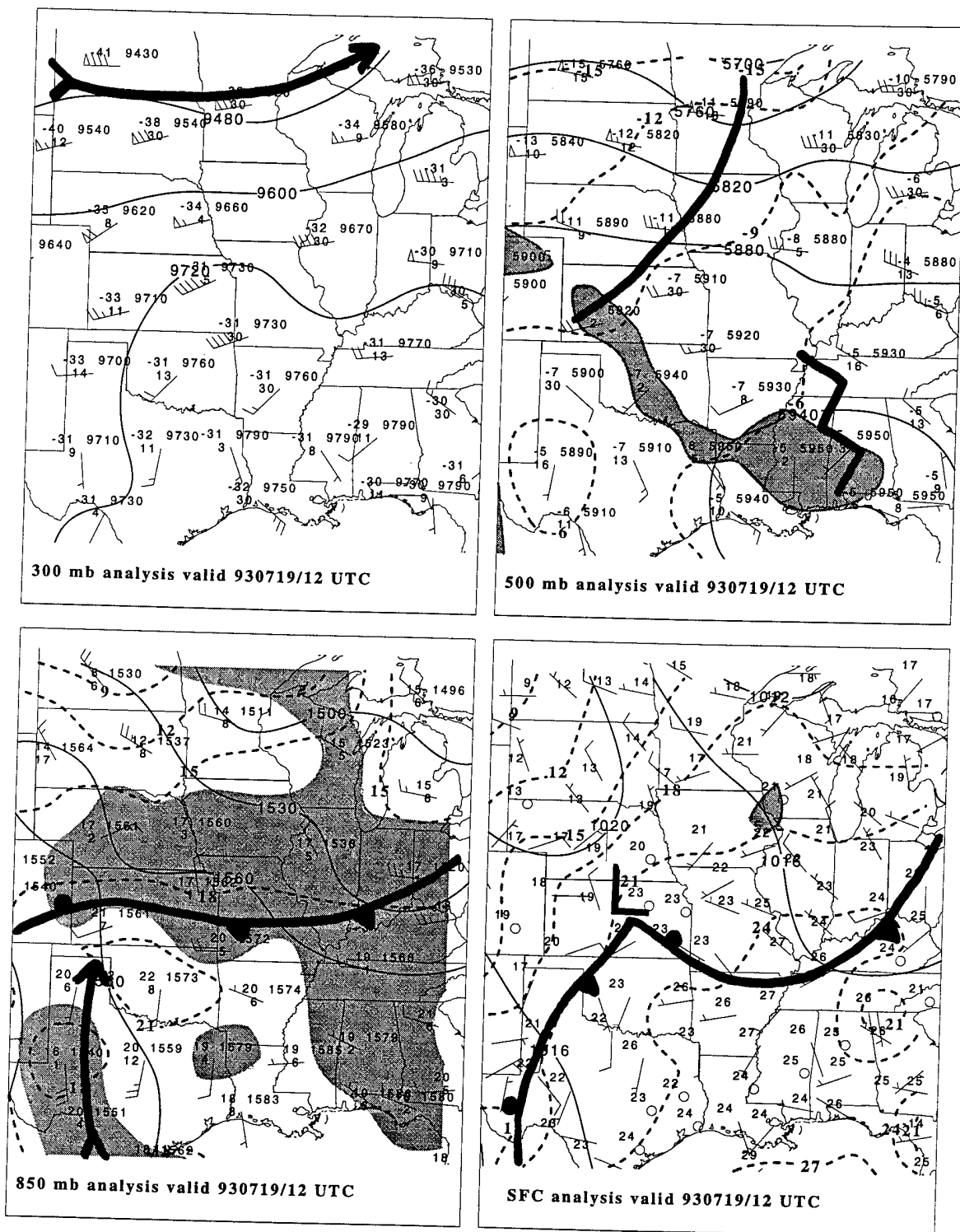
Figure 4.29: Analysis for 300 mb, 500 mb, 850 mb and surface levels at 1200 UTC 19 July 1993. The gray shaded regions are areas of dewpoint depressions of 5°C or less.
