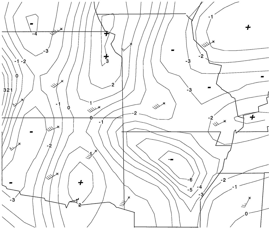
Figure 4.5: 600 mb vorticity ( 10^{-5}\text{s}^{-1} ) chart for 0600 UTC 8 June 1993.
