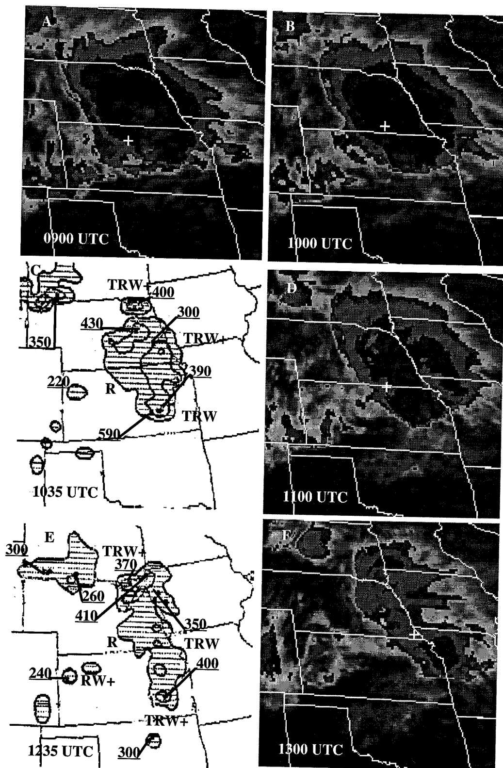
Figure 4.42: Infrared satellite images for (A) 0900 UTC, (B) 1000 UTC, (D) 1100 UTC, (F) 1300 UTC 13 August 1993; NWS radar summaries for (C) 1035 UTC and (E) 1235 UTC 13 August 1993.
