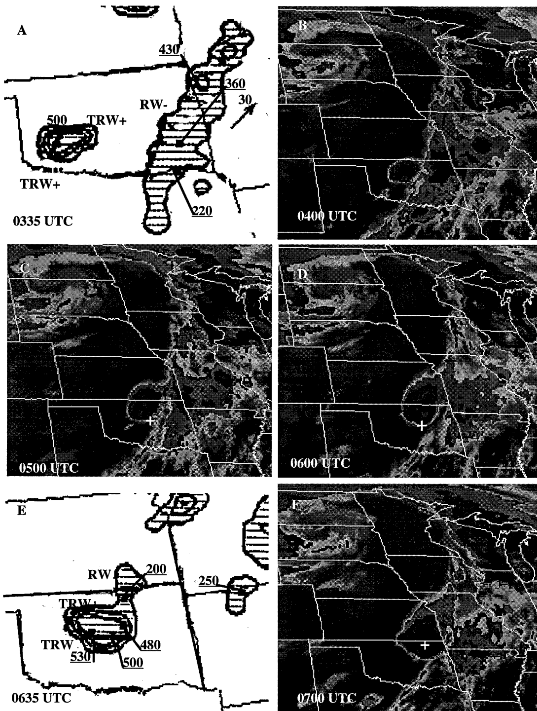
Figure 4.2: NWS radar summaries for (A) 0335 UTC and (E) 0635 UTC and infrared satellite images for (B) 0400 UTC, (C) 0500 UTC, (D) 0600 UTC and (F) 0700 UTC on 8 June, 1993.
