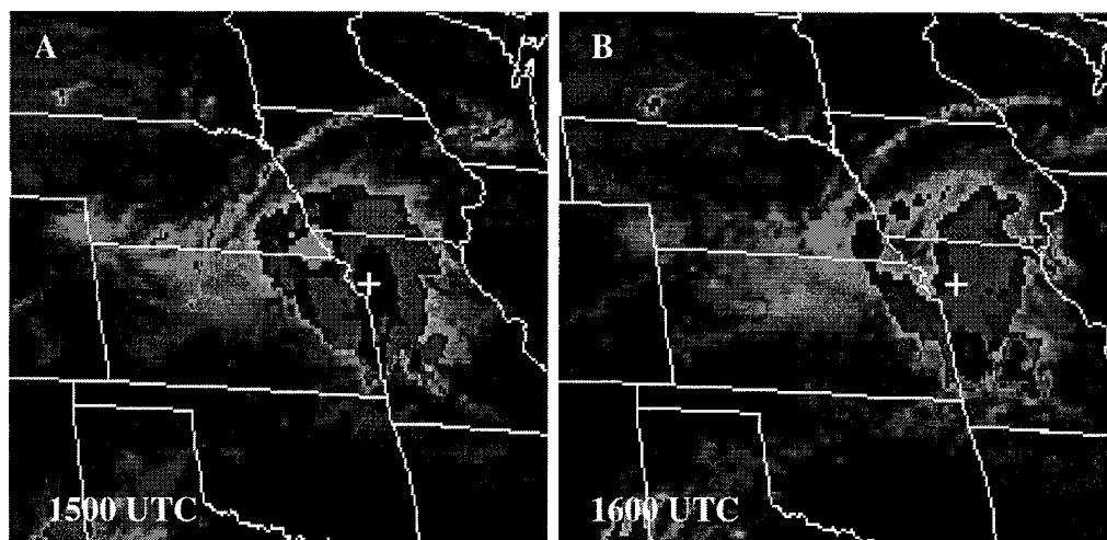
Figure 4.32: Infrared satellite images for (A) 1500 UTC and (B) 1600 UTC 19 July 1993.
