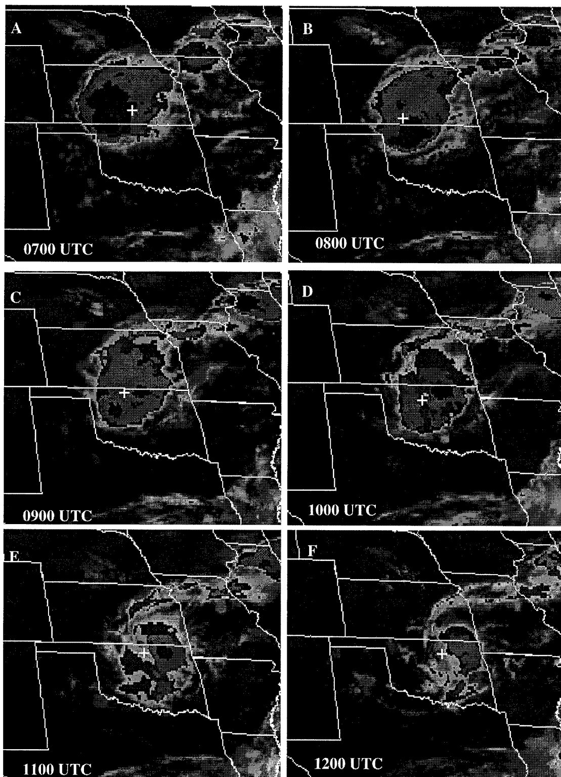
Figure 4.23: Infrared satellite images for (A) 0700 UTC, (B) 0800 UTC, (C) 0900 UTC, (D) 1000 UTC, (E) 1100 UTC and (F) 1200 UTC 27 June 1993.
