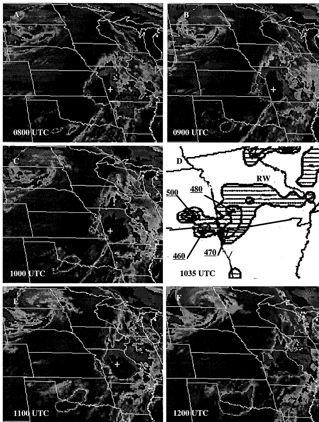
Figure 4.3: NWS radar summary for (D) 1035 UTC and infrared satellite images for (A) 0800 UTC, (B) 0900 UTC, (C) 1000 UTC, (E) 1100 UTC and (F) 1200 UTC on 8 June, 1993.
