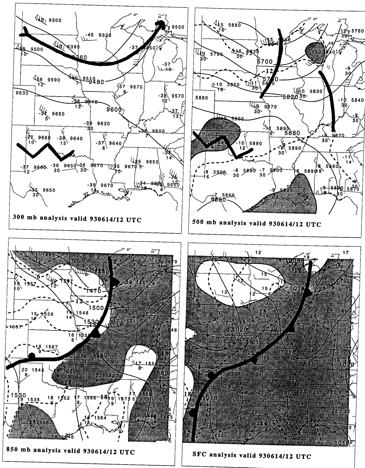
Figure 4.16: Analysis for the 300 mb, 500 mb, 850 mb and surface levels for 1200 UTC 14 June 1993. The gray shaded regions are areas of dewpoint depressions of 5°C or less.
