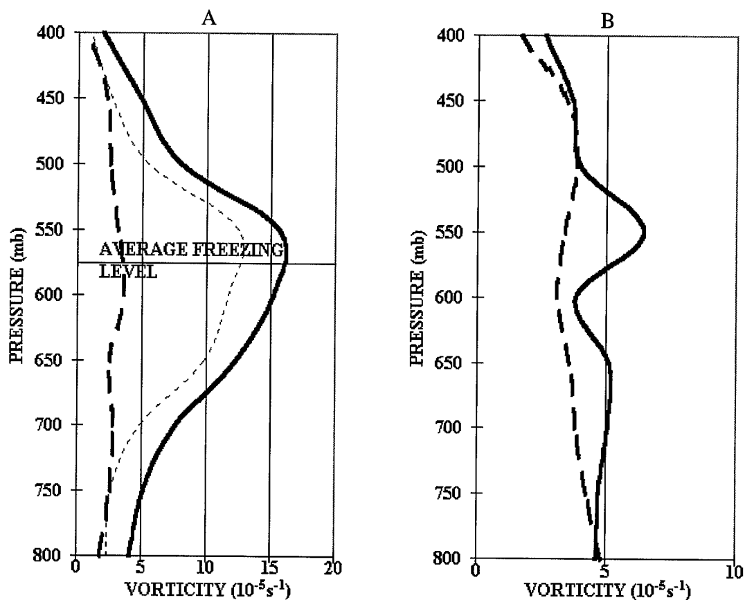
Figure 4.49: (A) Average vertical profiles of relative vorticity for the nine MCSs studied and (B) standard deviation. The long dashed line is for the beginning stage of the MCS and the solid line is for the maximum stage while the thin dashed line in A is the average increase of the relative vorticity.
