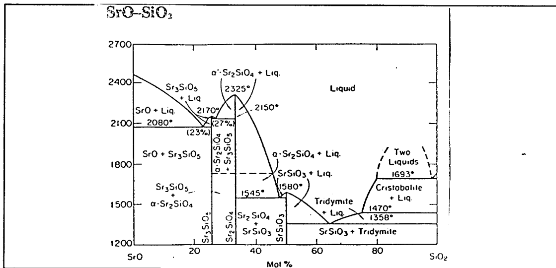
Fig. 38 \text{SiO}_2 -SrO Equilibrium Phase Diagram (24)
