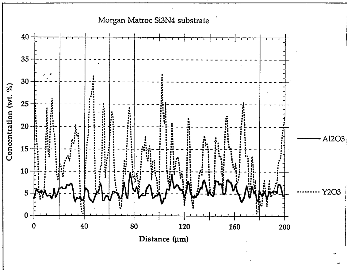
Fig. 6 Electron microprobe analysis of \text{Si}_3\text{N}_4 grain boundary composition. Microprobe scan taken in the bulk \text{Si}_3\text{N}_4 outside the diffusion zone in wetted \text{Si}_3\text{N}_4 ; distance starting point is arbitrary.
