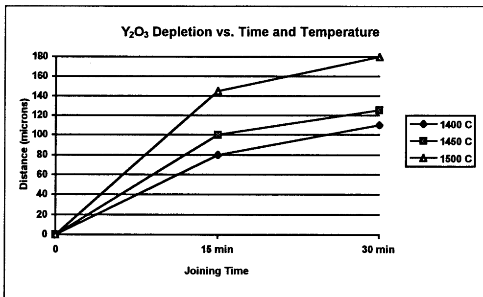
Fig. 44 Y 2 O 3 Depletion in SAS-10 Wetting of Si 3 N 4 vs. Time and Temperature [data presented at 0 min (0 distance) are inferred and do not reflect actual measurements]
