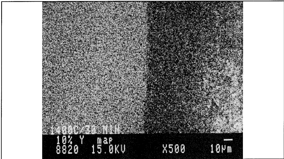
Fig. 35 10% Y Distribution Micrograph for SAS-5 Glass Wetting Si 3 N 4 at 1400 °C for 30 min (magnification: 500x) [glass is left of substrate]
