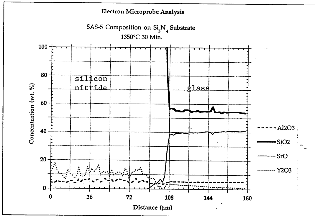
Fig. 17 Electron Microprobe for SAS-5 Wetting \text{Si}_3\text{N}_4 : 1350 °C / 30 min
