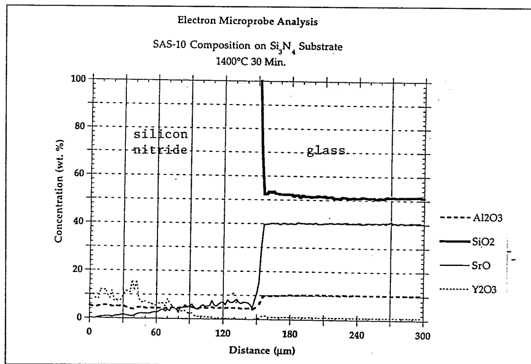
Fig. 25 Electron Microprobe for SAS-10 Wetting \text{Si}_3\text{N}_4 : 1400 °C / 30 min
