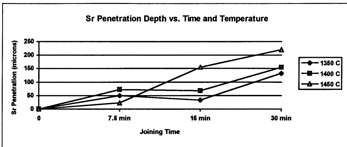
Fig. 41 Maximum Sr Penetration Depth vs. Joining Temperature and Time for SAS-5 Wetted Si 3 N 4 [data presented at 0 min (0 penetration) are inferred and do not reflect actual measurements]
