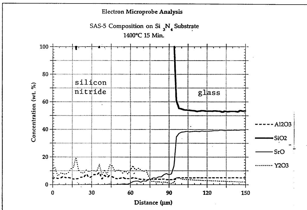
Fig. 19 Electron Microprobe for SAS-5 Wetting \text{Si}_3\text{N}_4 : 1400 °C / 15 min
