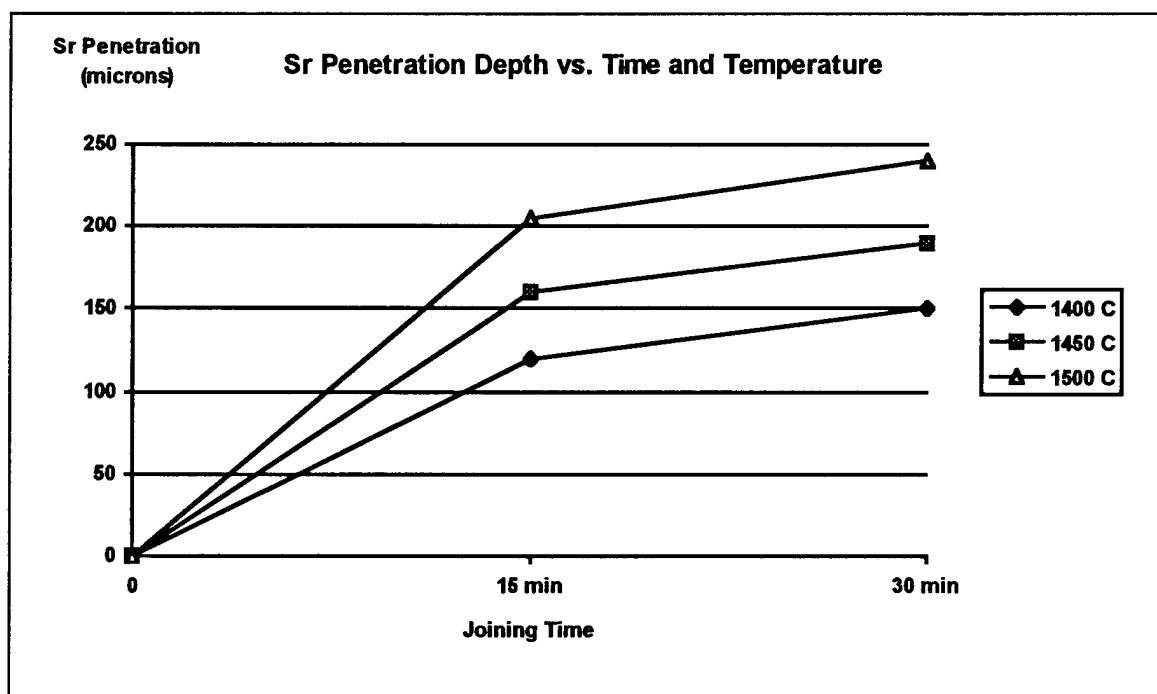
Fig. 42 Maximum Sr Penetration Depth vs. Joining Temperature and Time for SAS-10 Wetted Si 3 N 4 [data presented at 0 min (0 penetration) are inferred and do not reflect actual measurements]
