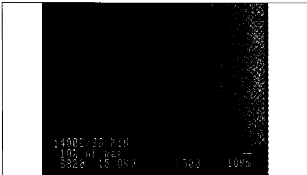
Fig. 37 10% Al Distribution Micrograph for SAS-5 Glass Wetting \text{Si}_3\text{N}_4 at 1400 °C for 30 min (magnification: 500x) [glass is left of substrate]
