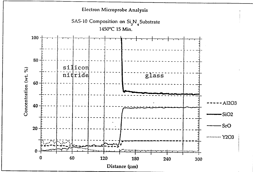
Fig. 26 Electron Microprobe for SAS-10 Wetting \text{Si}_3\text{N}_4 : 1450 °C / 15 min
