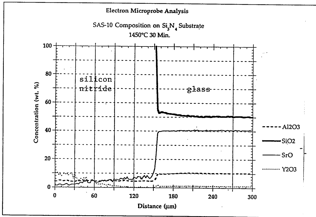
Fig. 27 Electron Microprobe for SAS-10 Wetting \text{Si}_3\text{N}_4 : 1450 °C / 30 min
