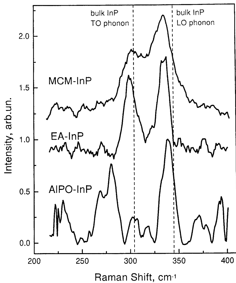
Figure 2 Raman spectra of InP filled dielectric matrices
