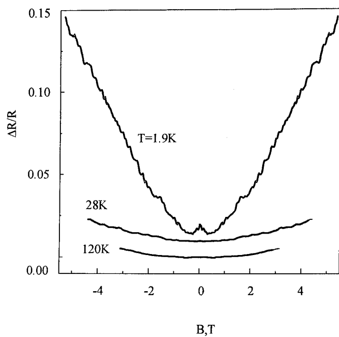
Fig.1a O-InSb: Magnetoresistance curves at T=120, 28 and 1.9K.
