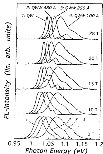
FIG. 2. Magneto-luminescence spectra of n-type modulation doped and lattice mismatched \text{InAsP}_{1-x}/\text{InP} quantum well wires (480, 250 and 100 Å wide) and the quantum well reference.
