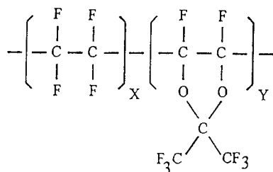
Figure 1. The structure of AF 1600, x:y = 1:2
