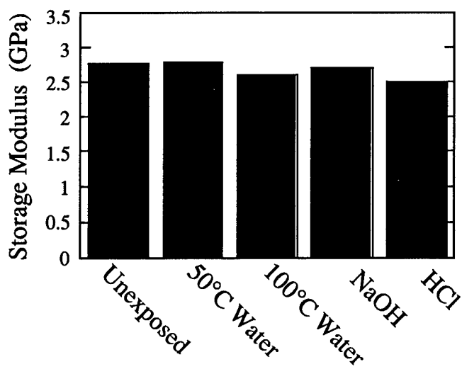
Figure 6. The storage modulus obtained using dynamic mechanical analysis for Epon 828 m-PDA cured epoxy resin as a function of exposure to aqueous environments. All samples were tested after achieving 95% or greater degree of saturation.
