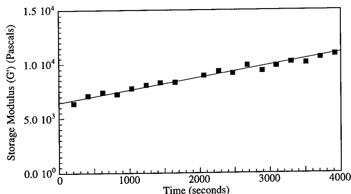
Figure 1. Variation in storage modulus with time at processing temperature. The sample used is 35% (vol) silica at a shear stress of 50 Pa and a frequency of 0.005 s -1 . The temperature is 200°C.
