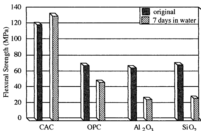
Fig. 1. Original flexural strength and residual strength after 7-day water immersion.
