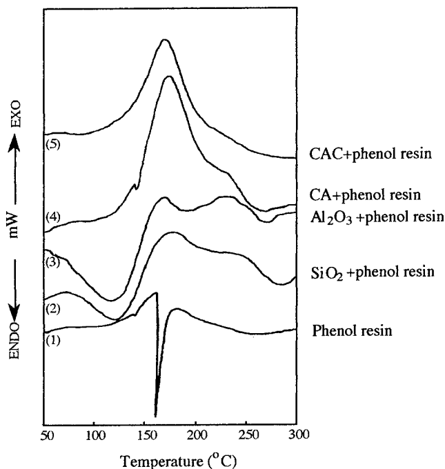
Fig. 2. DSC thermograms.
