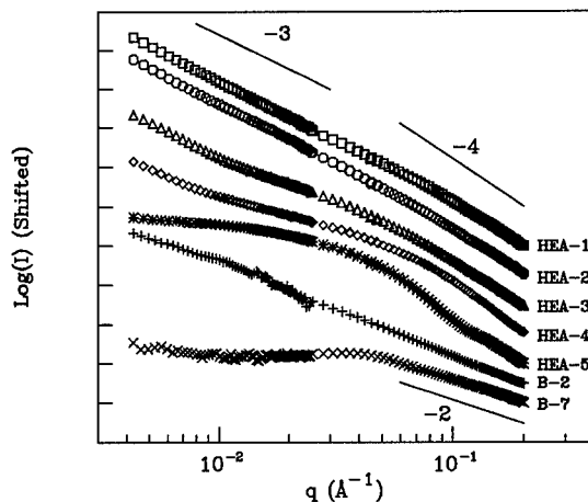
Figure 1. SANS and SAXS from PolyHEA/SiO 2 IPNs.
