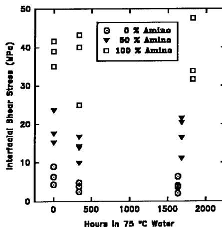
Figure 3 Interfacial shear stress vs. time in 75 °C distilled water.
