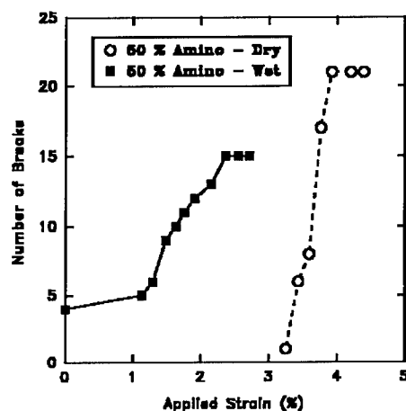
Figure 2 Number of breaks vs. applied strain for a dry and water conditioned sample.
