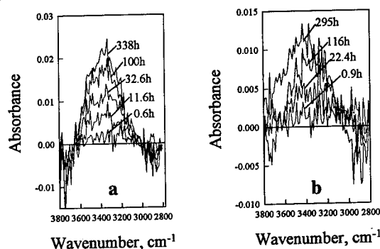
Figure 1. FTIR-MIR difference spectra of epoxy-coated untreated (a) and 0.1% silane-treated (b) \text{SiO}_2 -Si prisms exposed to 24°C water for several time intervals.
