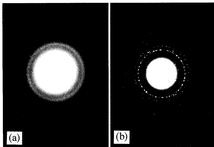
Figure 2. Electron diffraction patterns recorded from thin PTFE films deposited onto NaCl substrates heated to (a) 200°C and (b) 350°C. (Note: different camera constants were used for the two patterns.)
