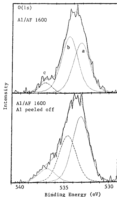
Figure 9. O(1s) spectra from a sample of 30 Å Al/AF 1600, top curve, and from a sample of Al/AF1600 with the Al peeled off, bottom curve.
