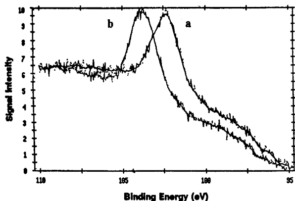
Figure 3. High resolution XPS spectra in the Si 2p region for PDMS samples before (a) and after ten minutes of UV/ozone exposure (b).
