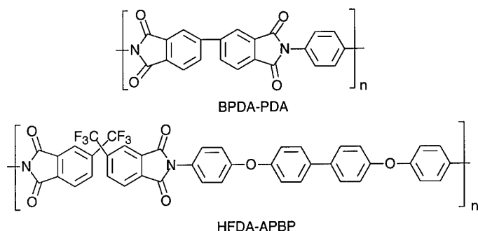
Figure 1. Structures of BPDA-PDA and HFDA-APBP.
