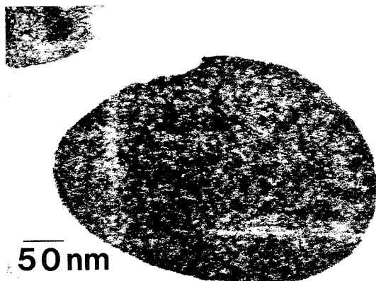
Figure 4 - HAADF STEM image of a \text{RuO}_4 -stained bulk epoxy section on a holey-C support film.
