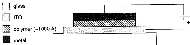
Figure 8. Typical polymeric light-emitting diode device structure.
