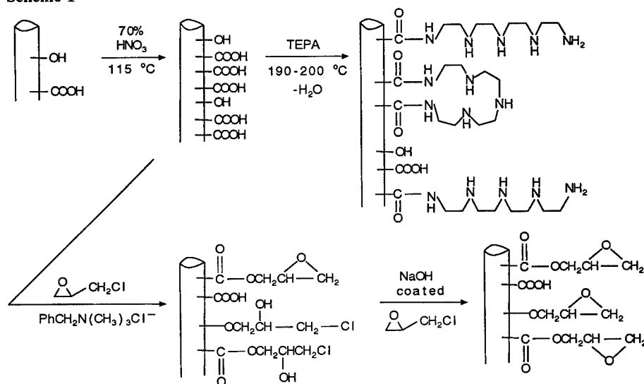
Scheme 1
