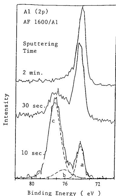
Figure 6. Al(2p) spectra from an AF 1600 film on Al sputtered for 10, 30, 120 sec.
