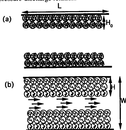
FIGURE 1: (A) The good-solvent planar brush microvalve. The planar polymer brushes, each of height H_0 , are grafted to opposing planes of length L , width Z , and separation W \ll Z . (B) When a good solvent flows across the planes, the brushes swell to a height H > H_0 . The flow penetrates the brushes only weakly so that the cross sectional area for flow is reduced. The brush swelling produces a closing of the flow area and a dramatic reduction in discharge results.
