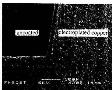
Fig. 1: SEM of PTFE surface electroplated with 20 \mu\text{m} copper after electroless deposition of copper.
