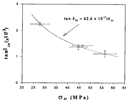
Figure 3. The relationship between \tan\delta_m and \sigma_{tr} . Error bars represent \pm 1 standard deviation.
