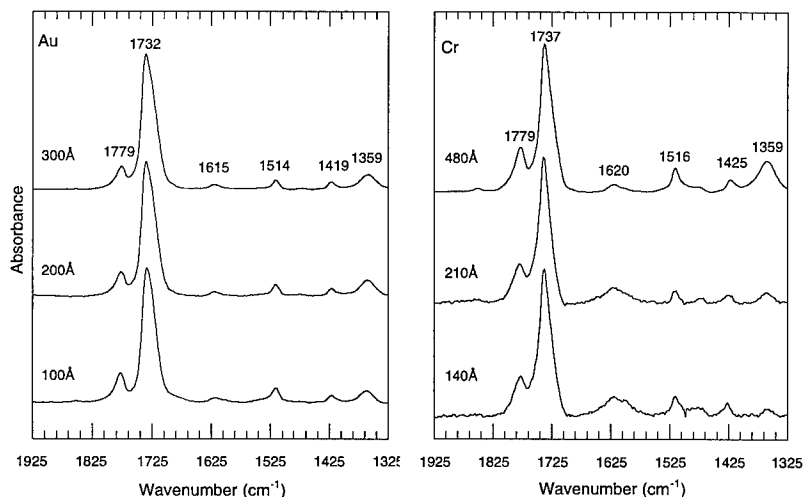
Figure 3. IRRAS spectra of BPDA-PDA on Au and \text{Cr/Cr}_x\text{O} as a function of polymer film thickness.
