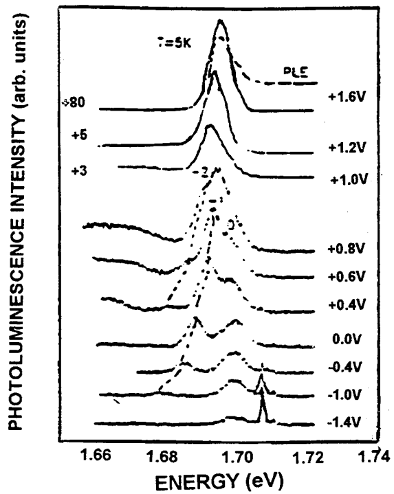
Figure 6 - Photoluminescence spectra
