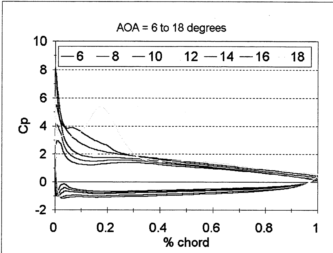
Figure 3.15 - Coefficient of Pressure Distributions for Elliptical Leading Edge Sail
