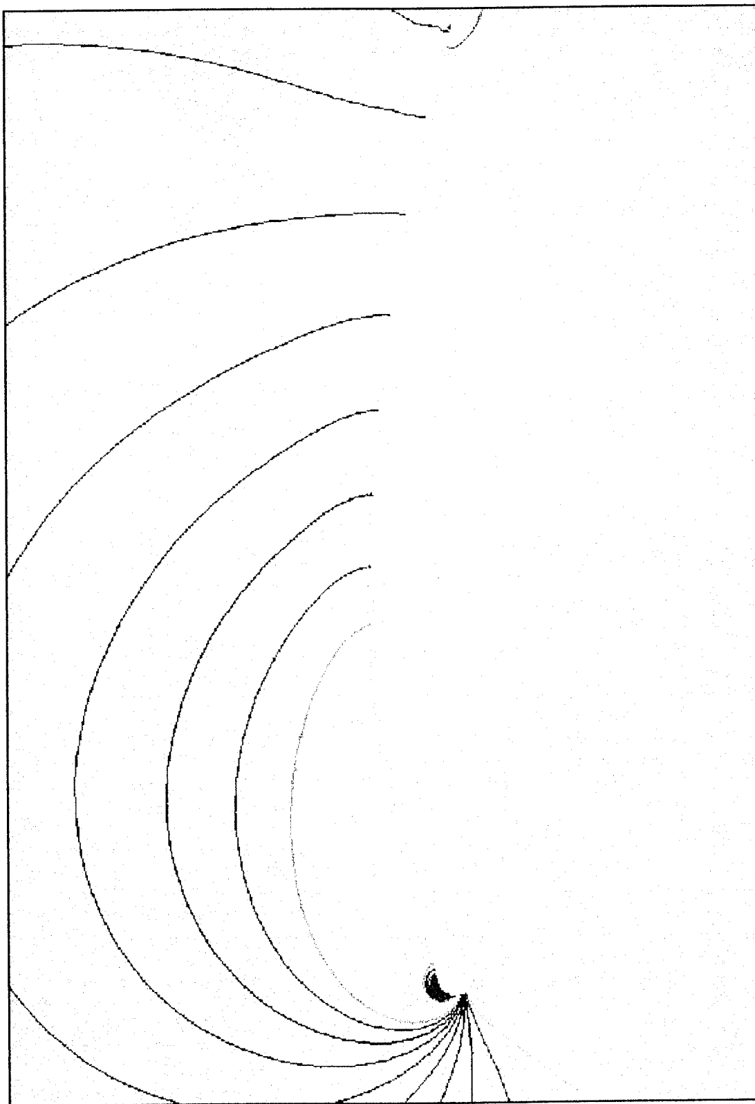
Figure 3.8 - Pressure Contour Plot for Reference Windsurfer Sail at 10° AOA.
