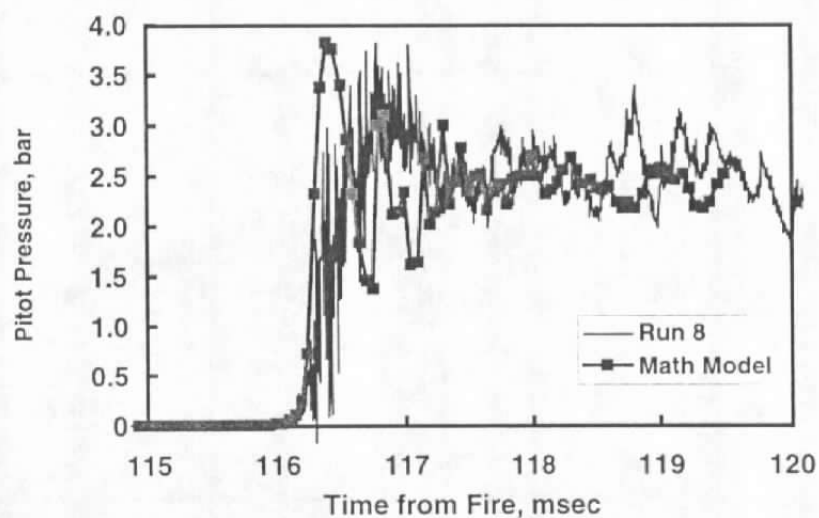
b. Run 8, Pressure Gage PT4
