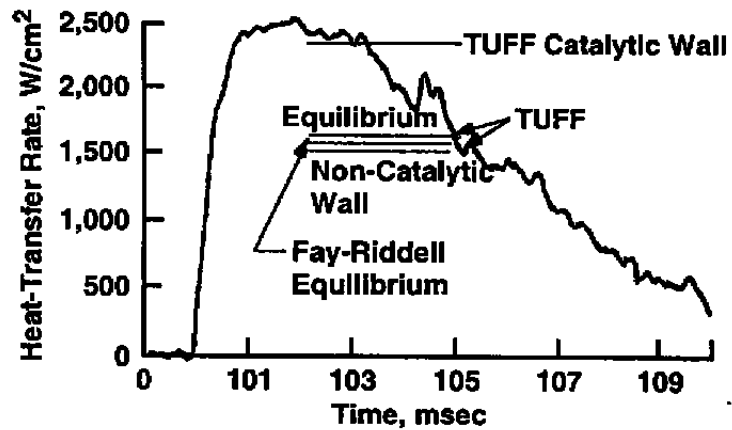
Figure 37. Comparison of computed stagnation point heat transfer with measurements, Run 13.
