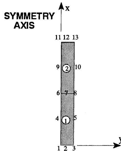
Figure 10. Axisymmetric FE Model (Element numbers are circled, node numbers are plain)
