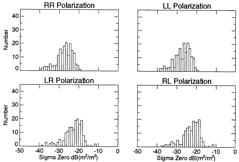
Figure 22. Sample low-resolution spatial histograms for Yuma clutter.
