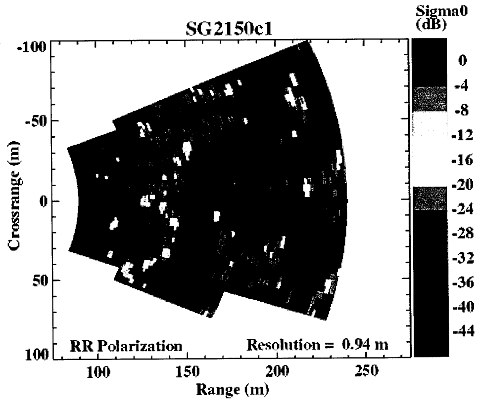
Figure 23. Sample high-range resolution RCS maps for RR and RL polarization for Grayling II.
