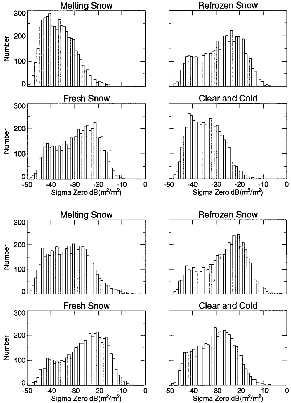
Figure 26. Sample high-resolution spatial histograms for RR polarization above and RL polarization below for Grayling II for different ground conditions.
