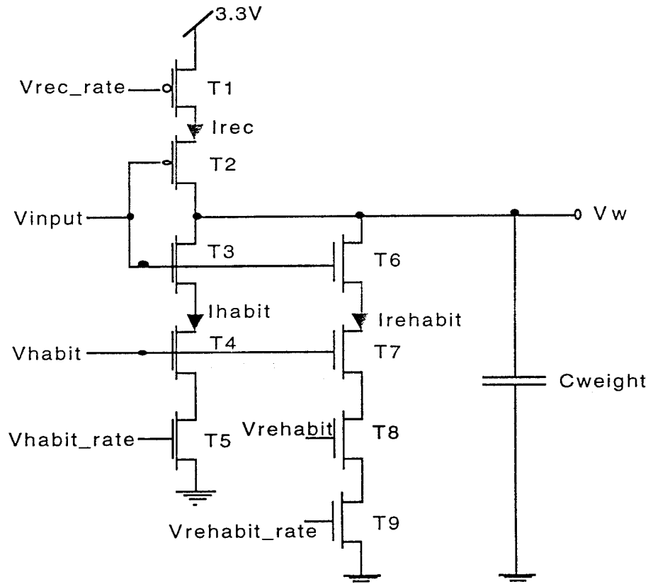
Fig. 2: Weight habituation, rehabituation and recovery circuit in one of the neurons.
