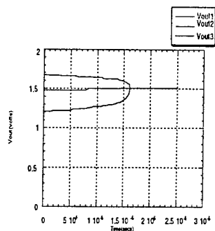
Figure 7. Output of MERAM network node as a function of time
