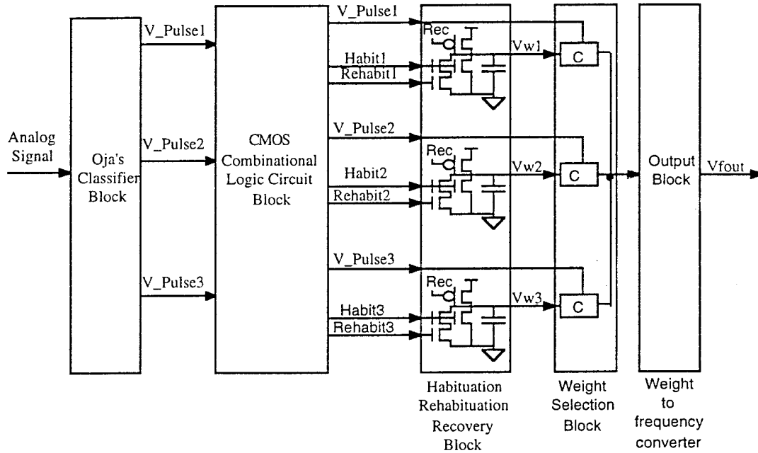
Fig. 1: Floorplan of habituation, rehabituation and recovery system
