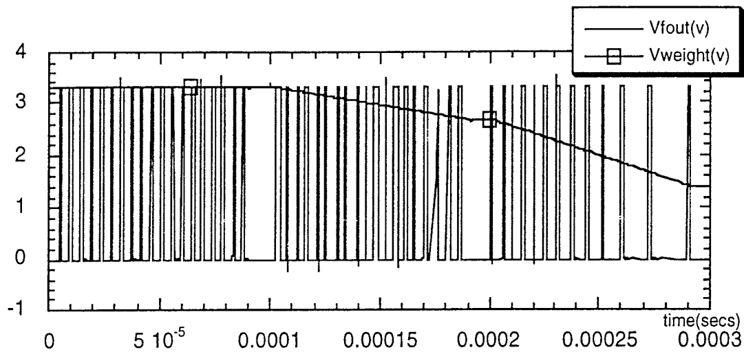
Fig. 4: Simulated output results from our chip showing habituation and rehabilitation.
