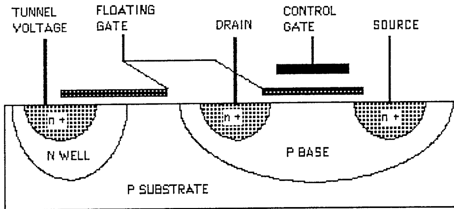
Figure 2. Crosssection of non-volatile memory cell. The cell contains p-base layer encompassing the source and drain gates. The four terminals of the cell are source, drain, control gate and tunneling gate
