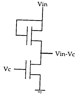
Figure 3. V_{in} - V_c circuit
