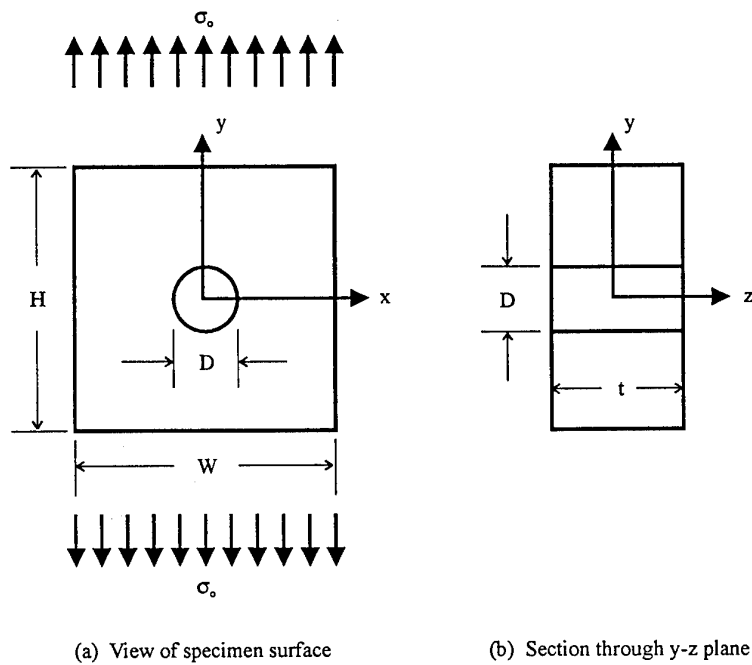
Figure 1. Axis and notation for circular hole in a plate
