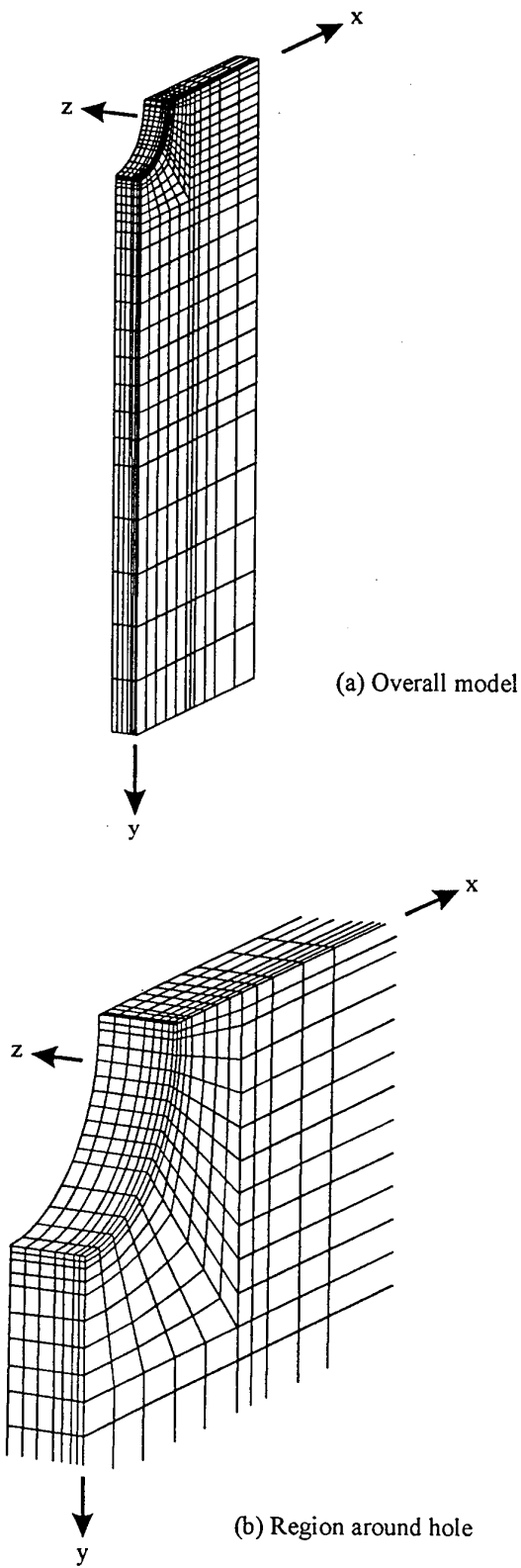
Figure 3. Finite element mesh for 10 mm thick specimen
