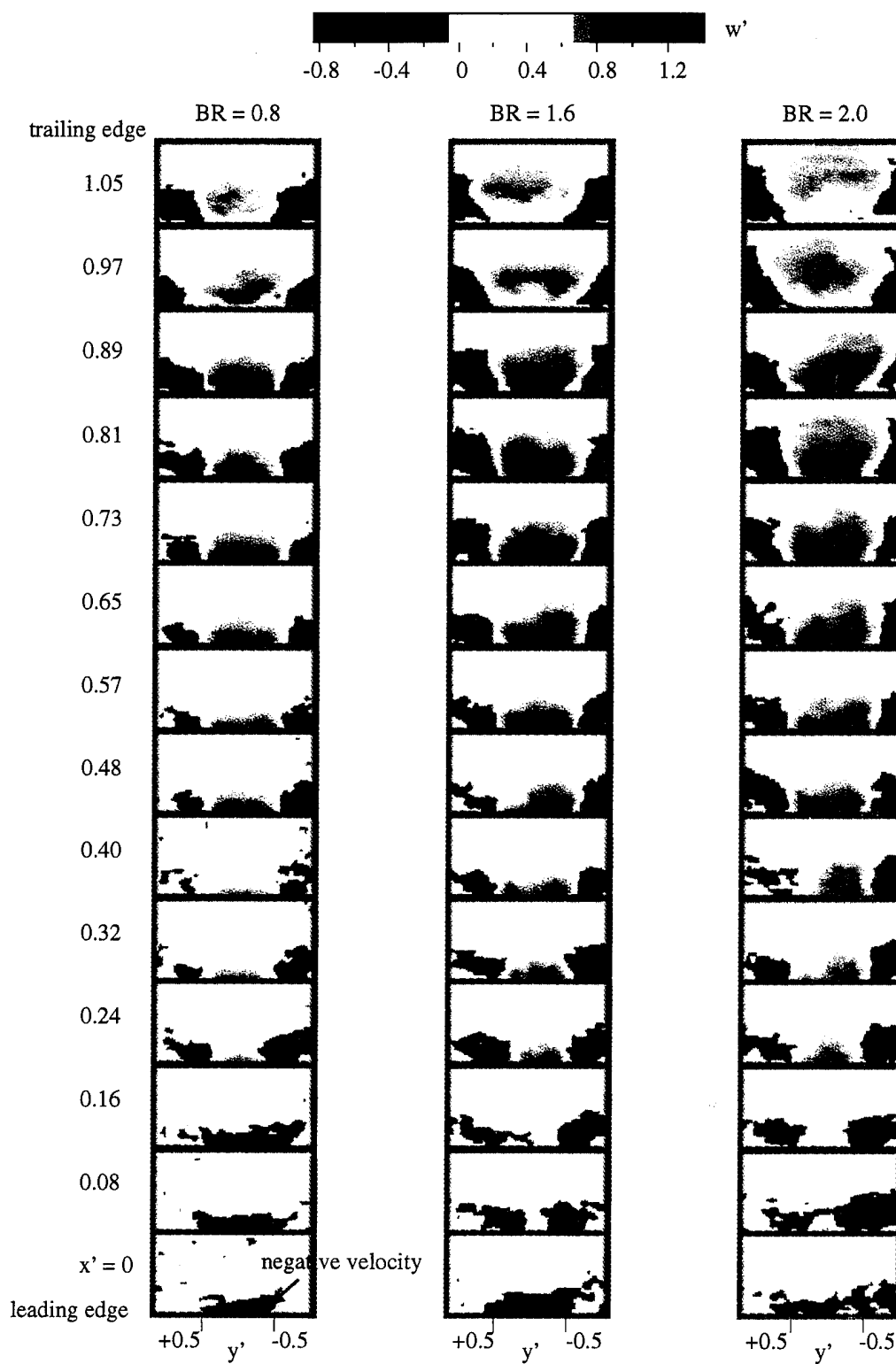
Figure 6-33: Hole 3: w' -Velocity Plots, BR = 0.8, 1.6, and 2.0
