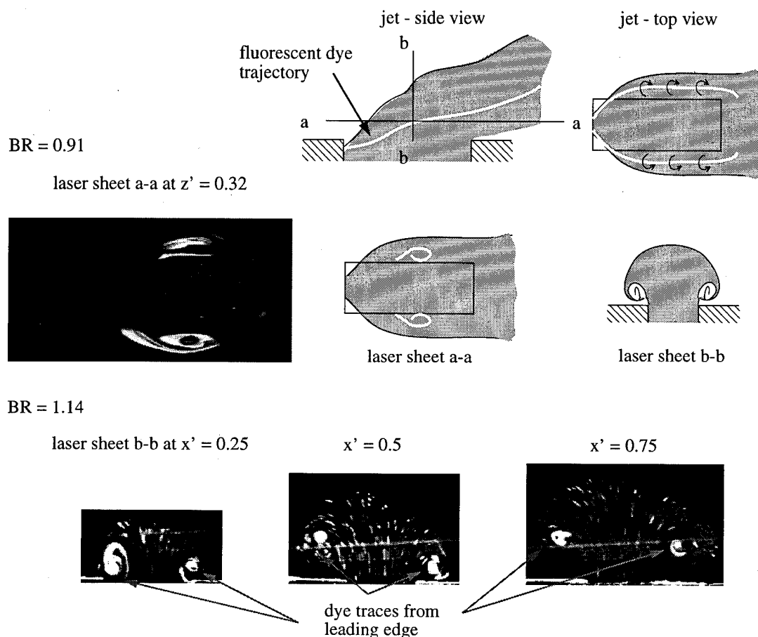
Figure 5-7: Combining of the Leading Edge and Side-wall Boundary Layers, Hole 1a
