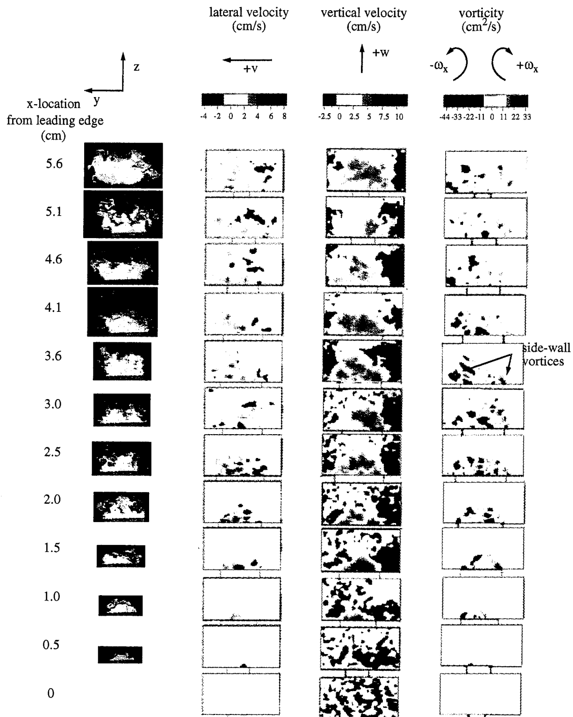
Figure 7-7: TP3: PIV Velocity and Vorticity Plots for Jet Cross-sections, BR_n = 1.0
