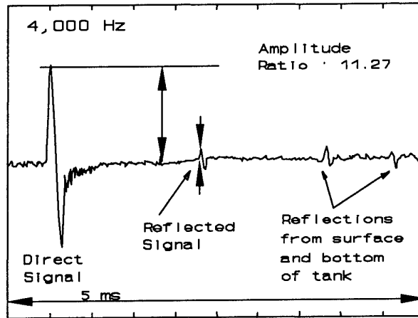
Figure 14: Hydrophone Output At 4kHz, MOD Salisbury Test Tank
