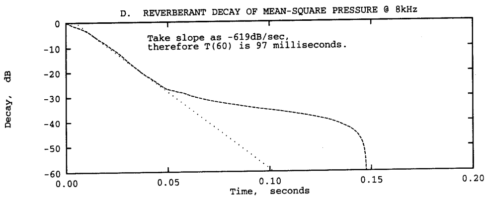
Figure 18: MOD Salisbury test tank reverberant decay curves integrated in time: (c) at source frequency 4 kHz, (d) 8 kHz. The measured decay curves are depicted by dashed lines. The dotted lines are an estimate of a uniform decay rate for use in the analysis.
