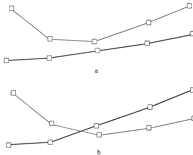
Fig 4.1: Non unique solution.
