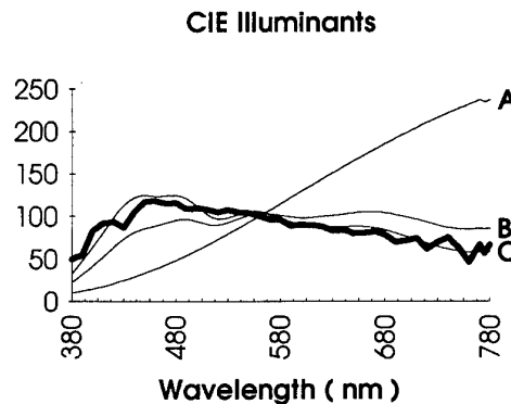
Figure A2. Relative power distributions of standard CIE Illuminants A, B, C and D65. The heavy line is Daylight (D65) which is used as the standard for all co-ordinate calculations in this paper.
