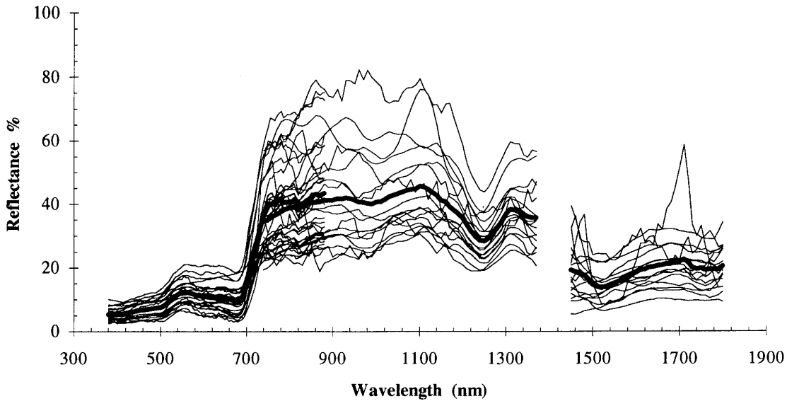
Figure 7.5 Measured reflectances of trees in the Townsville area, Qld, dry season, Oct 1983. The heavy line indicates the average reflectance.
