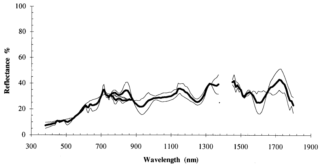
Figure 4.4 Measured reflectances of soils in the Tom Price area, WA, wet season, March 1983. The heavy line indicates the average reflectance.
