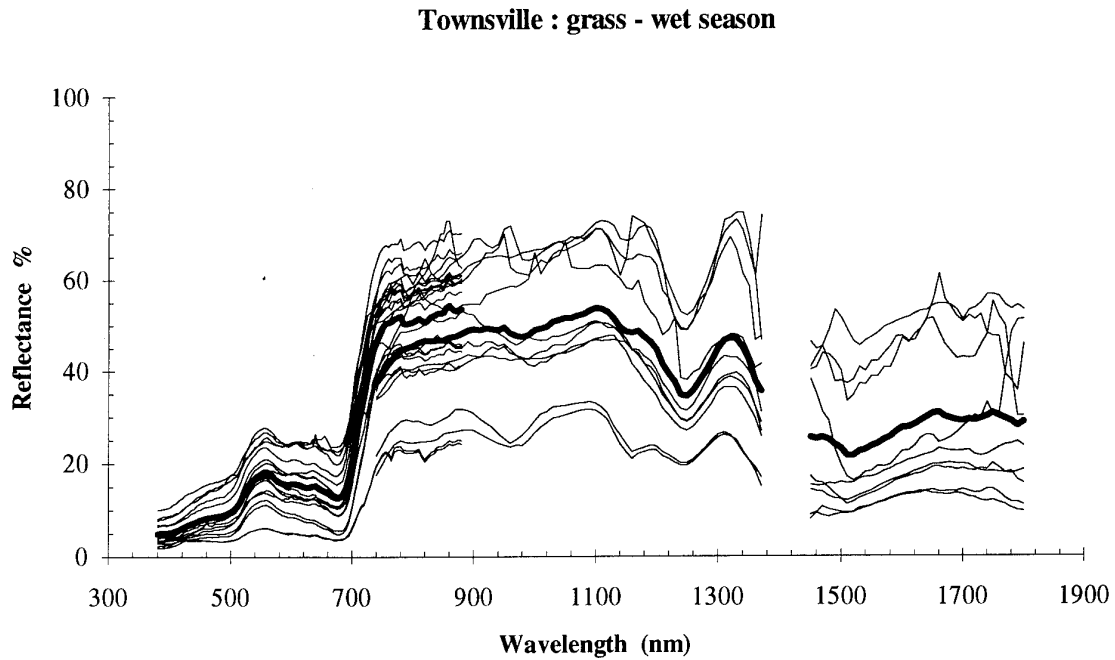
Figure 2.5 Measured reflectances of grasses in the Townsville area, Qld, wet season, April 1983. The heavy line indicates the average reflectance.
