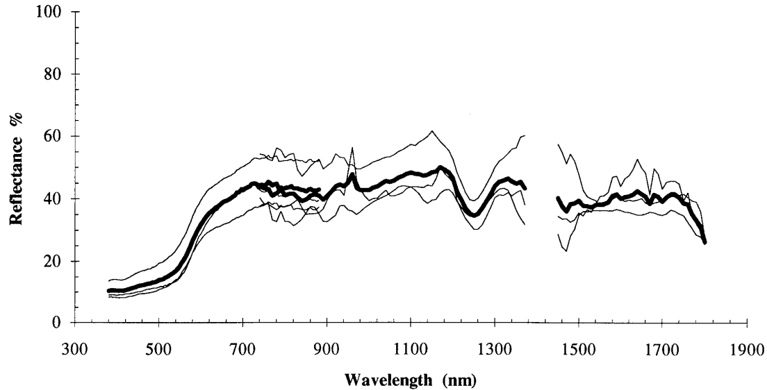
Figure 4.3 Measured reflectances of soils in the Derby area, WA, wet season, March 1983. The heavy line indicates the average reflectance.
