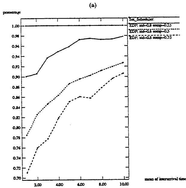
Figure 12: Percentage of accepted tasks (a) EDF (b) LLF compared with Set-Scheduler
