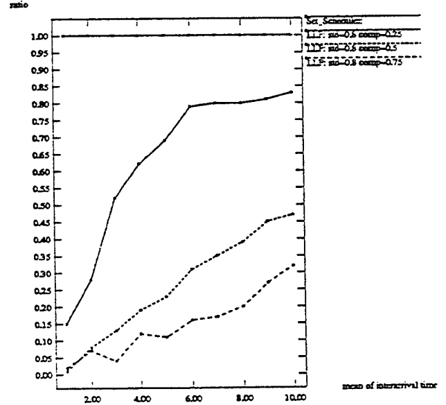
Figure 12: Percentage of accepted tasks (a) EDF (b) LLF compared with Set-Scheduler
