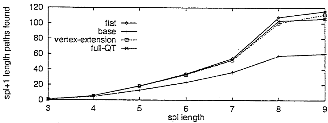
Figure 10: Number of spl + 1 length paths found for Internetwork 3.
