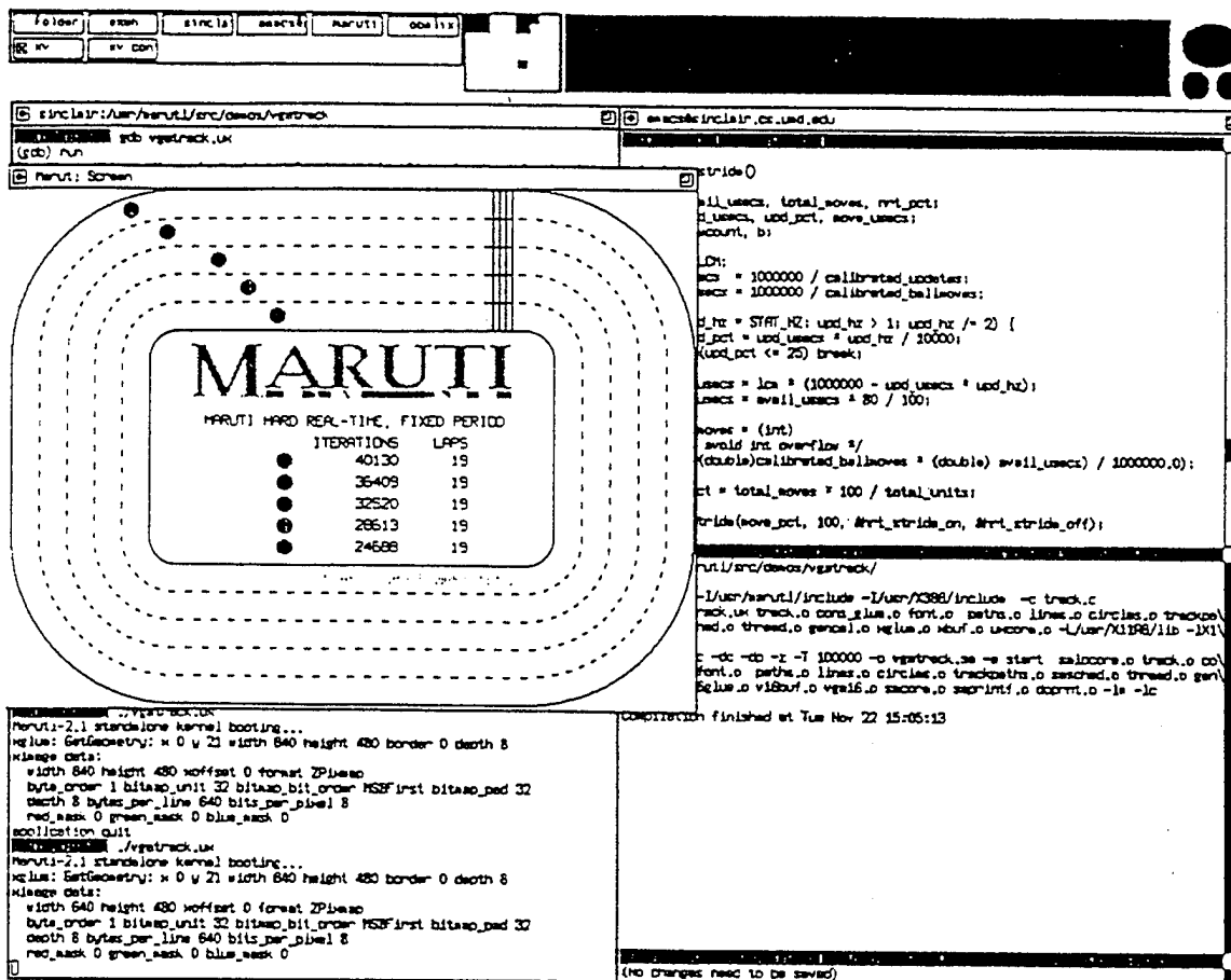
Figure 3: Maruti/Virtual screen running in the development environment
