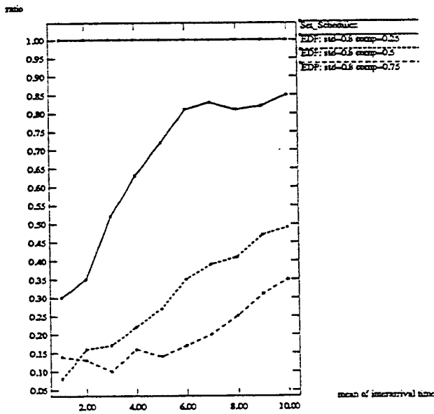
Figure 12: Percentage of accepted tasks (a) EDF (b) LLF compared with Set-Scheduler
