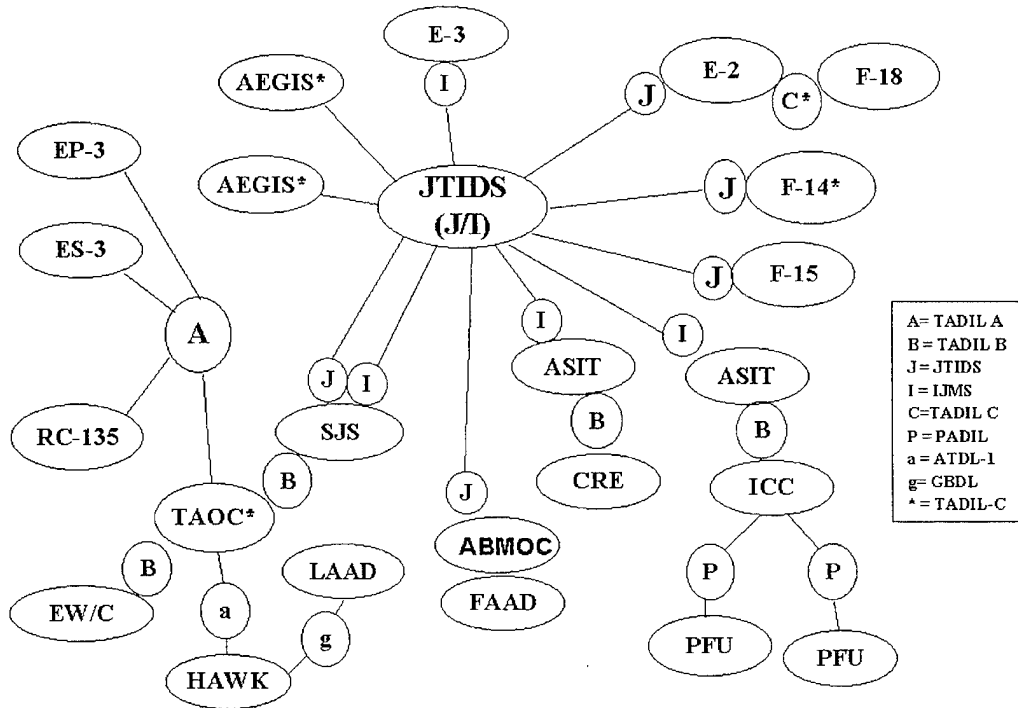
Figure 15. ASCIET95 Communications Architecture [From Ref. 17]
