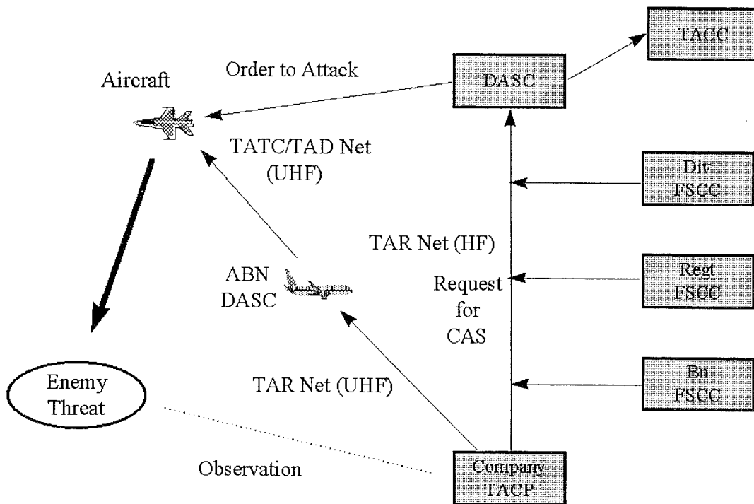
Figure 22. Information Flow for Close Air Support Requests
