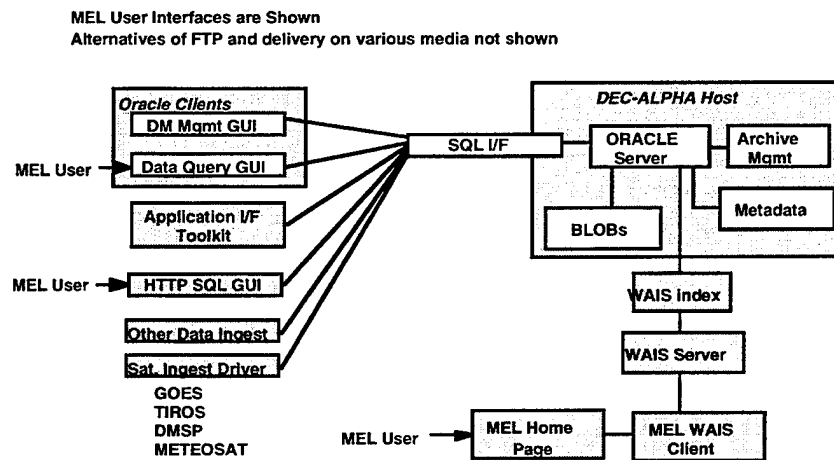
Figure 10. GEQS Architecture
