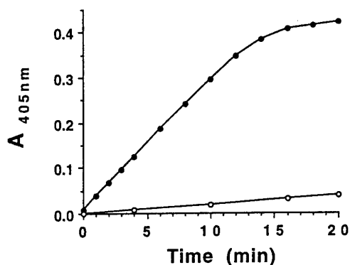
Figure 15. Hydrolysis of p-nitrophenyl ester 1p (0.3 mM; pH 8.3) in the presence of antibody D2.4 (1 \mu M, ●) and, inhibition of catalytic activity in the presence of PNB-phosphonate 4b' ( 4b -N-benzyl amide, 2.5 \mu M, ○)
