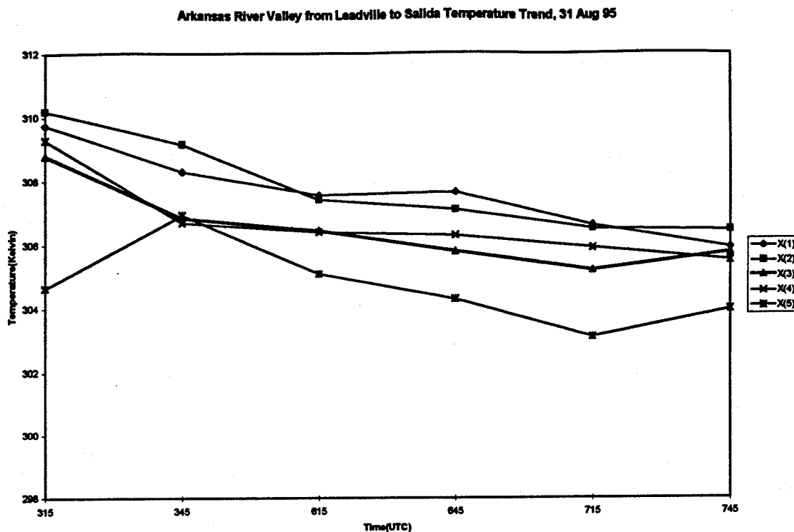
Figure 6.12 Temperature trends from 0315 UTC thru 0745 UTC for the Leadville to Salida valley segment.
