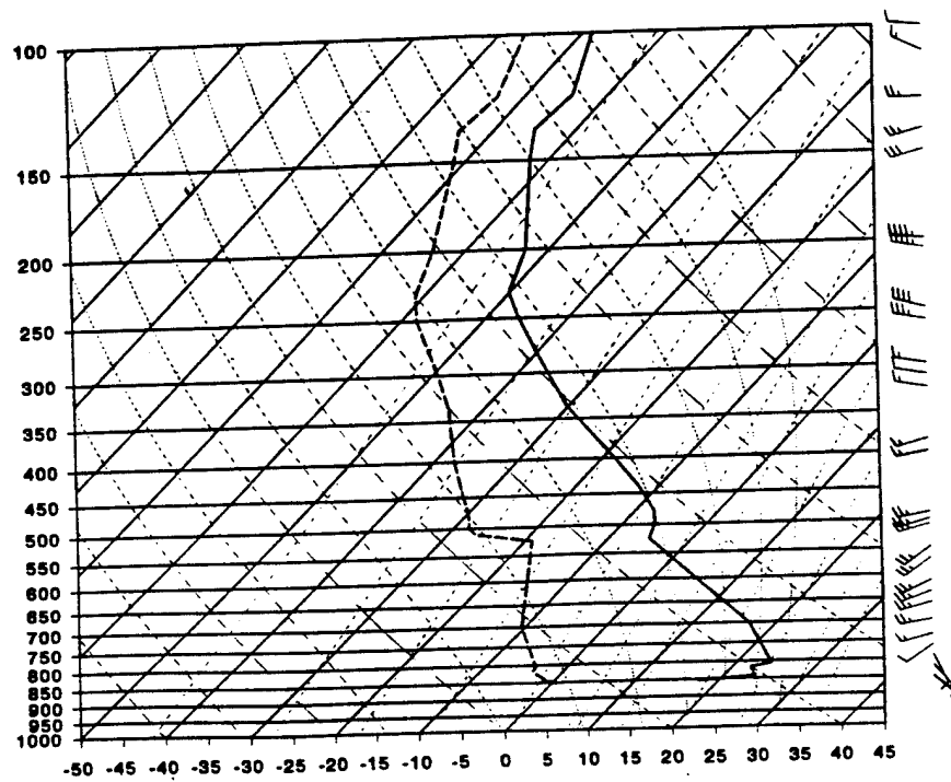
Figure 3.4 26 July 1995 Grand Junction, CO 1200 UTC sounding. The solid and dashed lines represent the temperature and dewpoint profiles, respectively.
