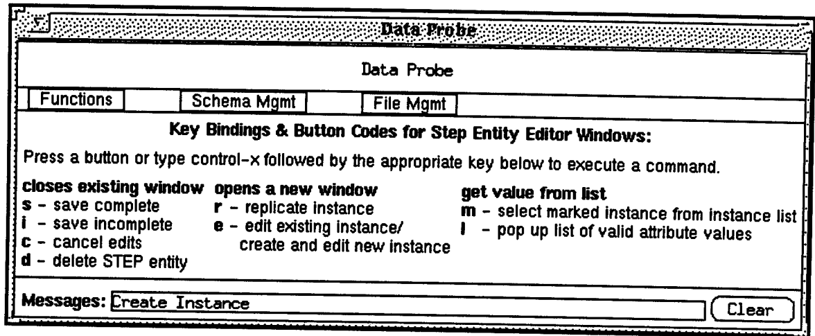
Data Probe Management Window
