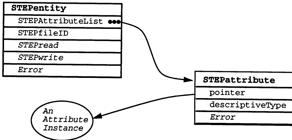
STEP Class Library - major classes and relationships
