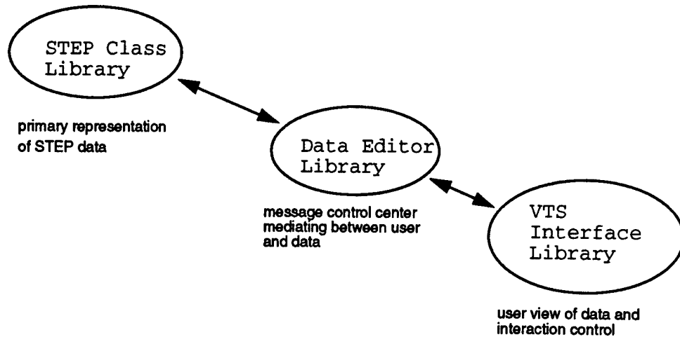
FIGURE 6 Data Editor Library as Mediator
