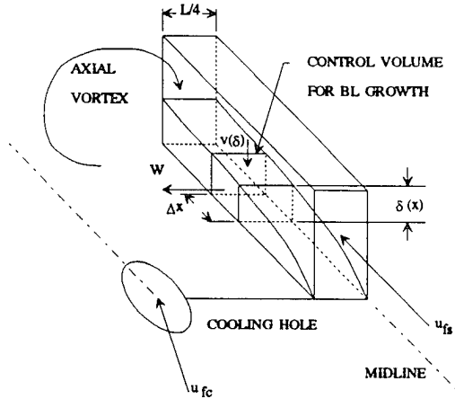
Figure 2. Control Volume for Boundary Layer Growth Near Midline
