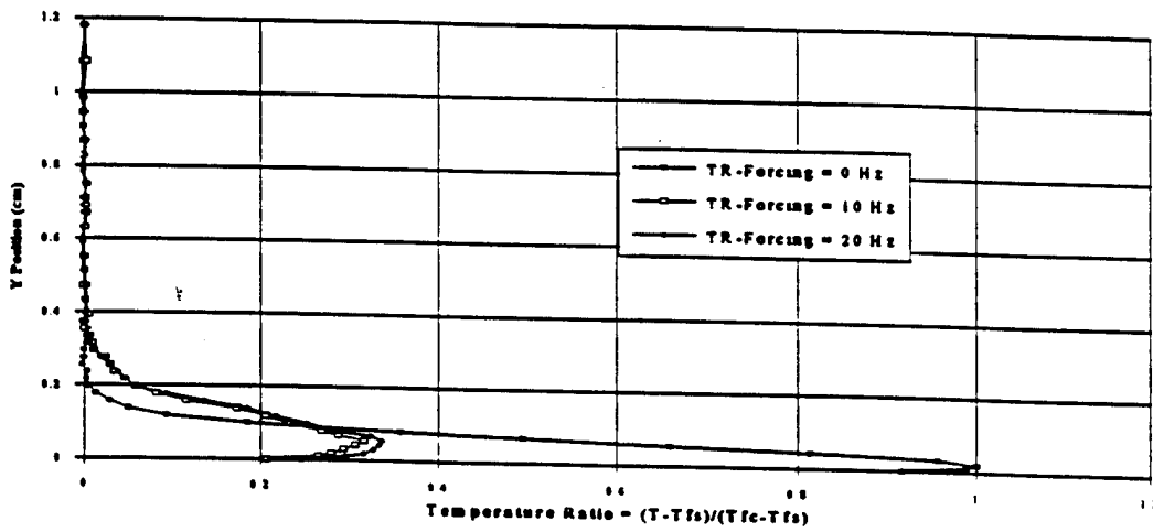
Figure 5a. Temperature Ratio Profiles at x/d = 0 , Tu = 0.7\% , and M = 0.7
